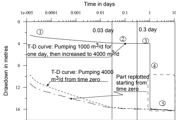
Figure 2. Time-drawdown curves
