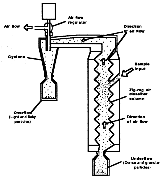
Zig-zag air classifier
