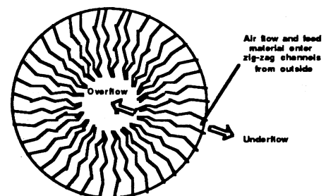
Centrifugal air classifier classifying wheel
