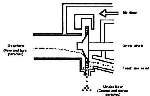
Centrifugal air classifier
