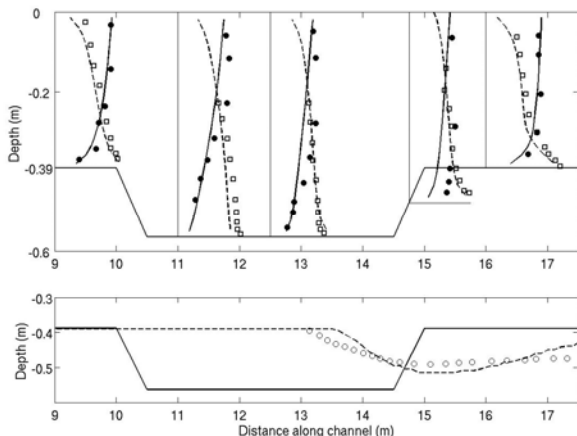
Model (lines) and data (symbols) comparison for "initial" flow velocity and suspended sediment concentration (top panel), and for the trench migration (bottom panel).
