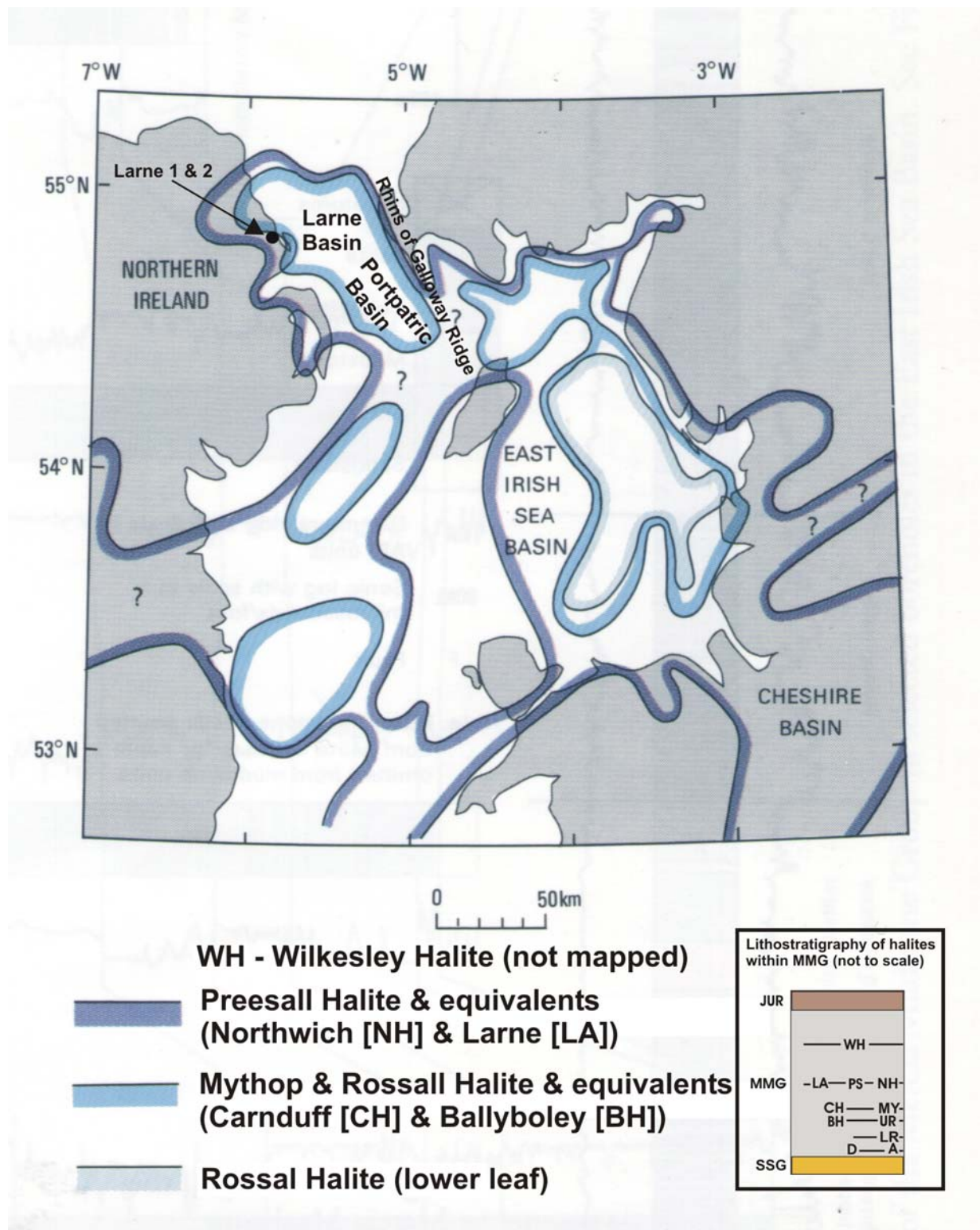
Figure 47 Approximate depositional limits of individual halites within the Mercia Mudstone Group (based upon Jackson et al., 1995).
