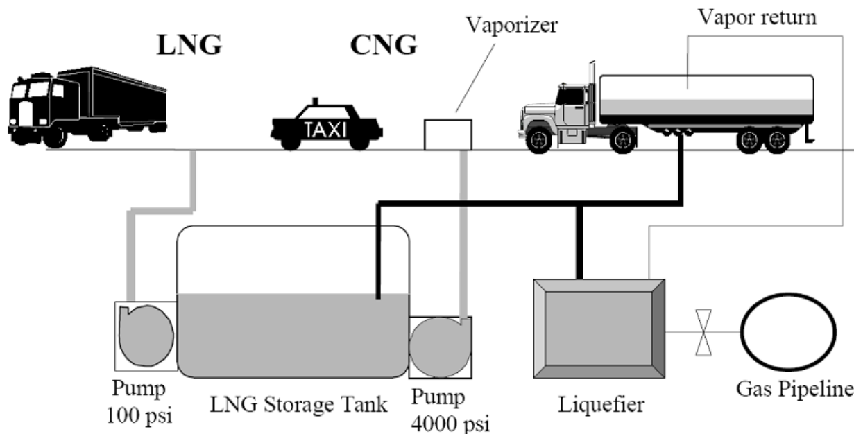
Figure 6. Schematic of liquefied and compressed natural gas facility (after Wegrzyn and Litzke, 1999).
