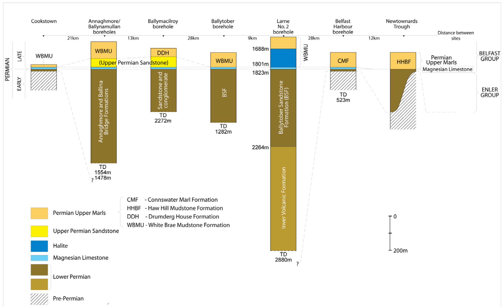
Figure 28 Correlation of Permian rocks from outcrops and boreholes in Northern Ireland (after Mitchell, 2004)
