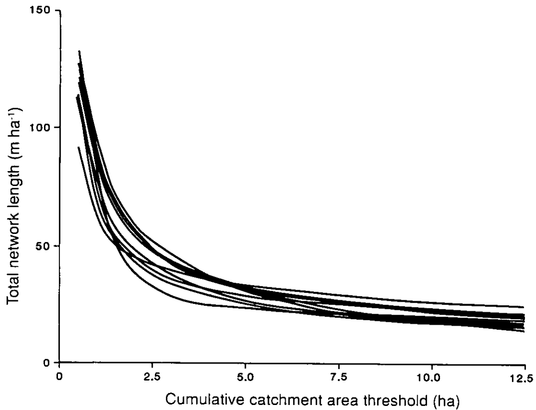
Figure 4.2 Variation in stream length with changes in contributing area threshold
