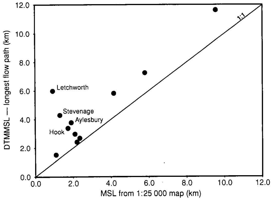
Figure 4.4 Comparison of main stream lengths
