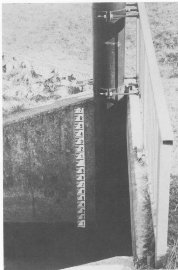
Plate 2.3 Bridge rails used to secure top of stilling well, Stevenage
