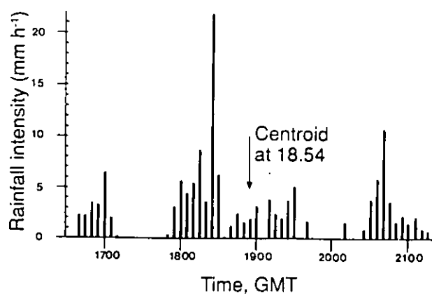
Figure 3.1 Instantaneous uncalibrated five-minute interval catchment average rainfall for the event at Wingrave on 20th December 1989
