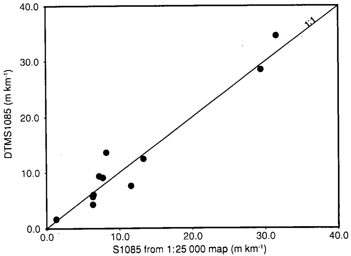
Figure 4.5 Comparison of main channel slopes
