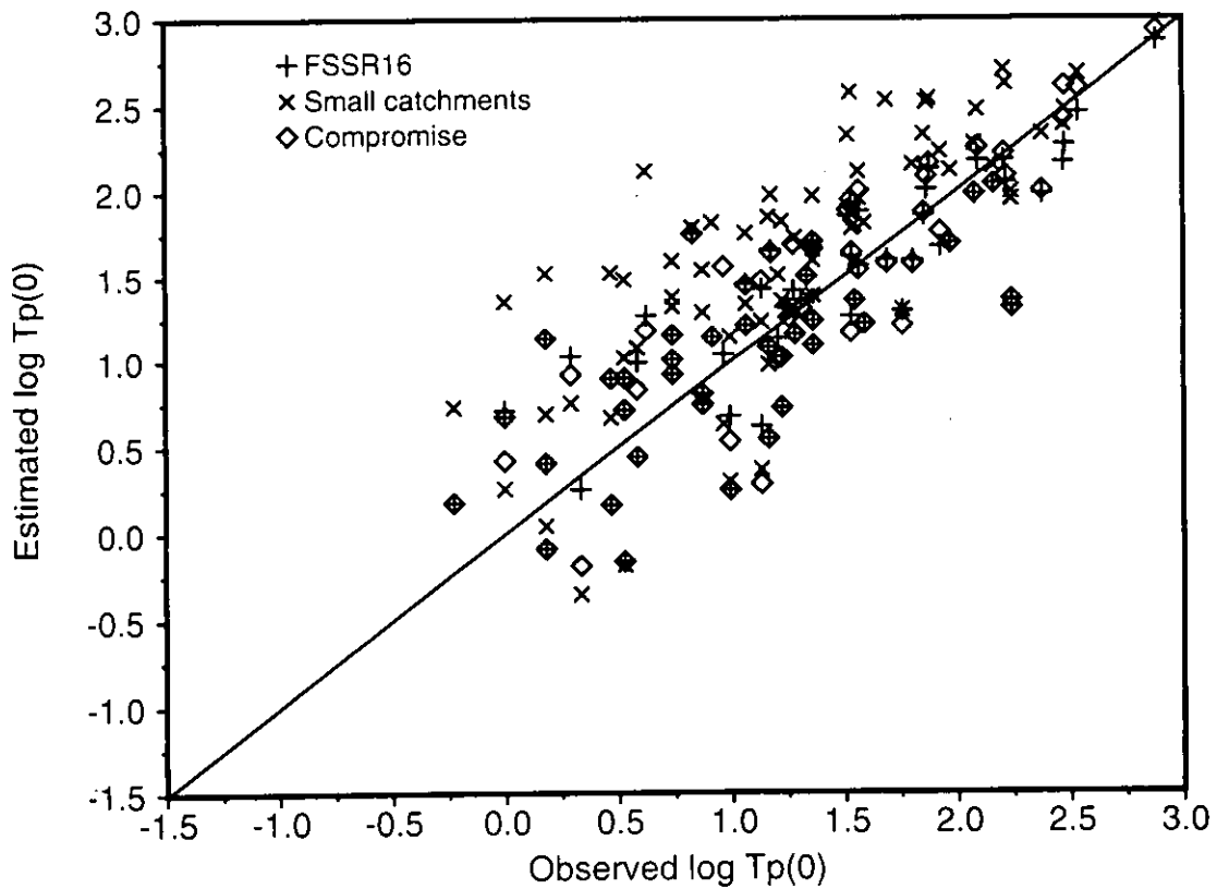
Figure 6.4 Comparison between observed and estimated T_p(0) data for 75 small and/or urban catchments used in FSSR 16 analysis
