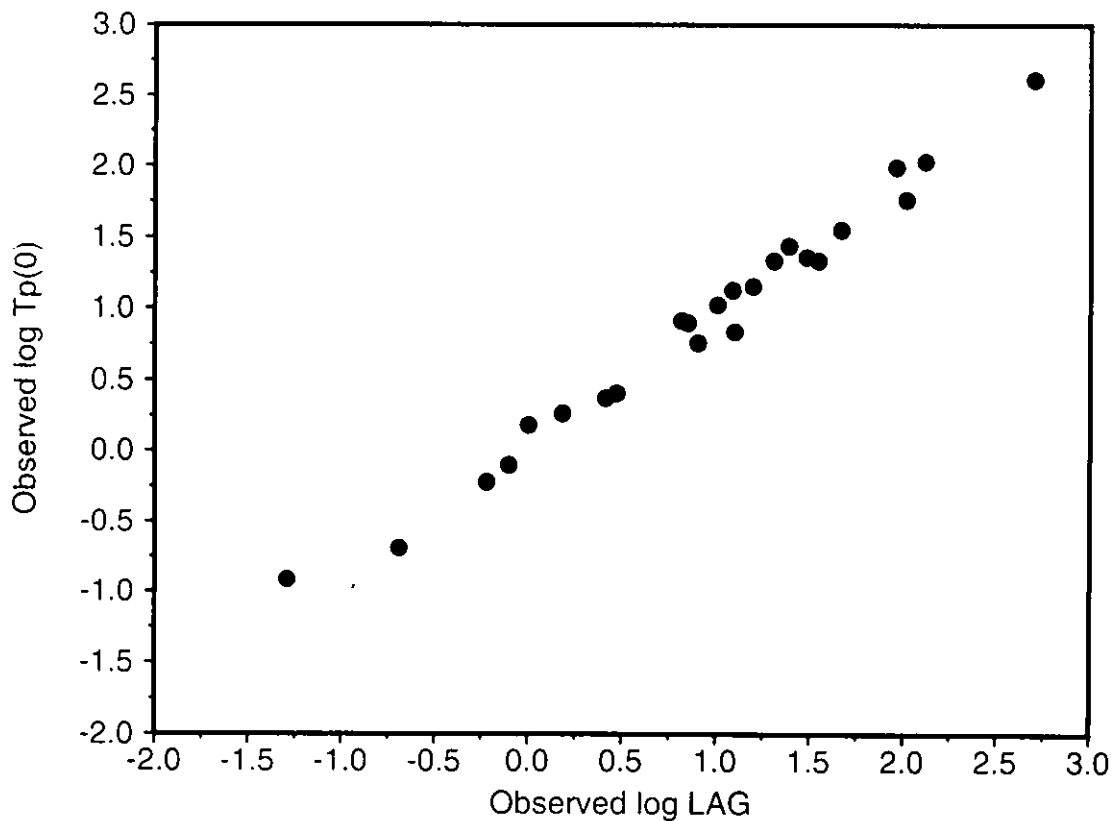
Figure 6.1 Relationship between catchment LAG and T_p(0) geometric means
