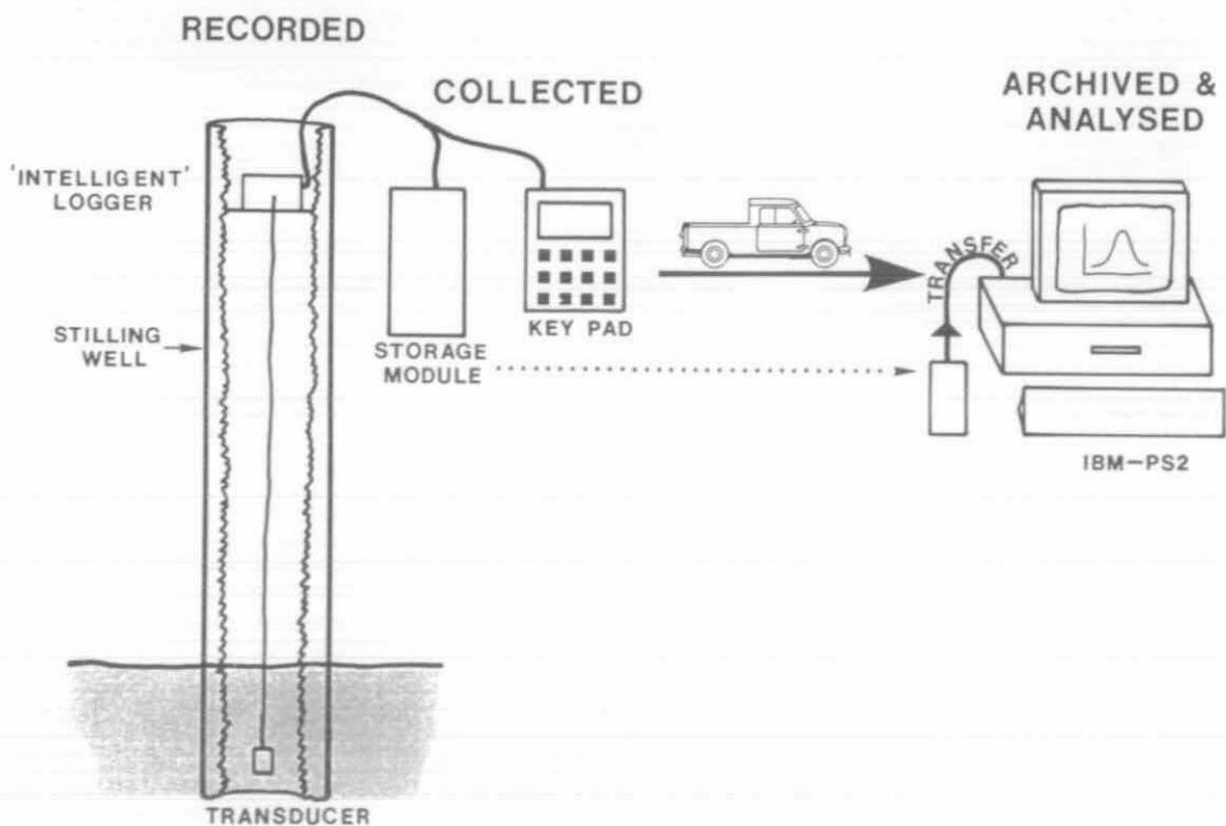
Figure 2.4 Diagrammatic representation of water level data collation
