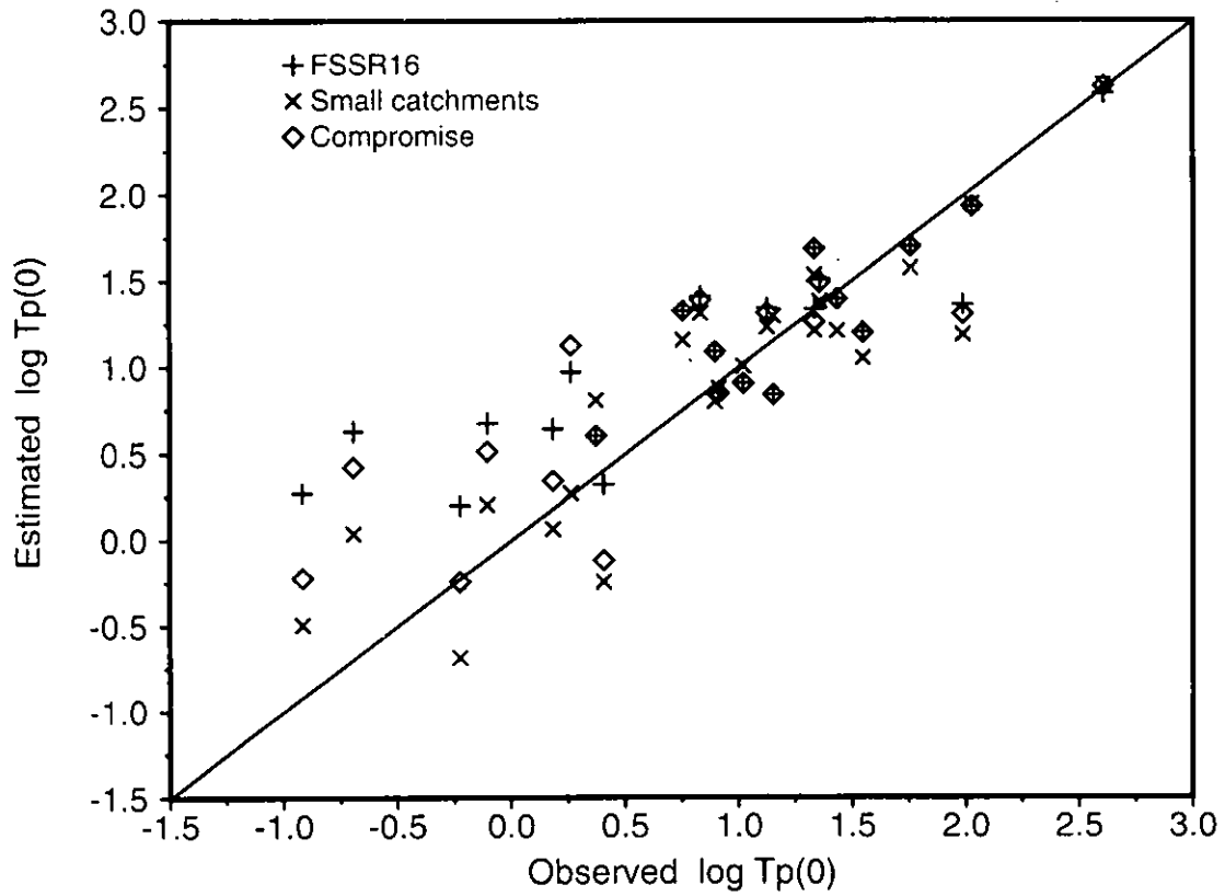
Figure 6.3 Comparison between observed and estimated T_p(0) data for a 24 catchment dataset
