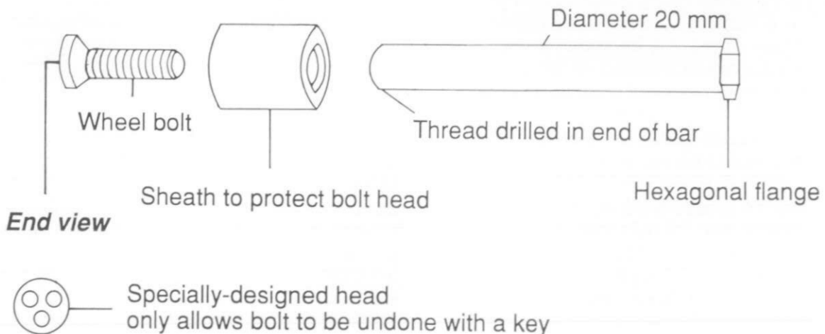
Figure 2.3 Locking bar with special wheel bolt to reduce vandalism
