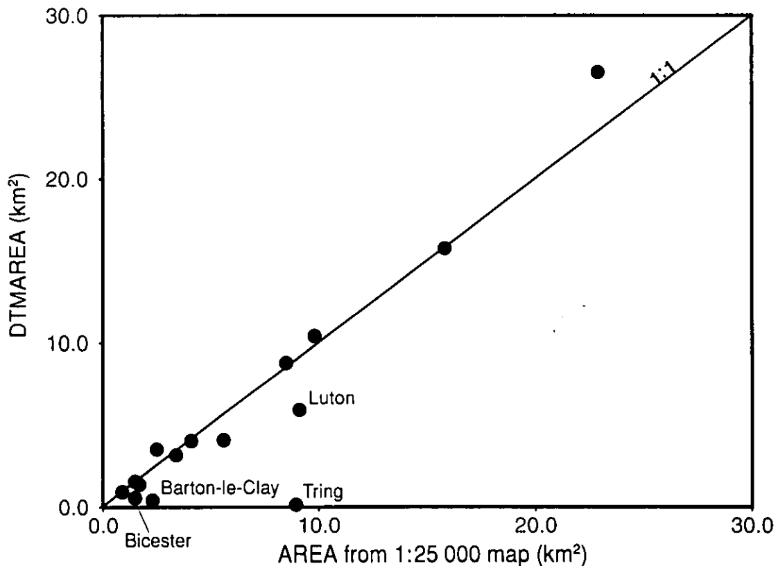
Figure 4.1 Comparison of drainage areas
