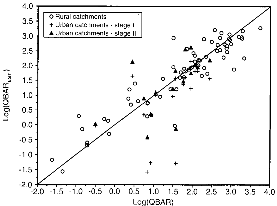
Figure 7.1 Comparison between estimated ( QBAR_{rural} and QBAR_{urban} ) and observed QBAR data for rural and partially urbanised catchments
