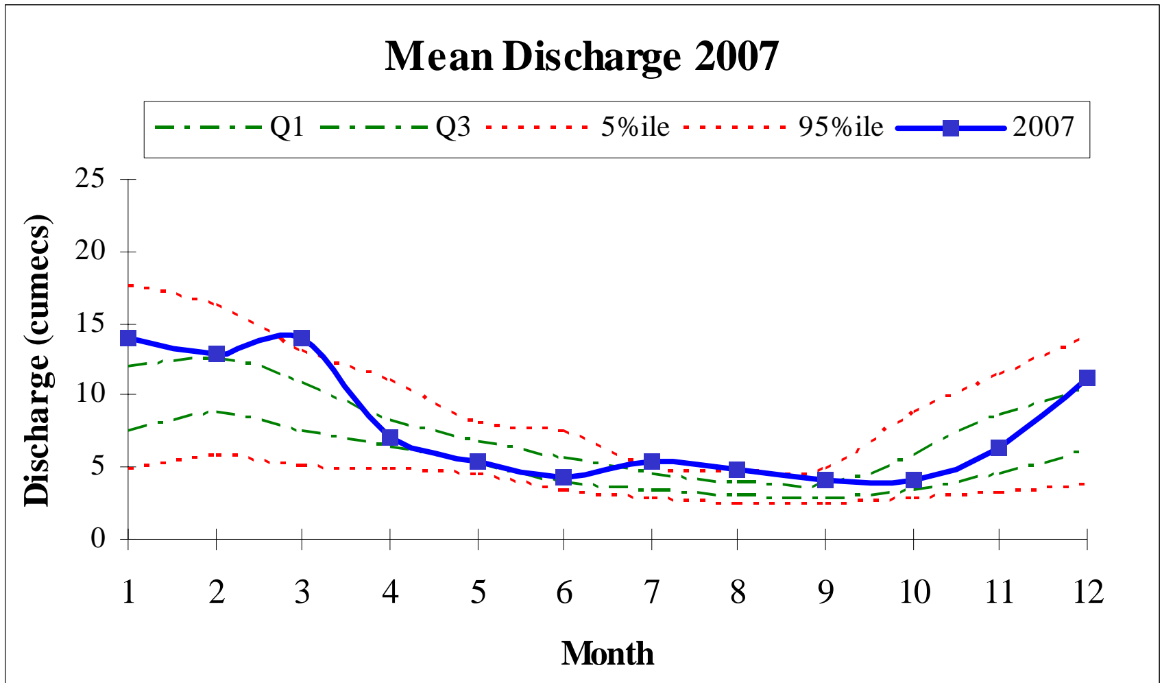
Figure 11: Monthly mean discharge and long-term percentile data (Jan – Dec data)
