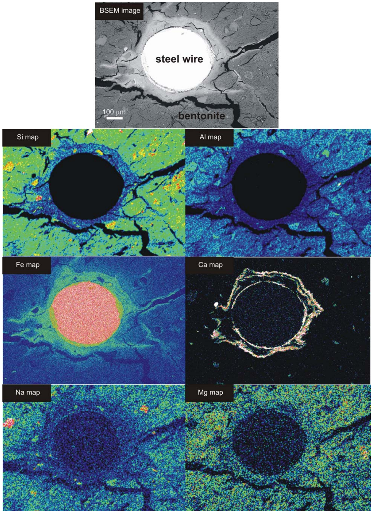
Figure 10. EDXA elemental maps showing the distribution of Si, Al, Fe, Ca, Na and Mg around corroded steel wire within the field of view shown by the BSEM photo in Figure 7. Elements maps are thresholded and rainbow colour contoured to show high concentration as red to white colours and low concentration as black to blue colours. Experiment NFC12, subsample 12c.
