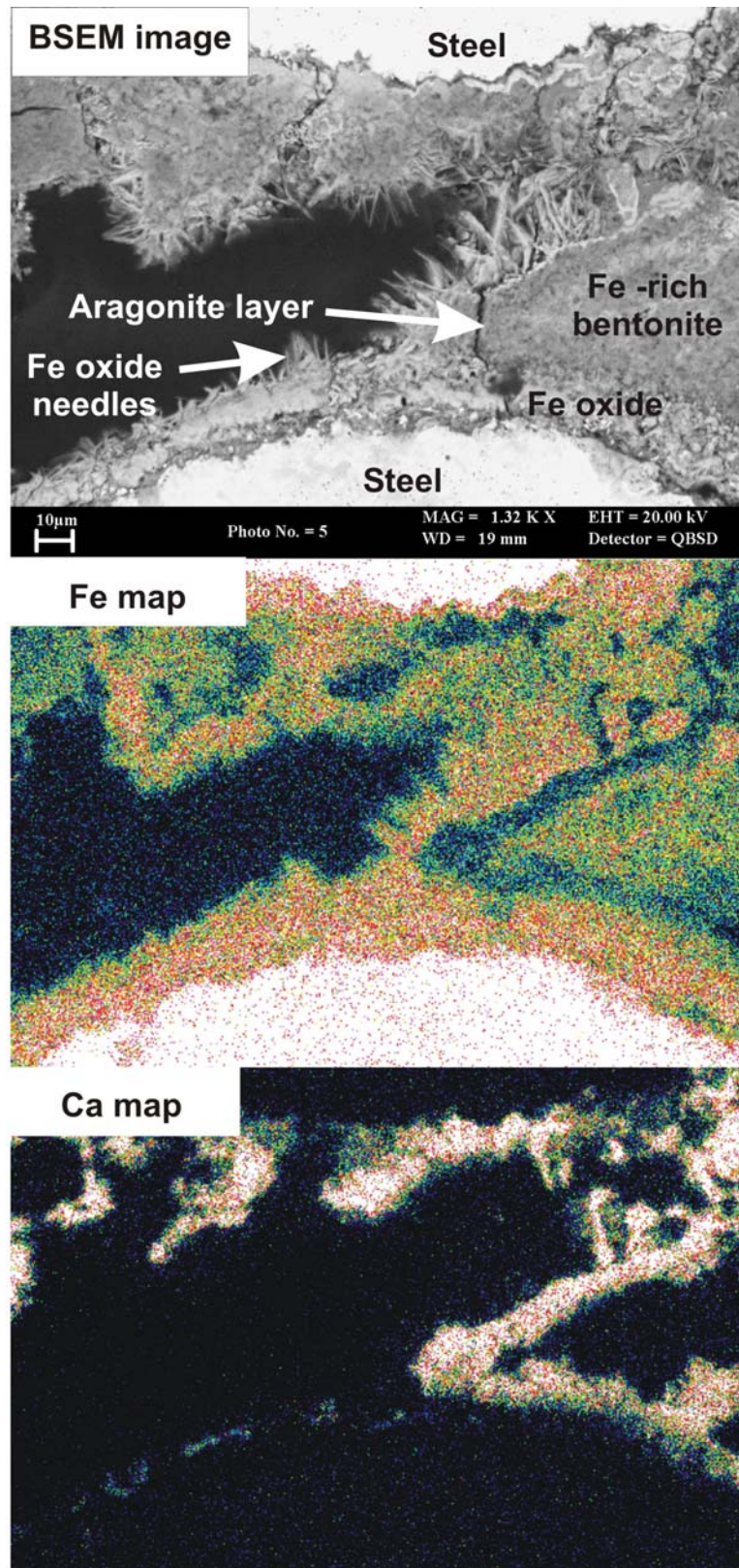
Figure 23. High magnification EDXA elemental maps showing the detailed distribution of Fe and Ca around a corroded steel wire and along open microfractures in the interstitial bentonite matrix. The maps show that a Ca-rich reaction product corresponding to a layer of aragonite on top of Fe-enriched bentonite, and coated by needles of iron oxide or oxyhydroxide lining microcavities in the bentonite adjacent to corroding steel wire. Element maps are thresholded and rainbow colour contoured to show high concentration as red to white colours and low concentration as blue colours. Experiment NFC17, subsample 17a.
