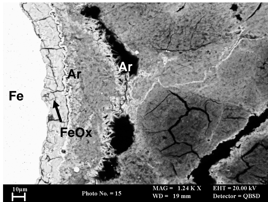
Figure 12. BSEM photomicrograph showing aragonite needles (Ar) lining open shrinkage fractures within the alteration halo in bentonite around a corroded steel wire. The surface of the steel (Fe) is corroded and coated in gel-like iron oxide (FeOx). Clay matrix enriched in Fe appears brighter than unaltered smectitic clay Experiment NFC12, subsample 12c.
