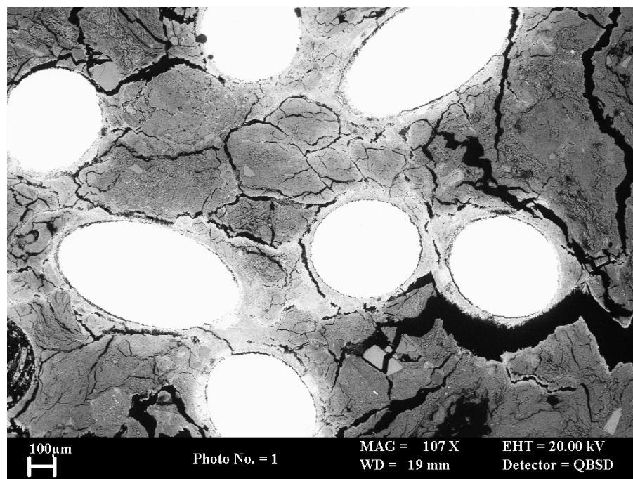
Figure 21. BSEM photomicrograph showing extensive alteration halos around corroded steel wires (white) in bentonite matrix. The altered clay matrix appears brighter than the background unaltered clay due to enrichment with Fe from the corroded metal. Boundaries of the original bentonite clasts are discernible as a result of Fe-enrichment of the clay matrix adjacent to the clast surfaces. Experiment NFC17, subsample 17a.
