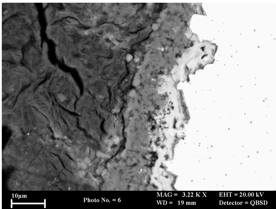
Figure 17. BSEM photomicrograph showing detail of the thin alteration halo around a corroded steel wire. The steel wire (white) is pitted and coated with a thin layer of iron oxide corrosion product (bright). A thin coating of aragonite (mid grey) rests on the iron oxide at the interface with the bentonite (dark grey). Wispy brighter areas within the bentonite matrix are enhanced with Fe along microfractures. Experiment NFC16, subsample 16a.
