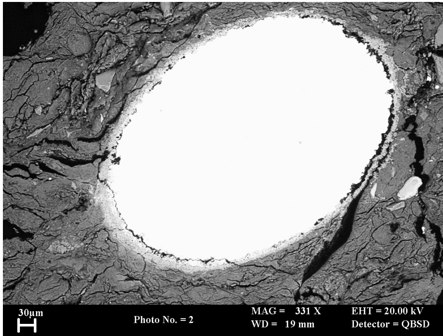
Figure 16 BSEM photomicrograph showing reacted steel wire surrounded by a thin alteration halo comprising iron oxide, aragonite and Fe-enriched altered bentonite. Experiment NFC16, subsample 16a.
