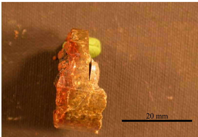
Figure 3. Photograph of subsample 12b. The left hand edge of the sample contains embedded steel wires at the interface between the steel wire-bentonite zone and bentonite without steel wires. The reddish brown staining permeates for up to 5 mm from this interface into the adjacent bentonite. Experiment NFC12.
