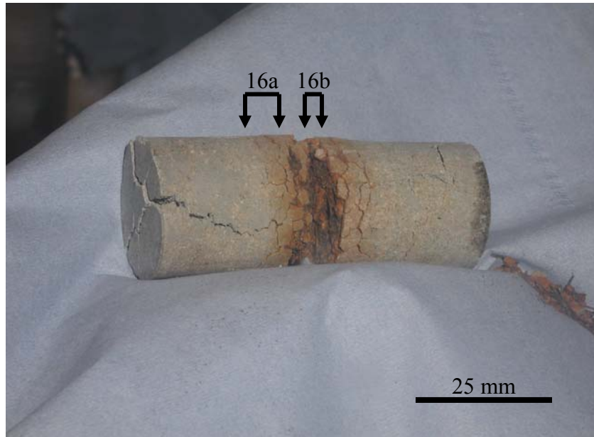
Figure 13. Composite cylinder of compacted bentonite with steel wires and iron coupons recovered from Experiment NFC16 (photographed in nitrogen filled glove box). The central region containing the corroded steel wires is strongly stained by reddish brown iron oxide alteration, with staining along a network of fine fractures. Relatively fresh or unaltered grey-green bentonite remains at the end of the cylinder. The locations of subsamples taken for analysis are shown. [Photograph provided courtesy of Serco Assurance]
