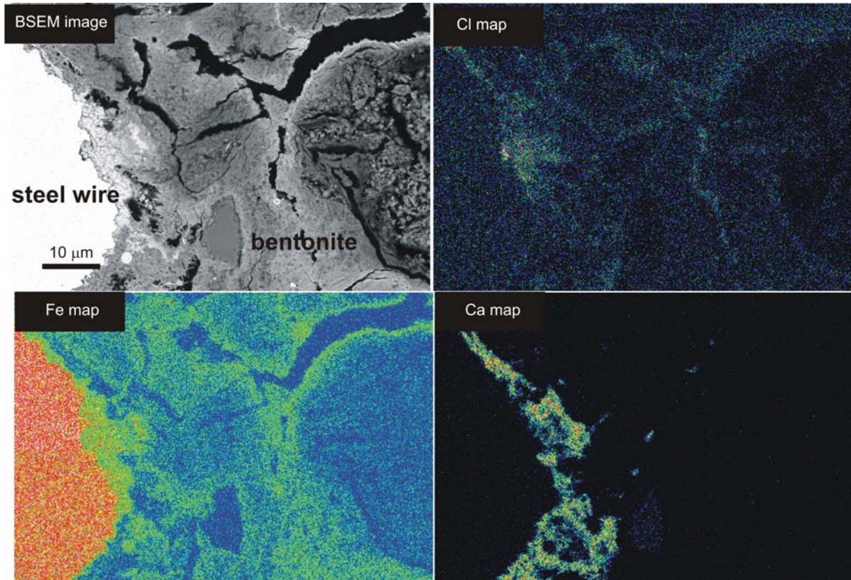
Figure 11. High magnification EDXA elemental maps showing the detail of the distribution of Cl, Fe and Ca close to the surface of a corroded steel wire and along open microfractures in adjacent bentonite. Elements maps are thresholded and rainbow colour contoured to show high concentration as red to white colours and low concentration as black to blue colours. Experiment NFC12, subsample 12c.
