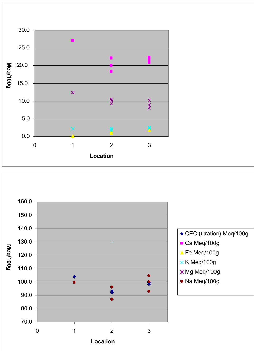
Figure 29. Plots showing the variation in CEC and exchangeable cation chemistry in bentonite, in relation to the location of the subsample within the reacted bentonite cylinders. Location 1 - unreacted background bentonite (subsample 17b); Location 2 – outer margin of the bentonite-steel wire alteration zone; Location 3 – central ‘core’ region of the bentonite-steel wire alteration zone.
