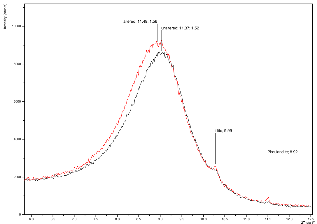
Figure 28. Low angle section of air-dry oriented mount XRD traces to illustrate increase in spacing (Å) and FWHM for the montmorillonite d_{001} peak in altered material (red trace) compared to the ‘unaltered’ material (black trace), Experiment NFC 16, sample 16a.
