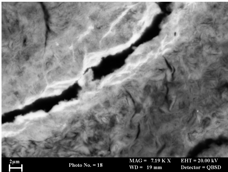
Figure 9. BSEM photomicrograph showing fine detail of secondary iron oxide (bright) lining the wall of a microfracture in bentonite from close to a corroding steel wire. Iron oxide fills second-order microfractures in the walls of the primary fracture. The platy clay particles in the matrix in the bentonite fracture wall appear much brighter than background clay due to their enhancement in Fe but no discrete iron oxide phases could be differentiated in the altered clay matrix. Experiment NFC12, subsample 12c.
