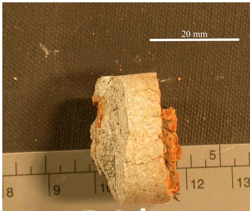
Figure 14. Photograph of subsample 16a showing interface between bentonite and ‘bentonite with steel wire’ region (right), and interface between bentonite and iron coupon (left). Reddish brown staining permeates the matrix of the bentonite between the steel wires but there is only very limited penetration of ‘iron staining’ into the adjacent the wire-free bentonite. Experiment NFC16.
