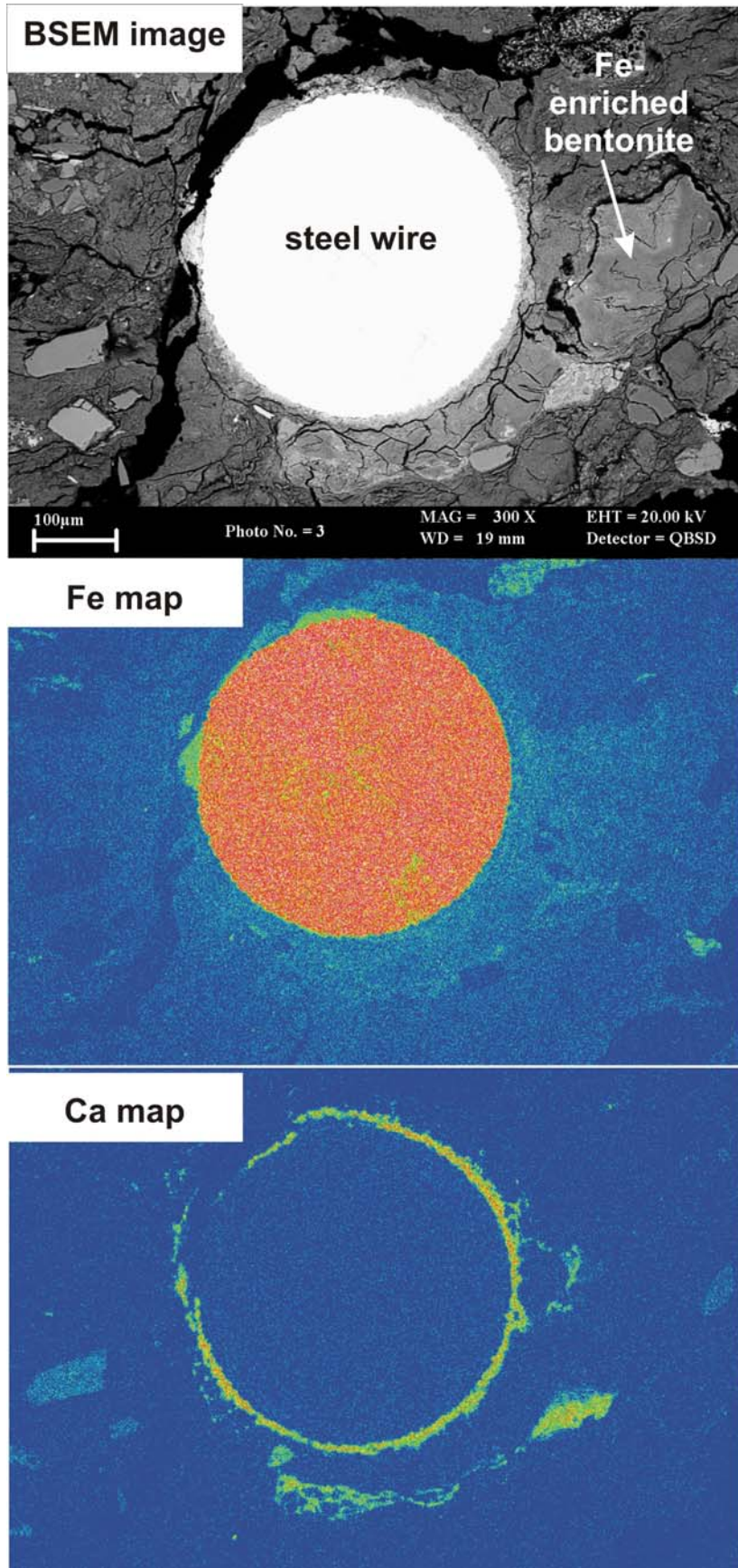
Figure 18. EDXA elemental maps showing the distribution of Fe and Ca around a corroded steel wire and along open microfractures in adjacent bentonite. Elements maps are thresholded and rainbow colour contoured to show high concentration as red to white colours and low concentration as blue colours. Experiment NFC16, subsample 16a.
