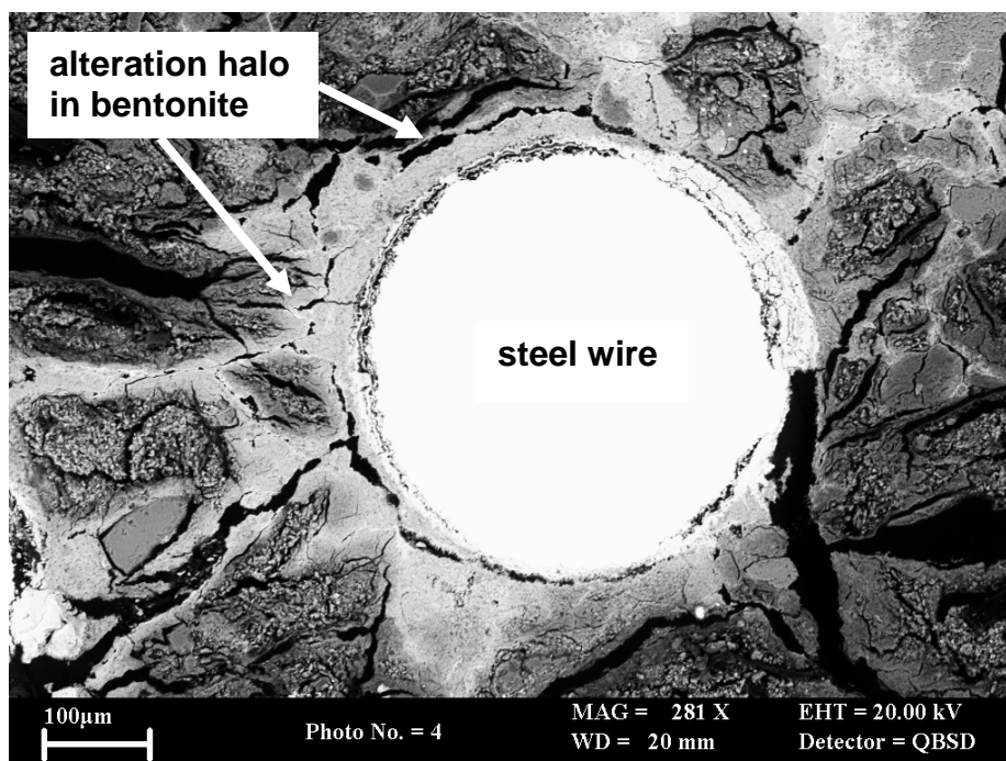
Figure 7. BSEM photomicrograph of a corroded steel wire (white) in bentonite. The bentonite around the wire shows a halo of alteration (light grey) which also penetrates further into the bentonite clay matrix (darker grey) along microfractures radiating away from the wire. Disseminated angular grains of K-feldspar (mid grey) show no evidence of alteration. Experiment NFC12, subsample 12c.
