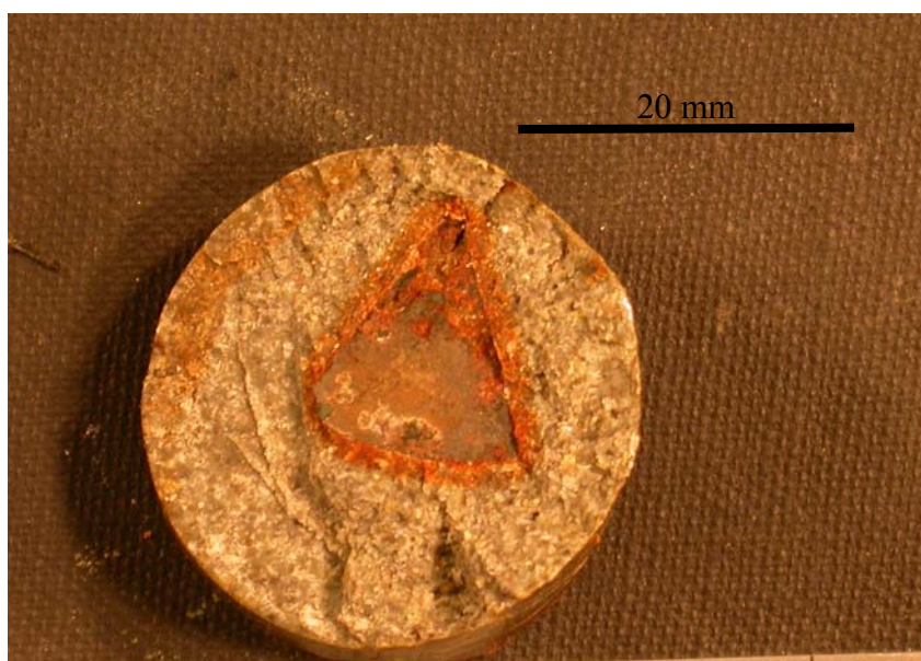
Figure 5. Photograph of subsample 12a sliced through the contact of the iron coupon near the unaltered end of the compacted bentonite cylinder (iron coupon removed), showing the ‘triangular’ mouldic impression of the segment of iron coupon. The coupon surface is coated with a film of reddish-brown iron oxide corrosion product and surrounded by thin halo of reddish-brown iron oxide staining in the immediately adjacent bentonite. Localised weak staining by orange-brown alteration can be seen in the outer margins of the sliced bentonite disc. Experiment NFC12.
