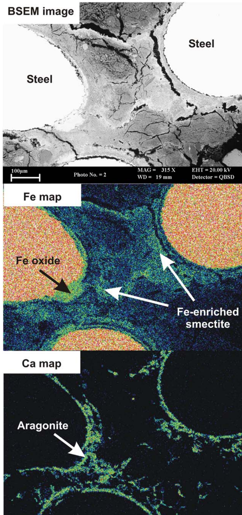
Figure 22. EDXA elemental maps showing the distribution of Fe and Ca around corroded steel wires and along open microfractures in adjacent bentonite matrix. Elements maps are thresholded and rainbow colour contoured to show high concentration as red to white colours and low concentration as black to blue colours. Experiment NFC17, subsample 17a.
