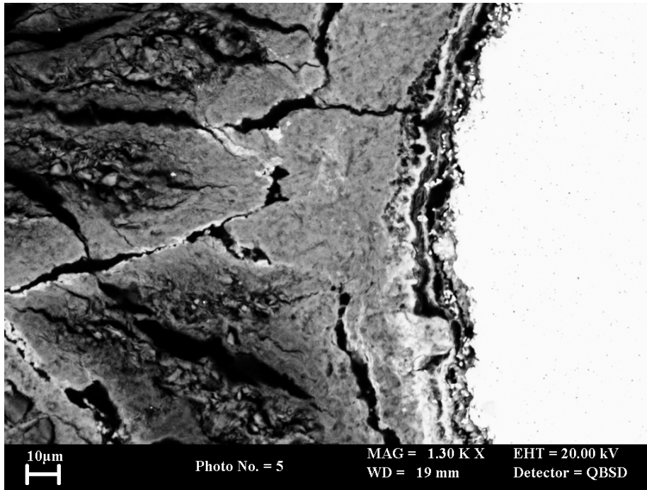
Figure 8. BSEM photomicrograph showing detail of a corroded steel wire. The metal surface is surrounded by concentric bands of microporous iron oxide. Interconnected open microfractures in the clay matrix are lined by a fine layer of iron oxide or iron oxyhydroxide (bright). The fracture walls appear to have enhanced backscattered electron coefficient (i.e. appear brighter than the background clay) due to significant iron enhancement to a depth of up to 20 \mu\text{m} . Experiment NFC12, subsample 12c.
