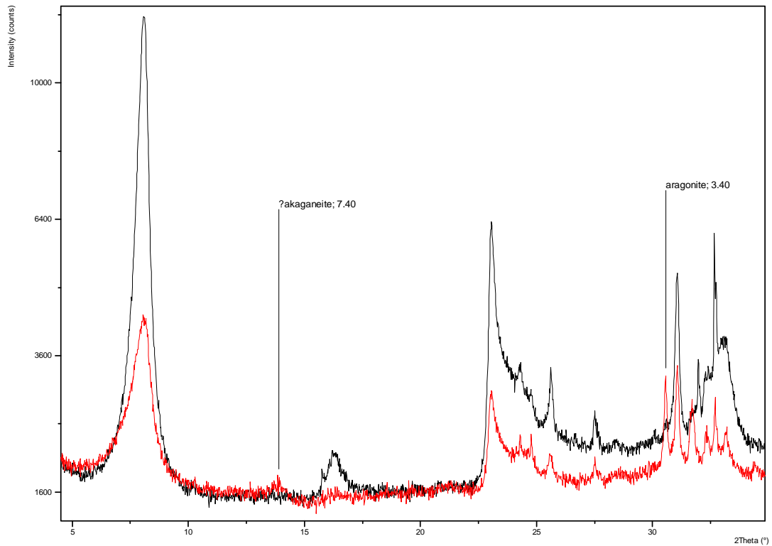
Figure 25. Section of random powder mount XRD traces for altered bentonite material (black trace) and material removed from the surface of the corroding wire (red trace). Diagnostic peak positions for the alteration products for possible akaganeite and aragonite are shown, Experiment NFC 17, sample 17a.
