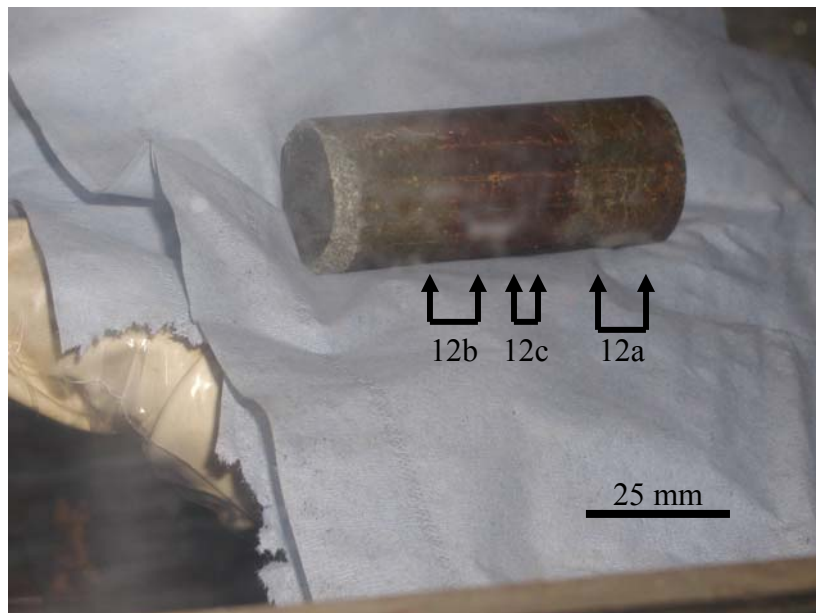
Figure 2. Composite cylinder of compacted bentonite with steel wires and iron coupons recovered after experimentation from Experiment NFC12 (photographed in nitrogen filled glove box). The central region containing the corroded steel wires is strongly stained by reddish brown iron oxide alteration. Relatively fresh or unaltered grey-green bentonite remains at the end of the cylinder. The locations of subsamples taken for analysis are shown. [Photograph provided courtesy of Serco Assurance]
