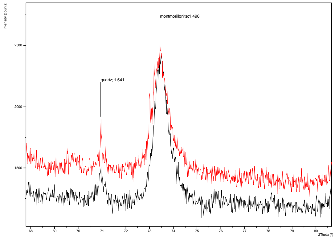
Figure 26. High angle section of random powder mount XRD traces for 'unaltered' material (black trace) and altered material (red trace) to illustrate a lack of change in the montmorillonite d_{060} spacing, Experiment NFC 12, sample 12b.
