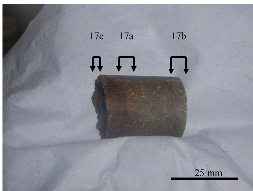
Figure 19. Composite cylinder of compacted bentonite with steel wires and iron coupons recovered after experimentation from Experiment NFC17 (photographed in nitrogen filled glove box). The central region containing the corroded steel wires is strongly stained by reddish brown iron oxide alteration. Relatively fresh or unaltered grey-green bentonite remains at the end of the cylinder. The locations of subsamples taken for analysis are shown. [Photograph provided courtesy of Serco Assurance]
