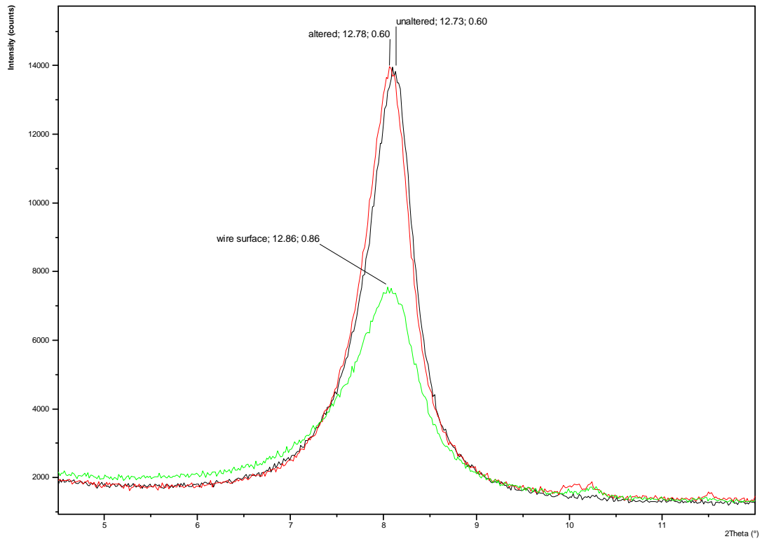
Figure 27. Low angle section of random mount XRD traces to illustrate increase in spacing (Å) and FWHM for the montmorillonite d_{001} peak in altered material (red trace) and wire surface material (green trace) compared to the ‘unaltered’ material (black trace), Experiment NFC 16, sample 16a.
