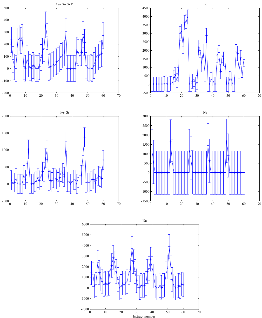
Figure 31. Component profiles for, Ca-Si-S-P, Fe, Fe-Si, Na1, Na2
