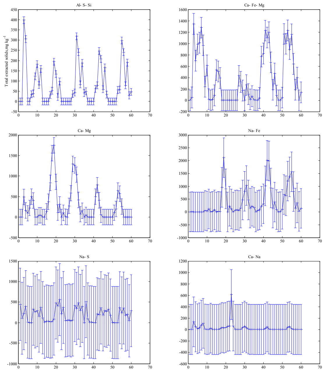
Figure 30. Component profiles for Al-S-Si, Ca-Fe-Mg, Ca-Mg, Na-Fe, Na-S, Ca-Na
