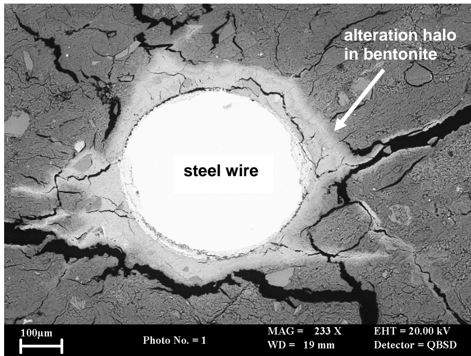
Figure 6. BSEM photomicrograph of a corroded steel wire (white) in bentonite. The bentonite around the wire shows a halo of alteration (light grey) which also penetrates further into the bentonite clay matrix (darker grey) along microfractures. Disseminated angular grains of K-feldspar (mid grey) show no evidence of alteration. Experiment NFC12, subsample 12c.
