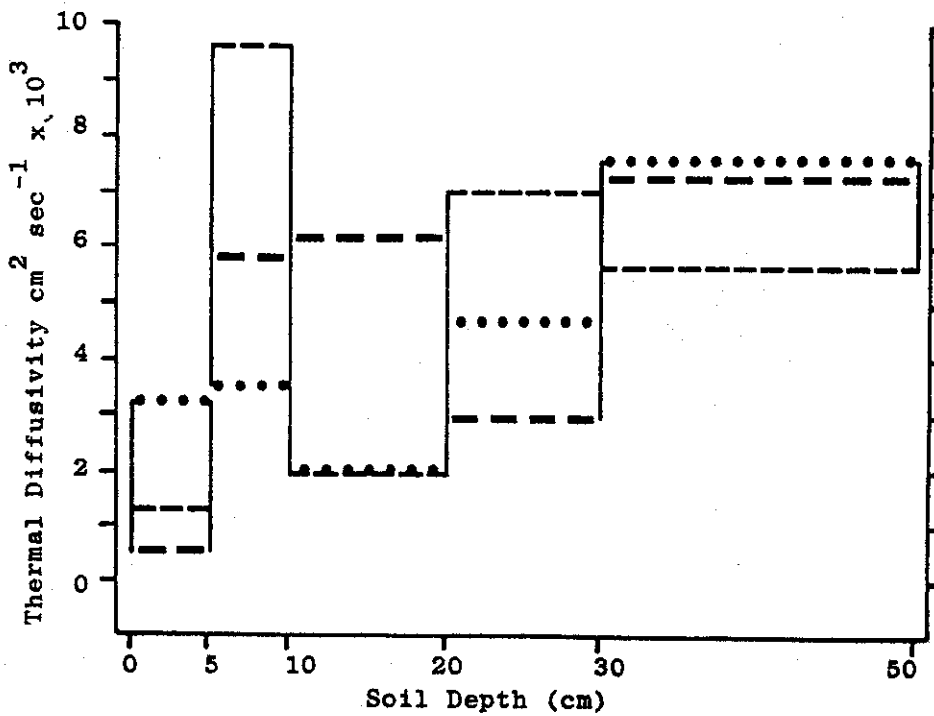
Mean thermal diffusivity calculated from phase angles of the fundamental sine waves for the top and bottom of each soil stratum. ——— 1966-67, ..... 1967-68, ----- 1968-69.
