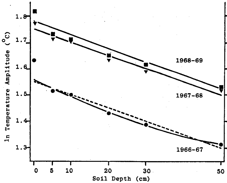
Natural logarithm of the amplitude of the fundamental sine curve of soil temperature for years August - July and soil depth. ——— Line of best fit, ----- linear regression where line of best fit is curvilinear. Comparable data for screen air temperature were 1.52, 1.65 and 1.72
