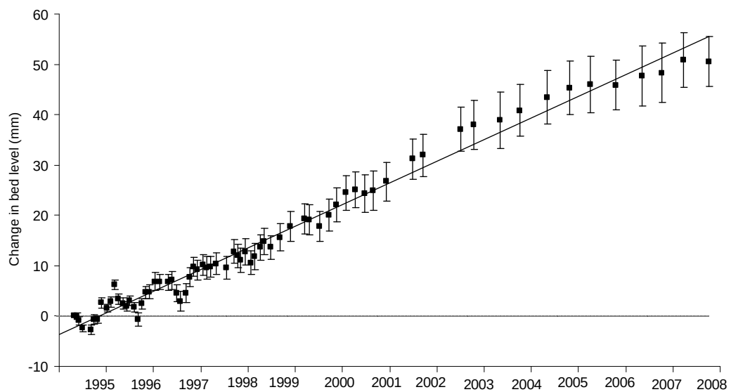
Figure 2.3 Mean sedimentation (n=16) for the Tollesbury salt marshes between April 1994 and October 2007 with best fit line. Mean rate is 4.2\text{mm year}^{-1} (regression equation: y = -7.505 + 0.01162 \text{ day} ; r^2=97.9\% , p<0.001 ).
