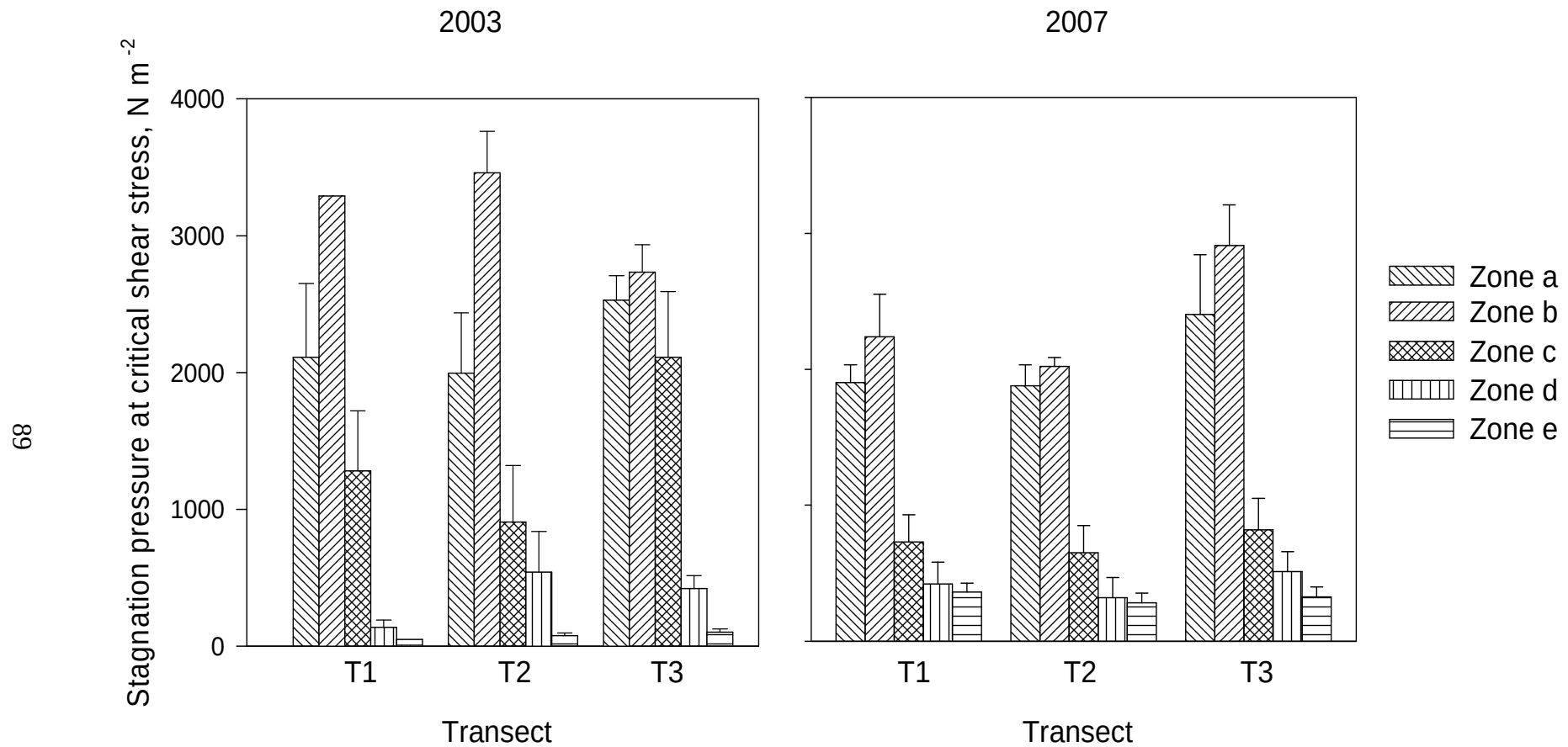
Figure 3.2 Stagnation pressure values at critical shear stress measured using the cohesive strength meter (CSM). Measurements were made in September 2003 and 2007 on three transects. Zones a to e represent different vegetation zones (see Table 3.1).
