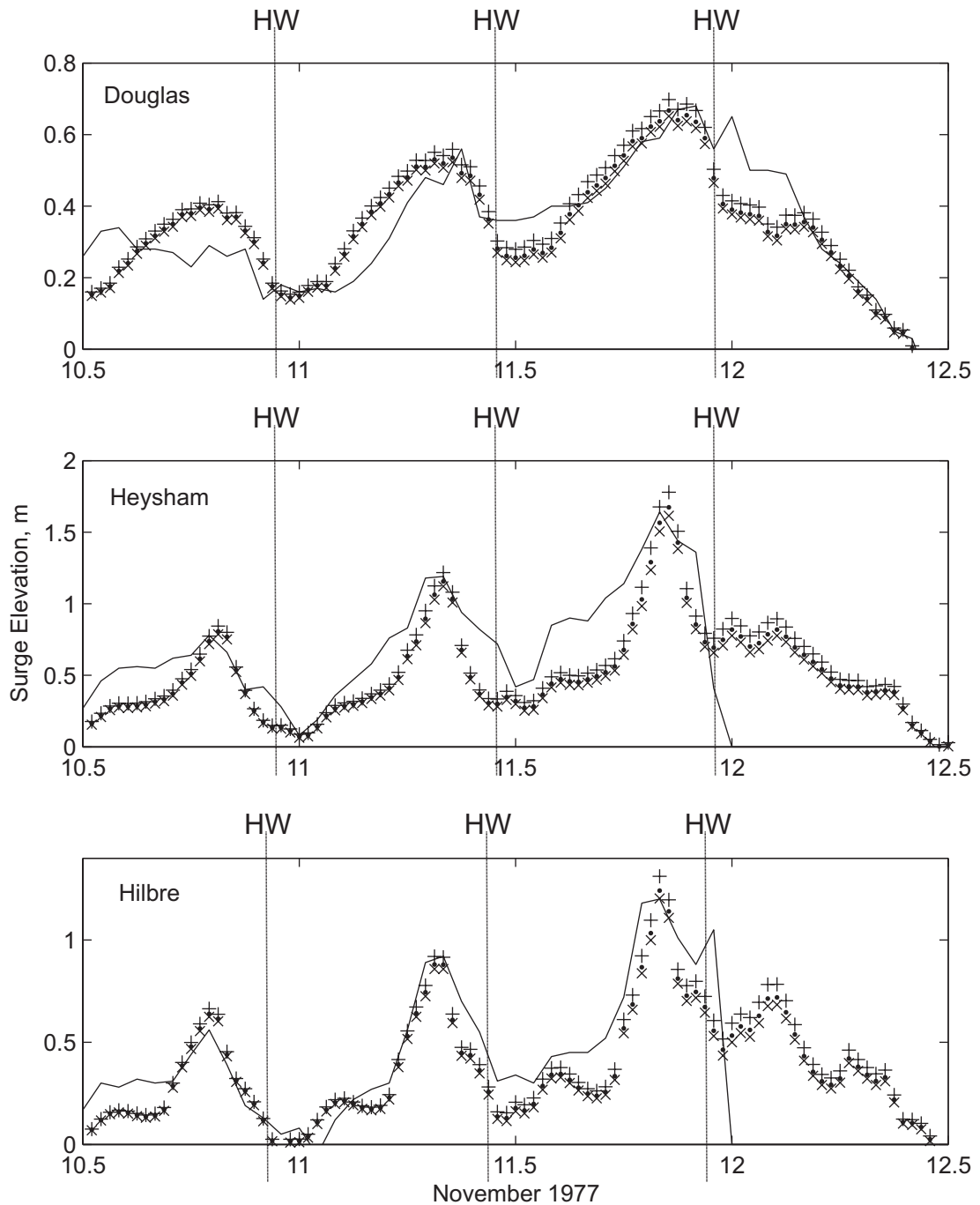
Fig. 4 Surge prediction using Charnock parameters of 0.0275 (+), 0.0185 (•) and 0.0144 (×), using POLCOMS with a minimum depth of 5m, compared to tide gauge data (-). Douglas represents a deep location, while Heysham and Hilbre represent shallow locations along the Sefton coast. The times of high water (HW vertical lines) are after the peaks in surge, which occur on the rising tide. The time resolution is the day in November, e.g. 10 = 00:00 10 th November and 10.5 = 12:00 10 th November
