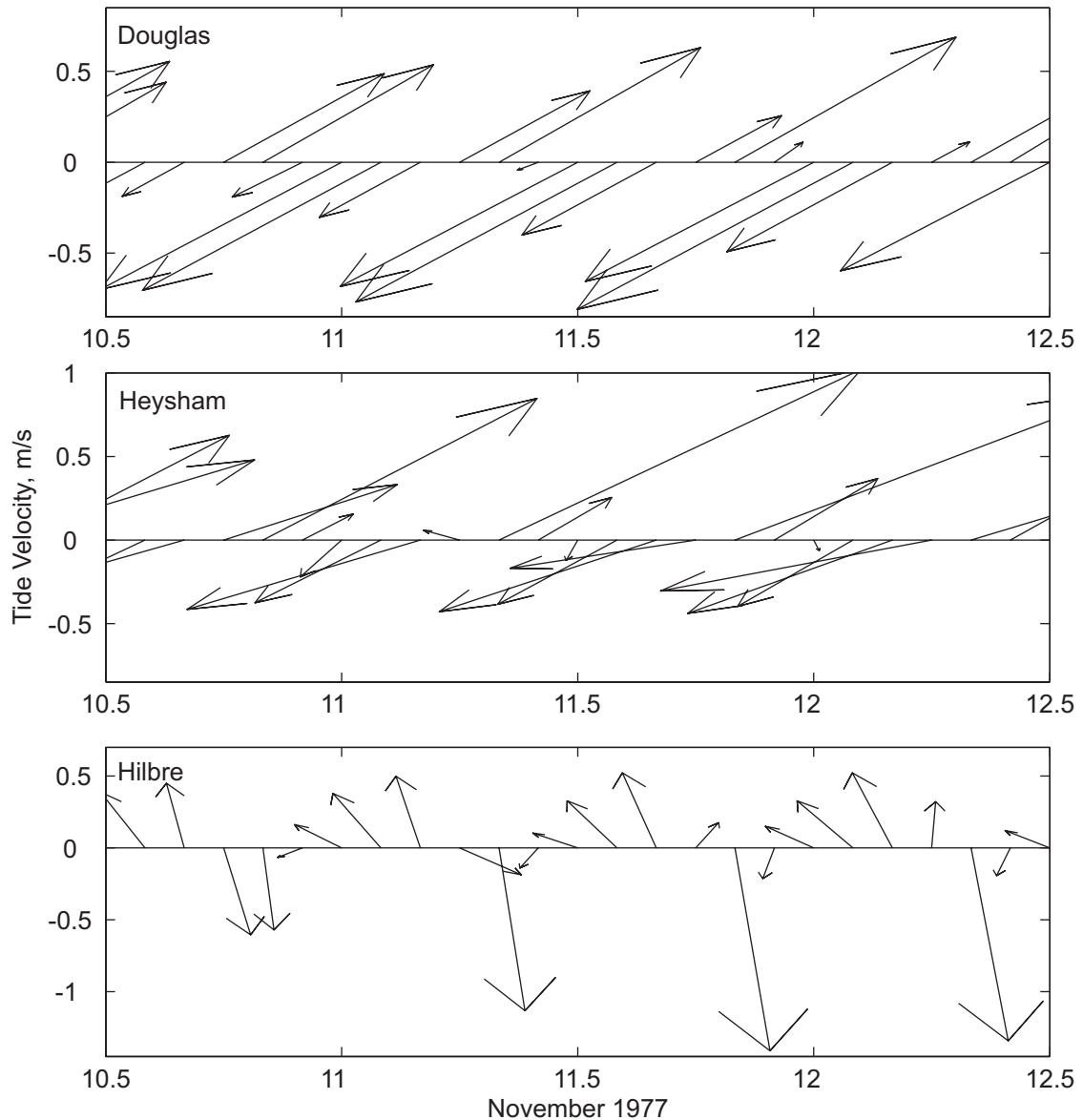
Fig. 6 Tide only depth – averaged current vectors every 2 hours at Douglas, Heysham and Hilbre, located in Fig. 3, during the period 10 th November (12:00) to 12 th November (12:00) 1977. The time resolution is the day in November, e.g. 10 = 00:00 10 th November and 10.5 = 12:00 10 th November
