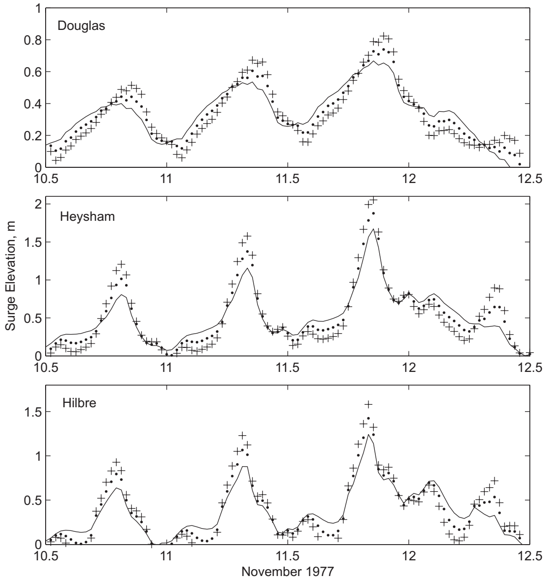
Fig. 7 The surge prediction at Douglas, Heysham and Hilbre for present day conditions (—) and with sea level rises of 0.7m (●) and 1.4m (+). The time resolution is the day in November, e.g. 10 = 00:00 10 th November and 10.5 = 12:00 10 th November
