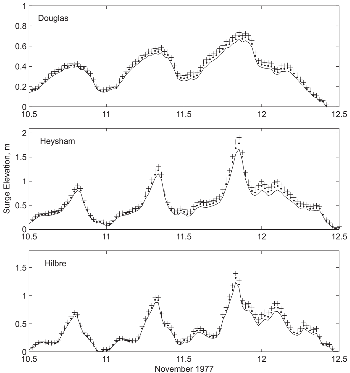
Fig. 8 The surge prediction at Douglas, Heysham and Hilbre for present day conditions (–) and with enhanced wind speeds of 5% (●) and 10% (+). The time resolution is the day in November, e.g. 10 = 00:00 10 th November and 10.5 = 12:00 10 th November
