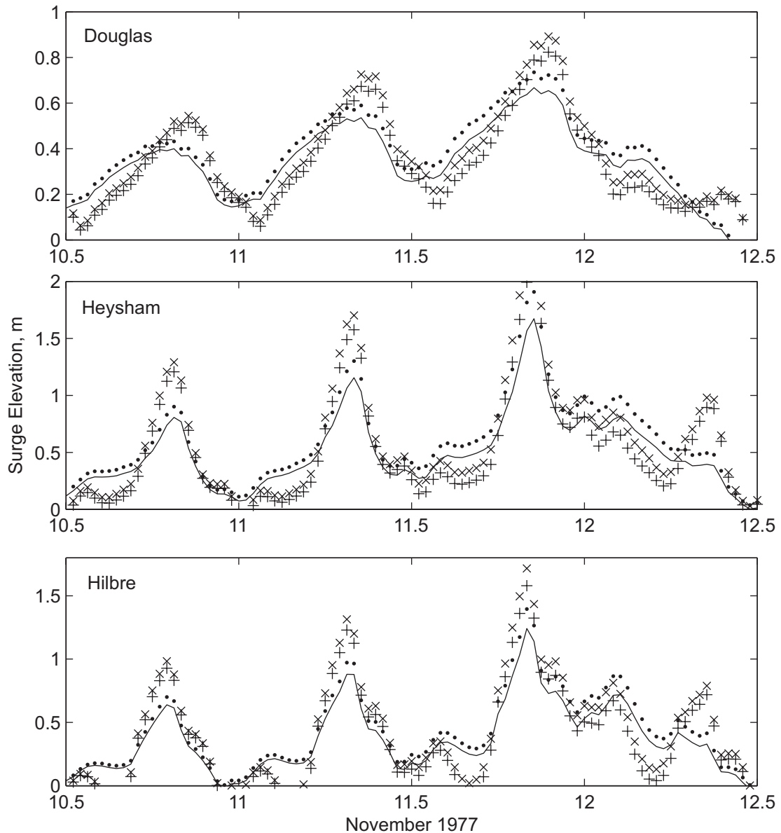
Fig. 9 The surge prediction at Hilbre and Douglas for present day conditions (-), present day conditions with enhanced wind speeds of 10% (•) and 1.4m sea level rise (+), and combined 1.4m sea level rise and 10% wind enhancement (x). The time resolution is the day in November, e.g. 10 = 00:00 10 th November and 10.5 = 12:00 10 th November
