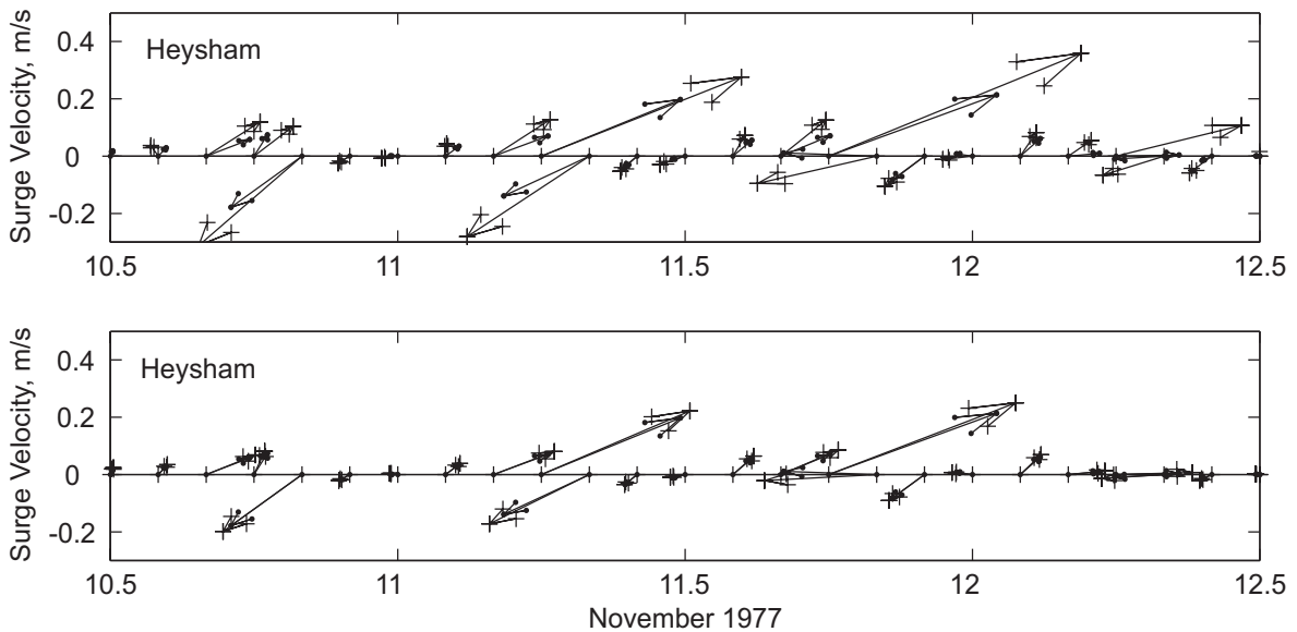
Fig. 11 Surge (residual) depth – averaged current vectors every 2 hours at Heysham, located in Fig. 3, during the period 10 th November (12:00) to 12 th November (12:00) 1977. The vector arrows depicted with dotted end points represent the actual 1977 surge conditions, while the arrows depicted by crossed end points represent the 1977 surge under future scenario conditions as follows: In the top panel a 1.4m sea level rise is included and in the bottom panel a 10% increase in wind speed is included. The time resolution is the day in November, e.g. 10 = 00:00 10 th November and 10.5 = 12:00 10 th November
