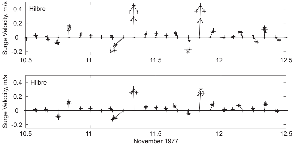
Fig. 12 Surge (residual) depth – averaged current vectors every 2 hours at Hilbre, located in Fig. 3, during the period 10 th November (12:00) to 12 th November (12:00) 1977. The vector arrows depicted with dotted end points represent the actual 1977 surge conditions, while the arrows depicted by crossed end points represent the 1977 surge under future scenario conditions as follows: In the top panel a 1.4m sea level rise is included and in the bottom panel a 10% increase in wind speed is included. The time resolution is the day in November, e.g. 10 = 00:00 10 th November and 10.5 = 12:00 10 th November
