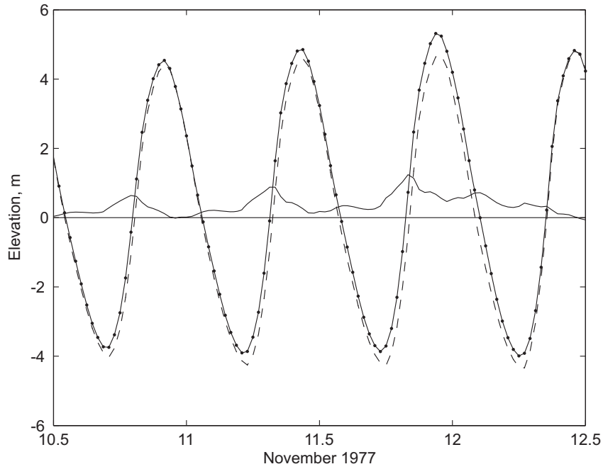
Fig. 2 The total (surge + tide) elevation (—●—), tidal elevation (---) and surge elevation (—) at Hilbre during the November 1977 event. The time resolution is the day in November, e.g. 10 = 00:00 10 th November and 10.5 = 12:00 10 th November
