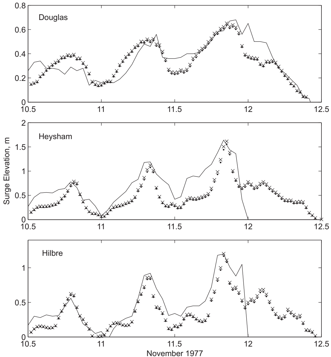
Fig. 5 Surge prediction using S&B (●) and a Charnock parameter of 0.0144 (×), using POLCOMS with a minimum depth of 5m, compared to tide gauge data (–). Douglas represents a deep location, while Heysham and Hilbre represent shallow locations along the Sefton coast. The time resolution is the day in November, e.g. 10 = 00:00 10 th November and 10.5 = 12:00 10 th November
