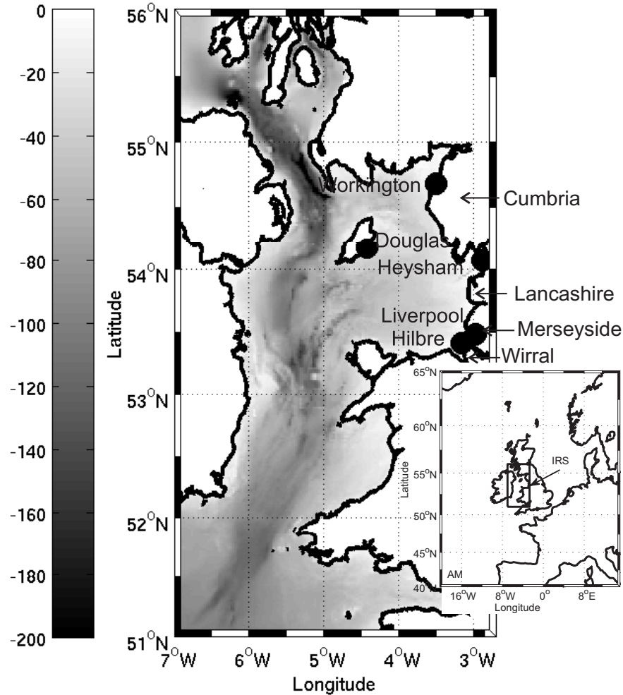
Fig. 3 The Irish Sea model domain and the coastal tide gauges used to validate the surge elevation predicted by the modelling system, during November 1977 (+). The nested model domains for the Atlantic Margin model (AM) and the Irish Sea model (IRS) are shown in the bottom right corner
