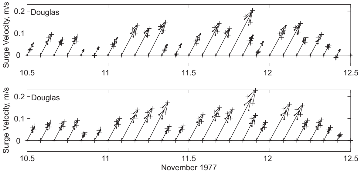
Fig. 10 Surge (residual) depth – averaged current vectors every 2 hours at Douglas, located in Fig. 3, during the period 10 th November (12:00) to 12 th November (12:00) 1977. The vector arrows depicted with dotted end points represent the actual 1977 surge conditions, while the arrows depicted by crossed end points represent the 1977 surge under future scenario conditions as follows: In the top panel a 1.4m sea level rise is included and in the bottom panel a 10% increase in wind speed is included. The time resolution is the day in November, e.g. 10 = 00:00 10 th November and 10.5 = 12:00 10 th November
