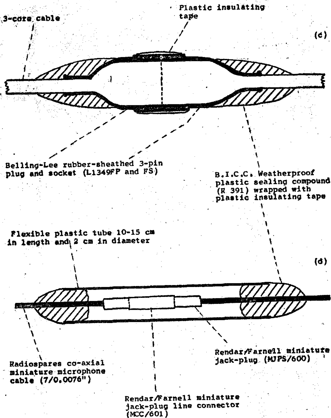
Figure 3 (continued). Types of cable junction for field use:
