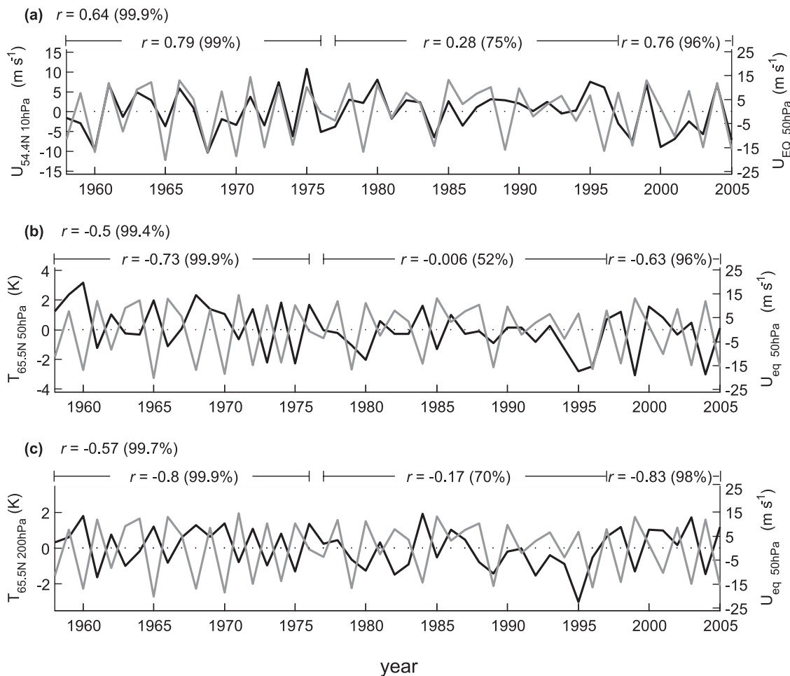
Figure 3. Time series (black lines) of the extratropical zonal-mean (a) zonal wind at 54.4°N, 10 hPa and (b) and (c) temperature anomalies at 65.5°N, 50 hPa and at 65.5°N, 200 hPa, respectively, plotted against zonal-mean zonal wind at the equator at 50 hPa averaged over the extended winter period (November–March) (gray lines). The correlation coefficients and confidence levels (in brackets) for the entire period of 1958–2006 are given on the top of each sub-plot together with those for the sub-periods of 1958–1976, 1977–1997, and 1998–2006.
