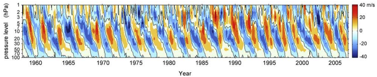
Figure 1. The QBO time series (i.e., de-seasonalized monthly mean zonal mean zonal wind at the equator) in \text{m s}^{-1} extracted from ERA-40 and ECWMF operational on 11 pressure levels from 1958 to 2006. Red and blue colors represent westerly and easterly winds. The black solid lines are zero wind lines.
