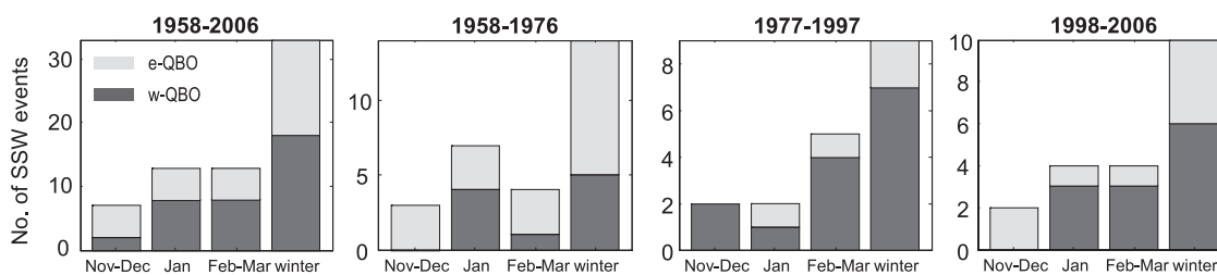
Figure 8. Major SSW occurrence grouped by early, middle, late and extended winter and the phases of the QBO, for the periods of 1958–2006, 1958–1976, 1977–1997, and 1998–2006 (from left to right). Westerly and easterly QBO are defined as >/< 0 , respectively.
