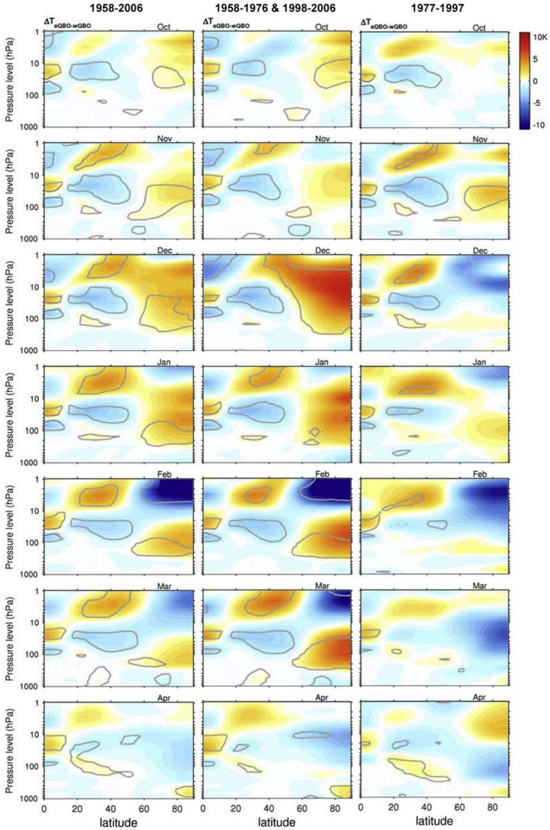
Figure 7. Same as Figure 6 but for the temperature anomalies.
