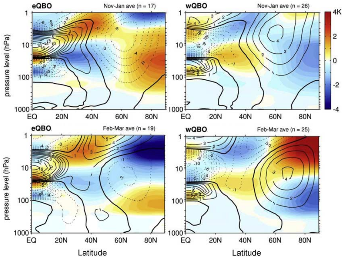
Figure 2. e-QBO (left-hand panels) and w-QBO (right-hand panels) composites of the zonal mean zonal wind (lined contours) and temperature anomalies (color shaded contours) for November to January mean (top panels), and for February and March mean (bottom panels). Thick solid lines represent zero wind. The QBO phases, the calendar months, with the total number of data samples indicated on the top of each panel.
