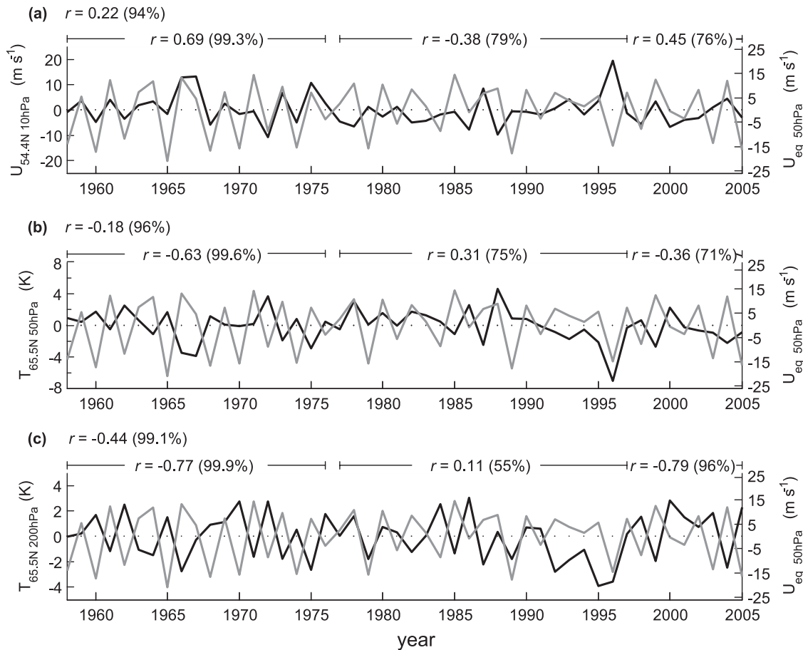
Figure 4. Same as Figure 3 but for late winter (February–March) averages.
