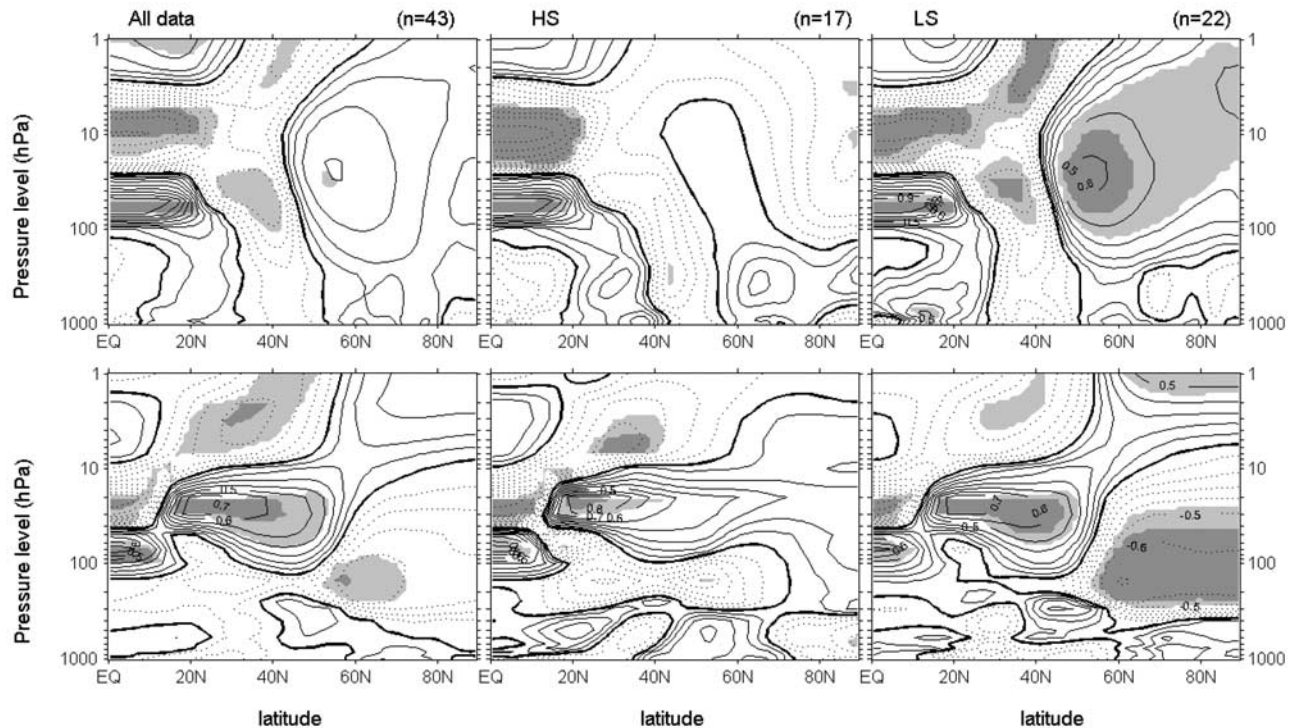
Figure 9. Linear correlations between January-February mean QBO and January-February mean zonal wind anomalies (1st row), and temperature anomalies (2nd row), under all solar conditions (1st column), when December-February mean F10.7 solar radio flux F_{10.7} is high (2nd column), and when F_{10.7} is low (3rd column). High/low F10.7 is defined as the standardized F_{10.7} >< than \pm 0.2 . The contour interval is \pm 0.1 and the thick black contour is zero correlation. The light and dark shaded areas indicate that the differences are statistically significance from zero with a confidence level of 90% and 95% or above, respectively.
