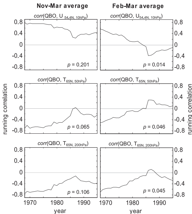
Figure 5. Running correlation coefficients between the equatorial QBO and the NH polar wind anomaly (first row) & temperature anomalies (second and third rows) with a 21-year window, using November to March mean (left-hand panels) and February to March mean (right-hand panels). The time series of the wind and temperature anomalies are the same as those shown in Figures 3 and 4. The p values represent the levels of statistical significance in terms of the difference between the maximum and minimum values of the running correlation. See text for details.
