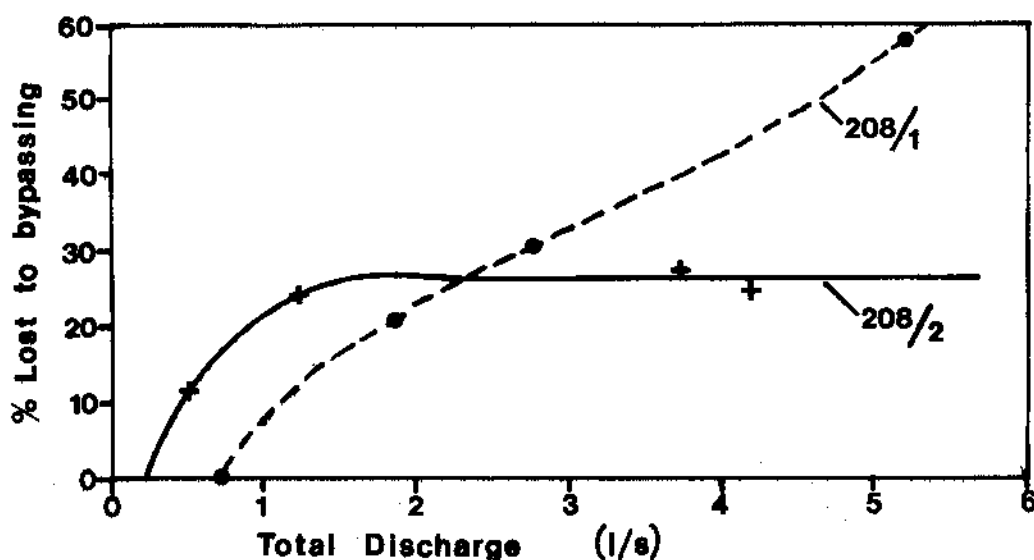
FIGURE 3.5 BYPASSING RELATIONSHIPS FOR PLOVER CLOSE GULLIES
