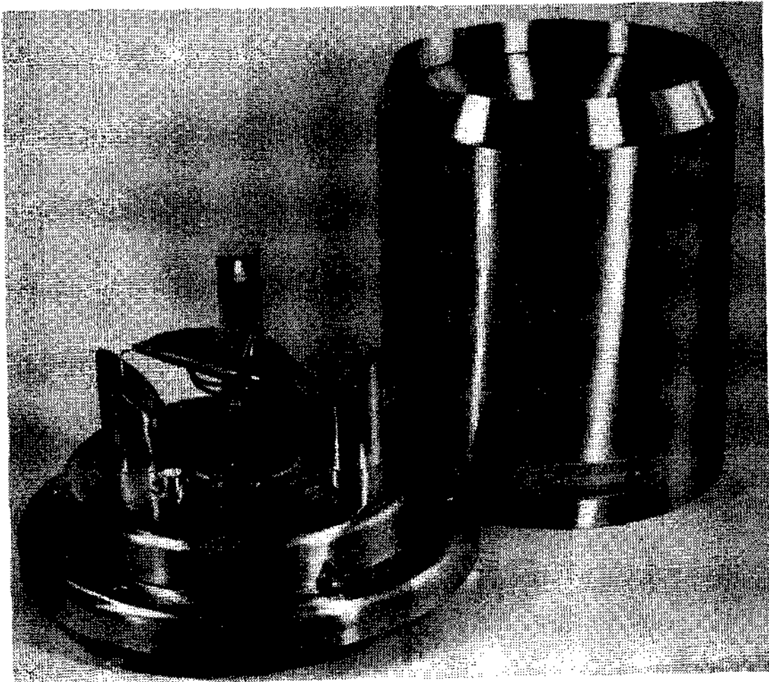
FIGURE 2.6 RIMCO RAINGAUGE WITH COLLECTOR REMOVED
