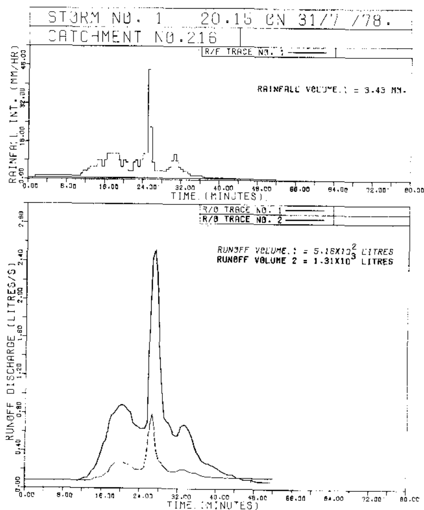
FIGURE 2.13 EXAMPLE OF PLOTTED EVENT
