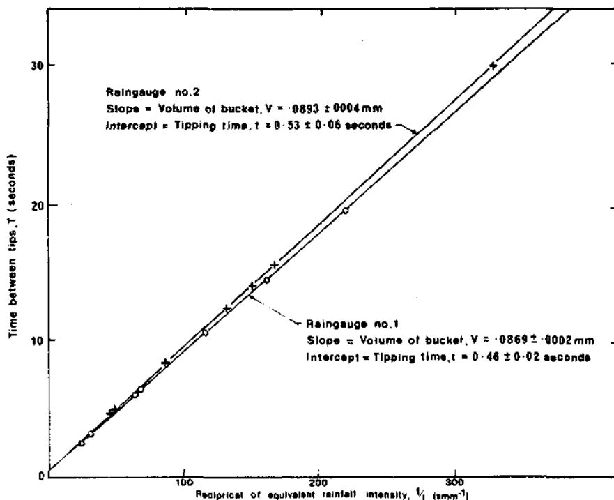
FIGURE 2.7 CALIBRATION OF RAINGAUGE, AFTER CALDER AND KIDD
