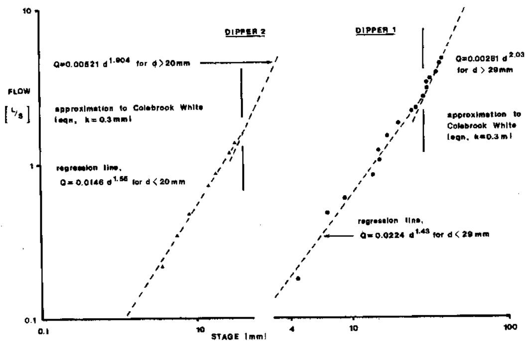
FIGURE 3.9 DIPPER CALIBRATIONS FOR ENNERDALE ONE
