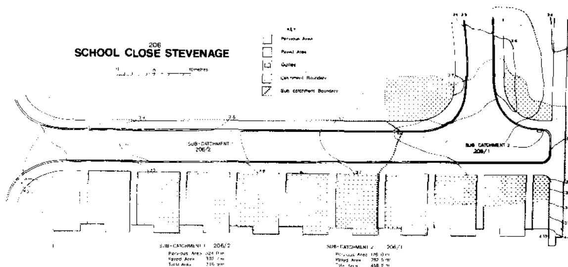
FIGURE 3.1 PLAN OF SCHOOL CLOSE ONE
