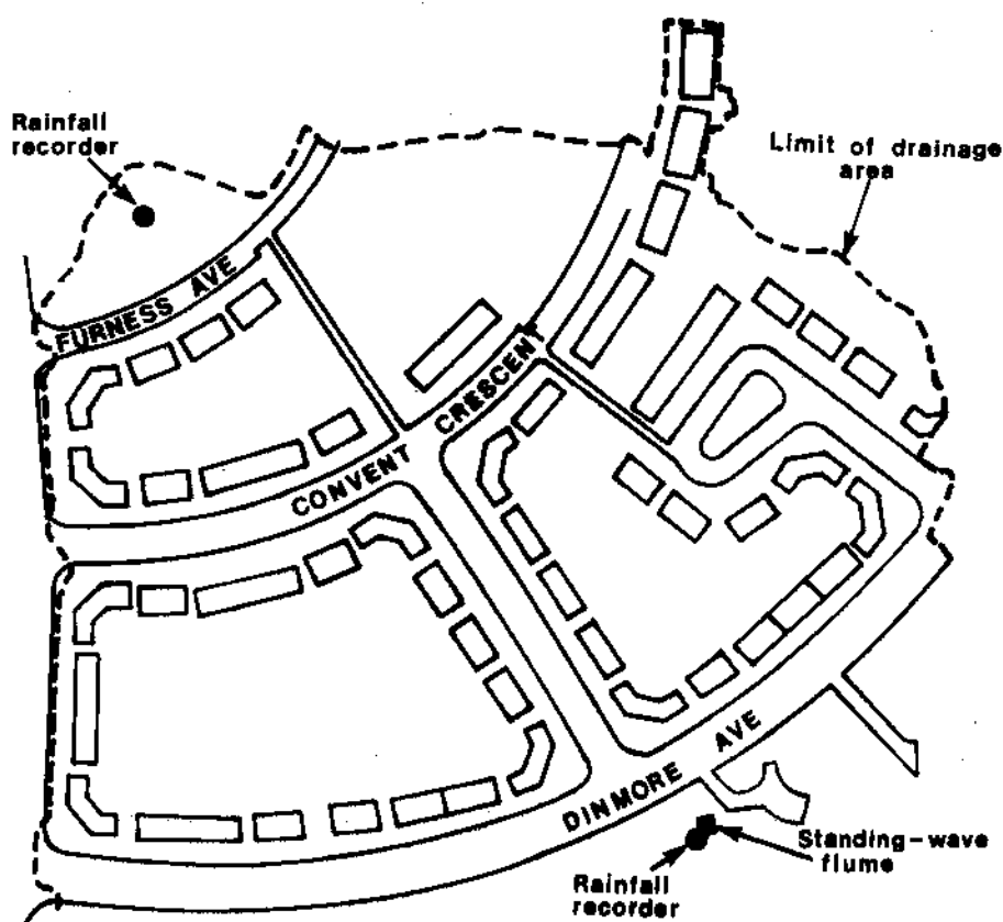
FIGURE 5.3 PLAN OF BLACKPOOL DRAINAGE AREA
