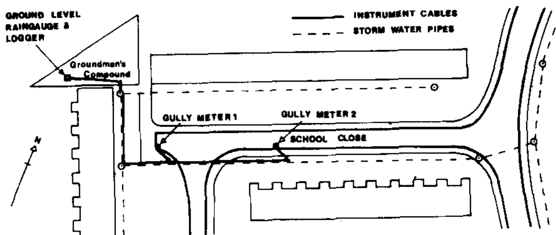
FIGURE 2.10 SCHEMATIC DIAGRAM OF SCHOOL CLOSE DATA COLLECTION SYSTEM
