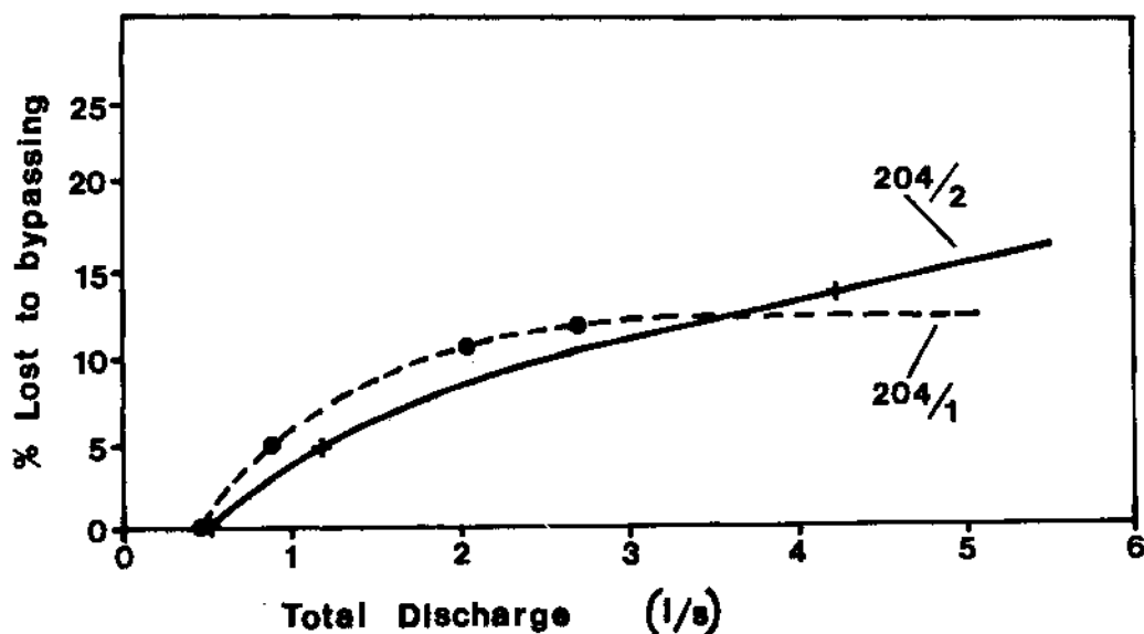
FIGURE 3.7 BYPASSING RELATIONSHIPS FOR BISHOPDALE GULLIES
