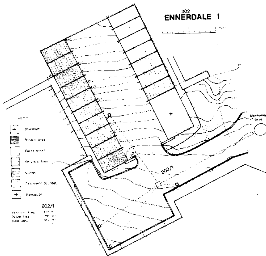
FIGURE 3.8 PLAN OF ENNERDALE ONE
