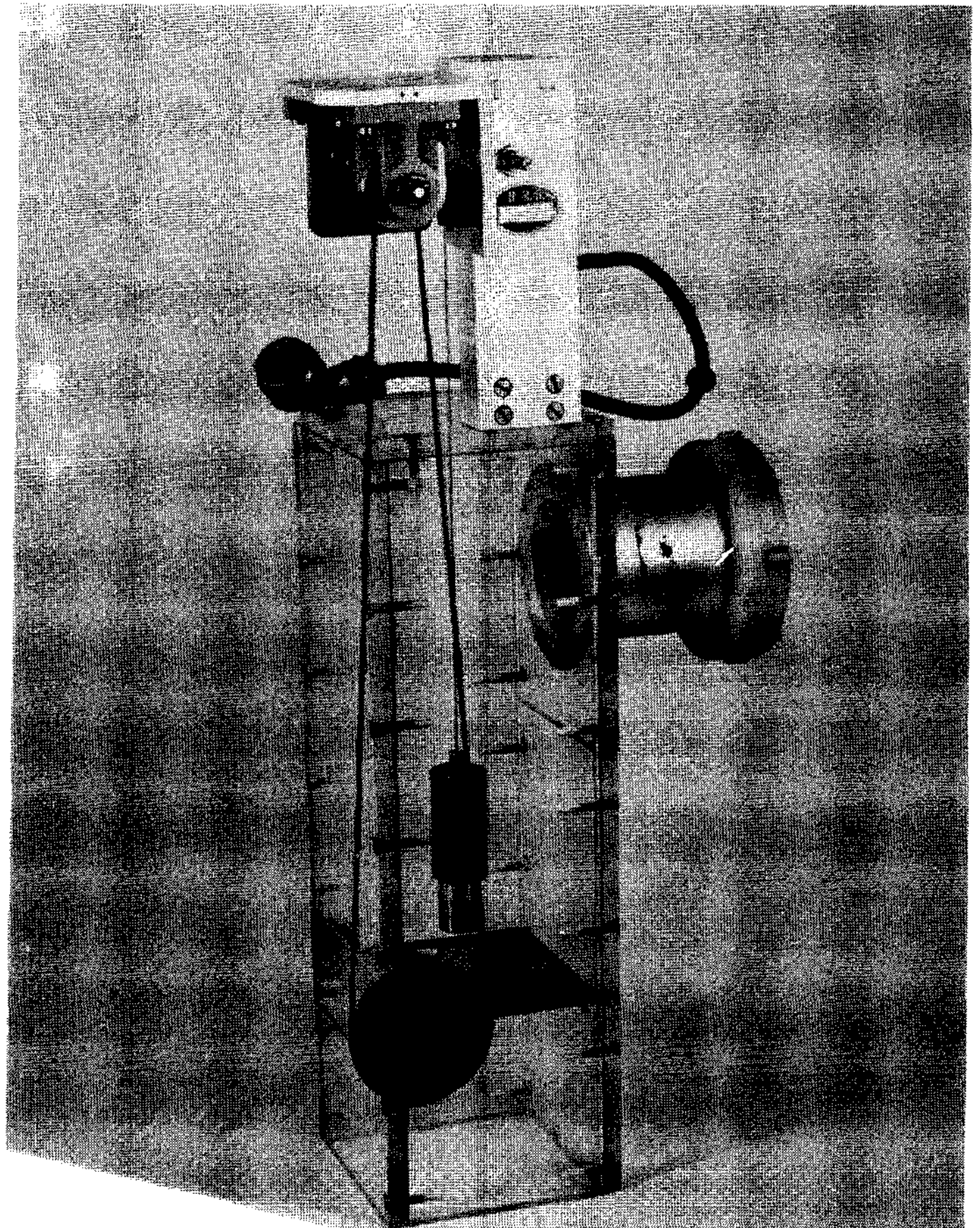
FIGURE 2.1 IH GULLY METER
