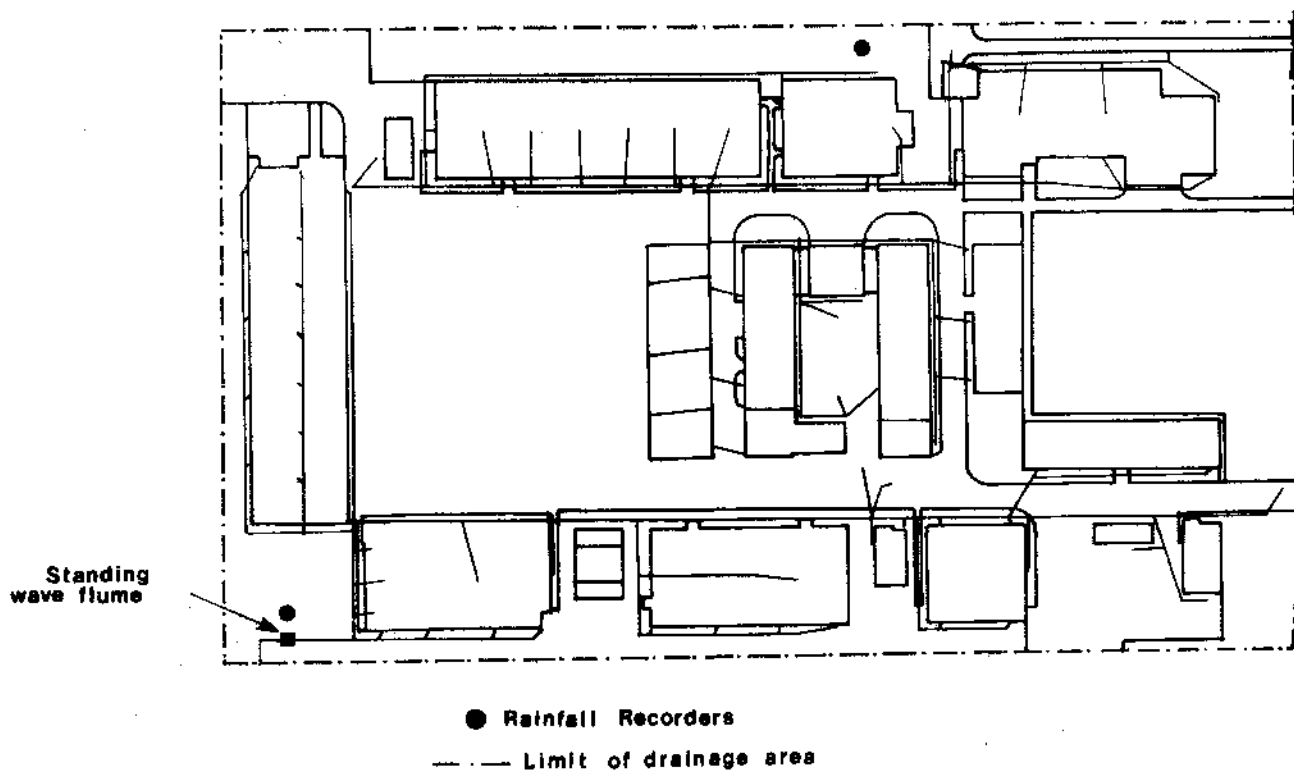
FIGURE 5.7 KIDBROOKE GOVERNMENT TRAINING CENTRE
