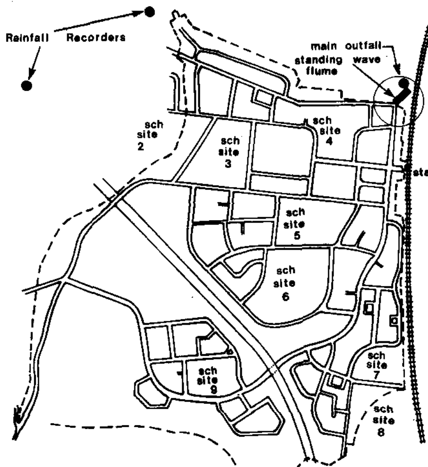
FIGURE 5.4 OXHEY DRAINAGE AREA
