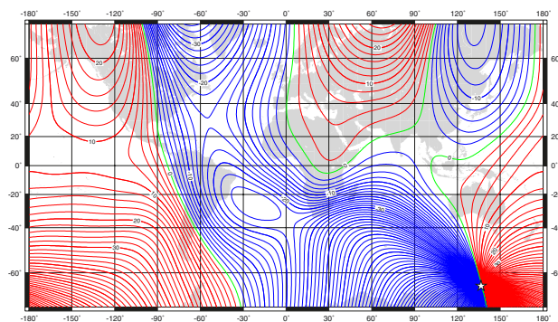
Declination (magnetic variation) at 2015.0 from the World Magnetic Model (WMM2015v2). Red - positive (east), blue - negative (west), green - zero (agonic line). Contour interval is 2°, white star is location of a magnetic pole and projection is Mercator. This is an example of an isogonic chart. Credit: British Geological Survey (UK Research and Innovation)
