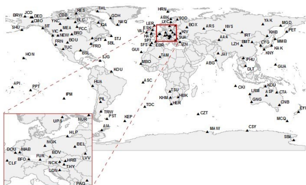
INTERMAGNET observatories contributing to the 2014 annual definitive data publication.
