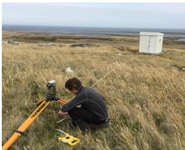
Surveying for RFI at Port Stanley Observatory, Falkland Islands
