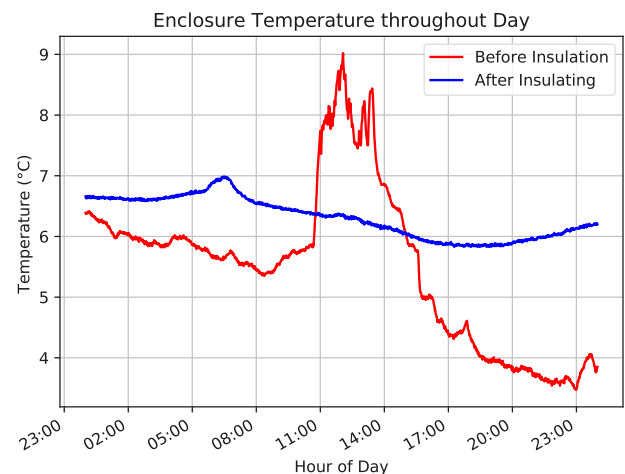
Thermally insulating the enclosure has reduced the temperature variation caused by solar heating of the enclosure roof
