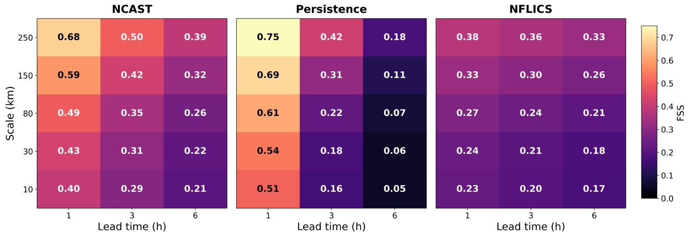
FIGURE 12 Fractions skill score for NCAST, persistence, and NFLICS as a function of spatial scale and lead time.
