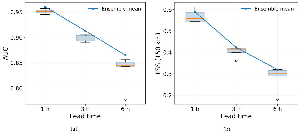
FIGURE 10 Performance of the five-member NCAST ensemble at lead times of 1, 3, and 6 h. Boxplots show the distribution of scores across the five independently trained ensemble members, while the line shows the ensemble forecast obtained by pixelwise averaging of member probabilities prior to evaluation. Ensemble averaging consistently improves AUC, while FSS remains comparable with the distribution of individual members. (a) Area under the receiver operating characteristic curve (AUC). (b) Fractions skill score (FSS) evaluated at a spatial scale of 150 km.
