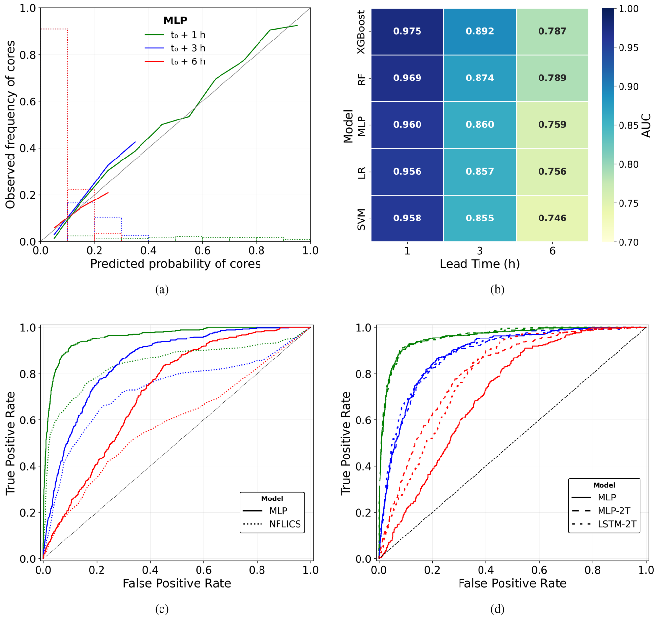
FIGURE 4 Performance of the single-location object-based framework over Dakar at forecast lead times of 1, 3, and 6 h (green, blue, and red, respectively). (a) Reliability and sharpness diagrams for the MLP; the grey diagonal indicates perfect reliability. (b) AUC values for the benchmark machine-learning models: logistic regression (LR), support-vector machine (SVM), multilayer perceptron (MLP), random forest (RF), and extreme gradient boosting (XGBoost). (c) ROC curves comparing the MLP with the NFLICS conditional climatology. (d) ROC curves comparing the MLP, MLP-2T, and LSTM-2T architectures. In panels (c) and (d), the diagonal line indicates no discrimination skill.
