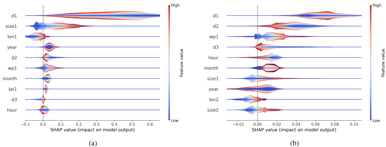
FIGURE 5 SHAP summary plots for the 10 most influential features in the single-time-step MLP model at forecast lead times of (a) 1 h and (b) 3 h. Features are ordered by mean absolute SHAP value, with colour indicating the feature magnitude.
