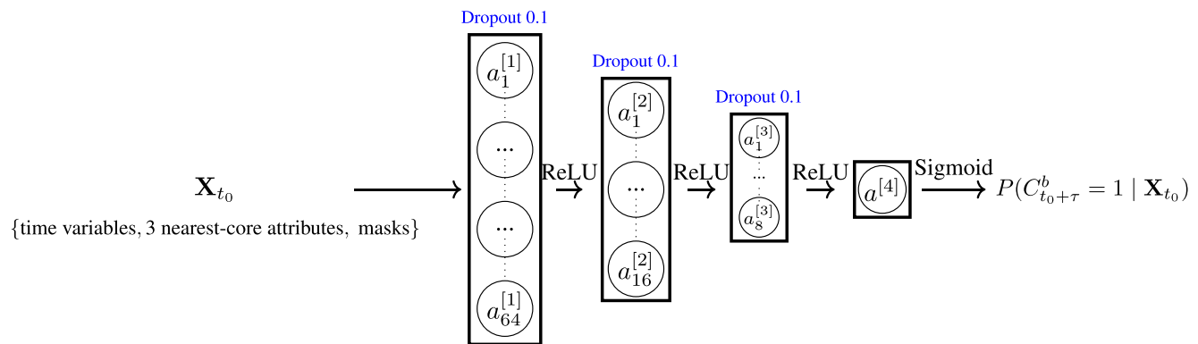
FIGURE 2 Neural-network architecture of the single-location MLP. The illustrated configuration corresponds to the architecture selected for the 3-h forecast lead time. The input vector \mathbf{X}_{t_0} contains time variables, attributes of the three nearest convective cores at the nowcast origin time t_0 , and binary mask variables indicating padded cores. The model comprises hidden layers containing 64, 16, and 8 neurons with ReLU activations and dropout regularisation. A sigmoid output neuron produces the probability P(C_{t_0+\tau}^b = 1 | \mathbf{X}_{t_0}) of convective-core occurrence over the target location. The architectures selected for the other forecast lead times are summarised in Table 2.
