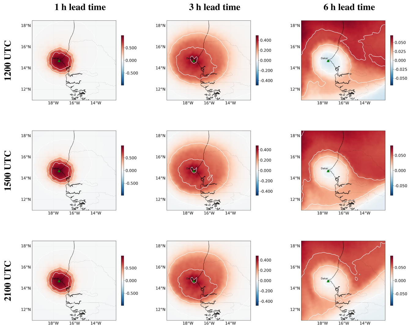
FIGURE 7 Spatial sensitivity of the single-location MLP model to the placement of a synthetic three-core cluster on July 15, 2020. Panels show probability differences relative to NFLICS unconditional climatology. Columns correspond to lead times of 1, 3, and 6 h; rows to nowcast origin times (1200, 1500, and 2100 UTC). Colour scales differ across lead times.
