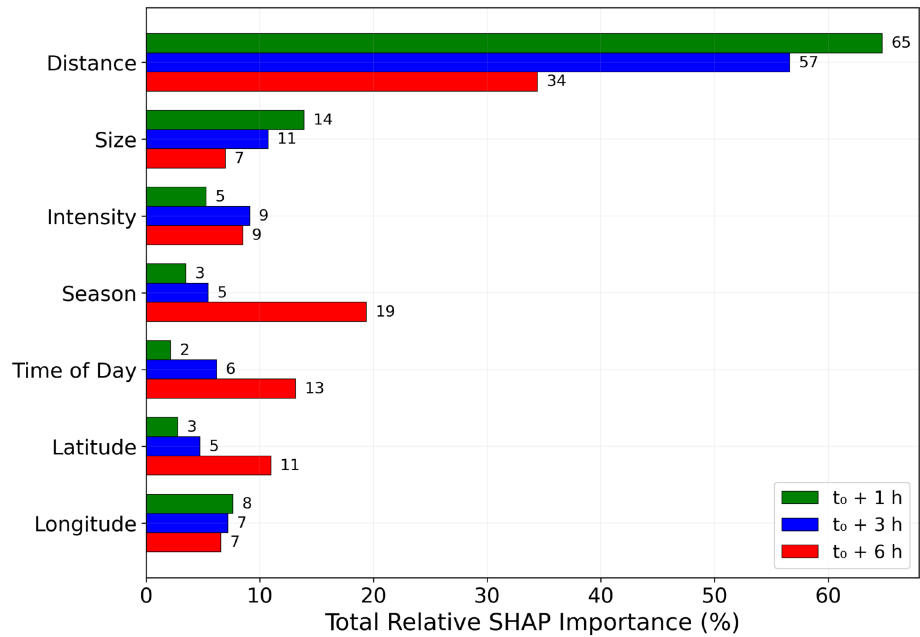
FIGURE 6 Relative SHAP importance of grouped features at 1-, 3-, and 6-h forecast lead times. Each bar shows the normalised contribution of feature groups to model predictions, averaged over the test set.
