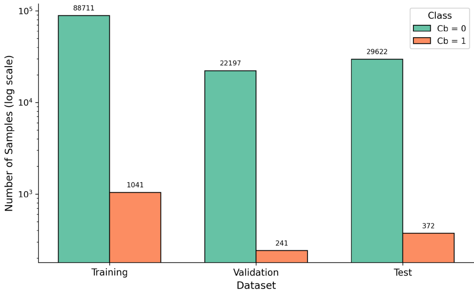
FIGURE A2 Class distribution across the training, validation, and test sets for the 1-h lead time in Dakar. Bars show the number of samples with ( y_{t_0+1h} = 1 ) and without ( y_{t_0+1h} = 0 ) convective-core occurrence. The pronounced class imbalance highlights the difficulty of standard binary classification metrics.
