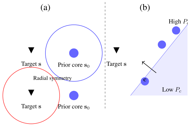
FIGURE 16 Schematic interpretation of the conditional probability field P_c(\mathbf{s}, t_1 | \mathbf{s}_0, t_0) . (a) In an isotropic environment, the conditional probability depends only on radial distance r = \|\mathbf{s} - \mathbf{s}_0\| and is maximised along an expanding ring centred on the prior core. (b) With propagation in direction \mathbf{c} , anisotropy arises: the conditional probability is structured by the projection (\mathbf{s} - \mathbf{s}_0) \cdot \mathbf{n} , producing linear level sets in prior-core space.
