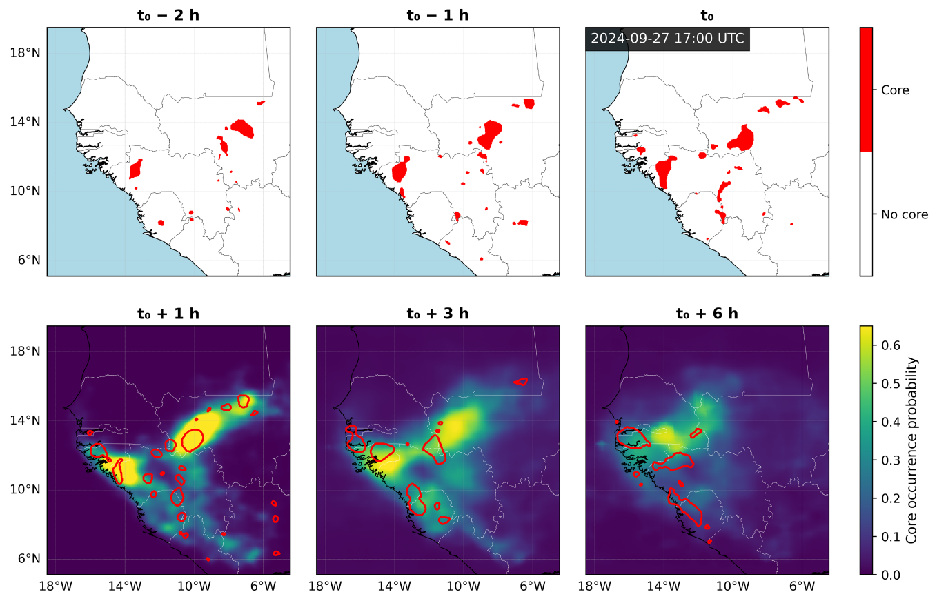
FIGURE 14 Example NCAST forecast for a multi-core convective system over the western Sahel, initialised at t_0 = September 27, 2024, 1700 UTC. Top row: observed convective cores (filled red) at t_0 - 2 h, t_0 - 1 h, and t_0 . Bottom row: probabilistic forecasts valid at verification times t_0 + 1 h, t_0 + 3 h, and t_0 + 6 h. Observed convective cores at the corresponding verification times are shown as unfilled red outlines.
