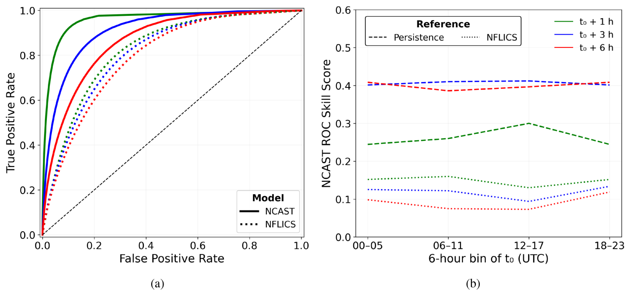
FIGURE 11 Pixelwise evaluation of NCAST over the western Sahel. Forecast lead times of 1, 3, and 6 h are shown in green, blue, and red, respectively. (a) ROC curves for NCAST (solid) and NFLICS (dotted). (b) ROCSS relative to persistence (dashed) and the operational NFLICS conditional climatology (dotted), stratified by 6-h bins of nowcast origin.
