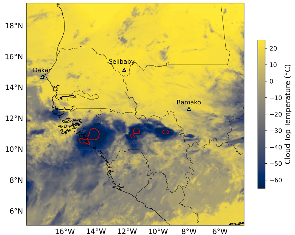
FIGURE 1 Cloud-top temperature (CTT; °C) from the MSG IR 10.8- \mu\text{m} channel over the western Sahel study domain on July 3, 2023 at 1515 UTC. Convective cores (red outlines) are identified using a two-dimensional wavelet transform.
