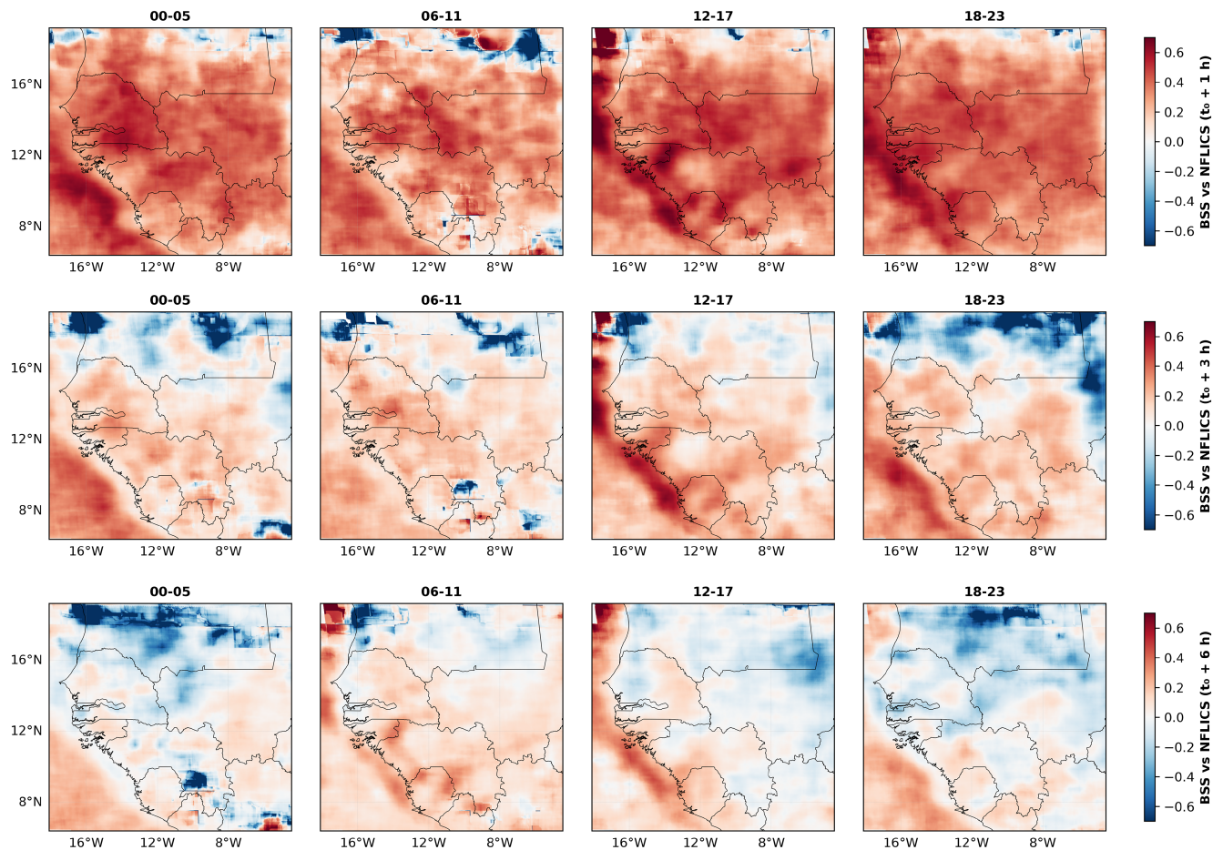
FIGURE 13 Spatial distribution of the pixelwise Brier skill score (BSS) of NCAST relative to NFLICS over the western Sahel, shown for lead times of 1, 3, and 6 h and averaged by 6-h bins of the nowcast origin (UTC). Rows correspond to forecast lead times and columns to 6-h bins of the nowcast origin. Warm colours indicate positive BSS (added skill of NCAST relative to NFLICS), cool colours indicate negative BSS, and white corresponds to near-zero skill difference.
