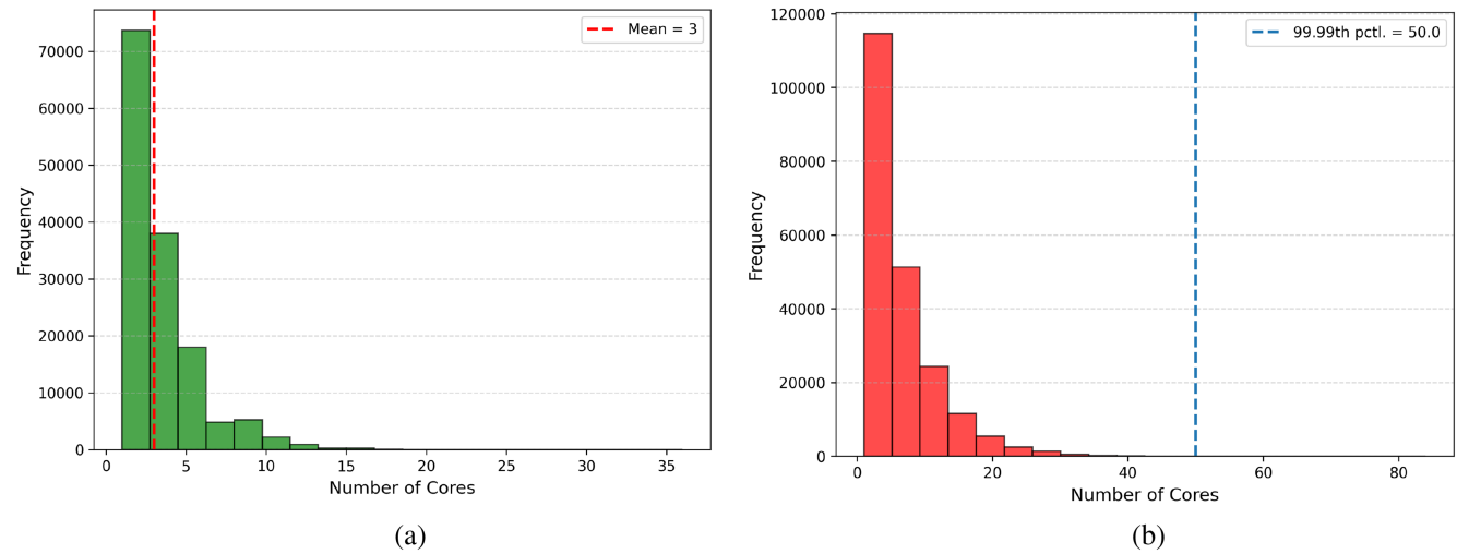
FIGURE A1 Distribution of detected convective core counts at 15-minute intervals during 2004–2024, conditioned on the presence of at least one core. Panel (a) shows the 12° × 12° Dakar context domain, and panel (b) the western Sahel (WS) domain. The dashed lines indicate (a) the mean and (b) the 99.99th percentile, respectively. Figure A1 shows the distribution of detected convective-core counts in the Dakar and western Sahel domains, while Figure A2 shows the class distribution across the training, validation, and test sets for the Dakar application.
