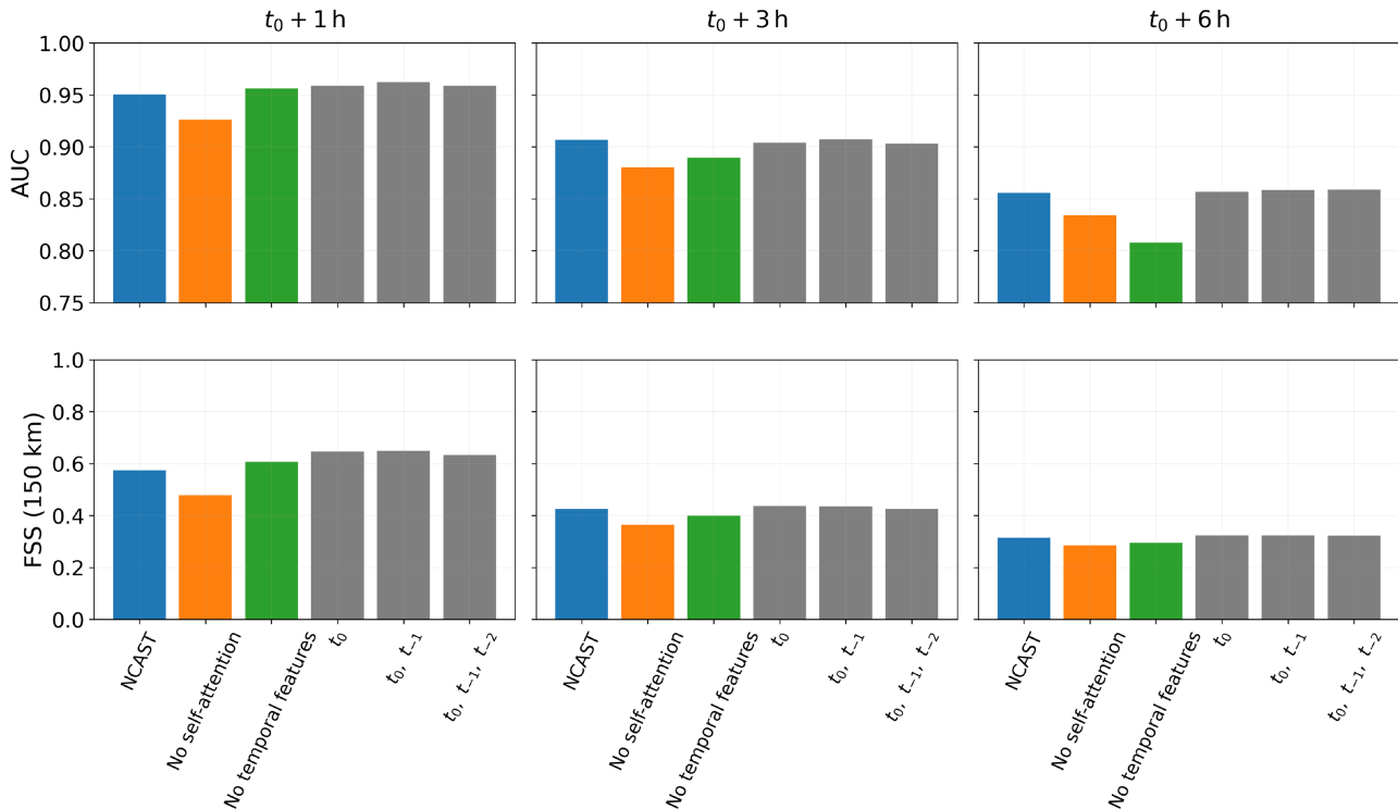
FIGURE 15 Ablation study of NCAST at forecast lead times of 1, 3, and 6 h. The top row shows the area under the receiver operating characteristic curve (AUC) and the bottom row shows the fractions skill score (FSS) evaluated at a spatial scale of 150 km. The full model is compared with variants without self-attention, without temporal features, and with reduced temporal input histories. Removing self-attention produces the largest reduction in both discrimination and spatial skill, highlighting the importance of modelling interactions between convective cores. Temporal features become increasingly important at longer lead times. In contrast, extending the temporal input history beyond one previous observation yields only modest additional improvements with the current architecture.
