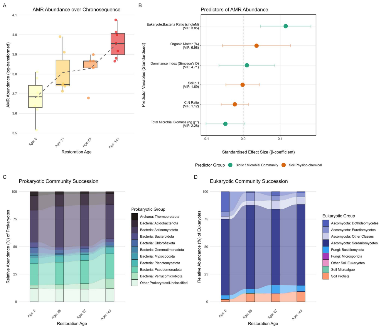
Figure 1 Soil resistome expansion, statistical predictors, and multi-kingdom taxonomic succession across the chronosequence; (A) AMR abundance over chronosequence: log-transformed total AMR gene abundance normalized to fragments per kilobase per million mapped reads on the chromosome ( \log_{10} FPKPMC +1) and mapped across the soil chronosequence; box plots indicate the median and interquartile range, individual points represent raw sample replicates ( n = 24 ); the dashed trendline tracks the shift in group means over time; (B) drivers of AMR abundance: standardized effect size ( \beta -coefficient) plot generated from a generalized least squares (GLS) multivariable model evaluating the direct predictors of soil AMR abundance; horizontal error bars signify 95% confidence intervals; biotic variables utilize low-variance inflation factor metrics, including total microbial biomass ( \text{ng g}^{-1} dry soil) derived from microbial-specific phospholipid fatty acid extractions, and the Eukaryote:Bacteria ratio mapped via universal single-copy ribosomal marker genes (singleM); (C) prokaryotic community succession (SingleM): alluvial profile showing the relative abundance transitions (%) of dominant bacterial and archaeal phyla across the restoration timeline; (D) eukaryotic community succession (Kraken2): taxonomic succession of the soil eukaryotic community filtered to exclude macro-organism; fungal reads are partitioned into dominant classes of the Ascomycota phylum ( Sordariomycetes , Dothideomycetes , Eurotiomycetes ) alongside Basidiomycota , Microsporidia , and soil protists to visualize shifting trophic complexity.
