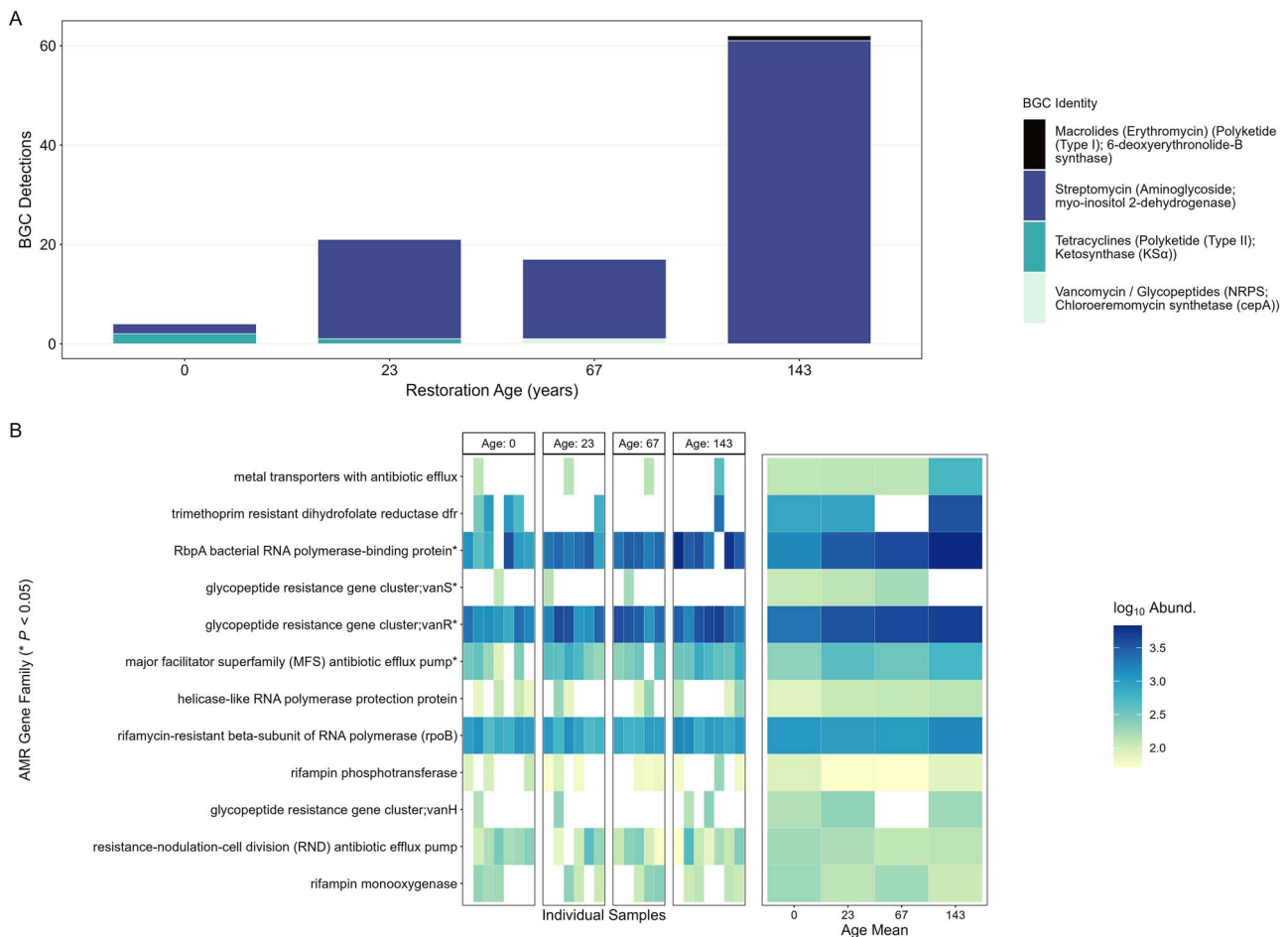
Figure 2 BGCs and resistome dynamics across the chronosequence; (A) stacked bar plot showing relative abundance and detection profiles of individual BGCs; (B) heatmaps tracking the dynamics of AMR gene families across individual samples (left panel) and their group-level mean log-transformed abundance per restoration age (right panel); asterisks (*) denote gene families exhibiting statistically significant linear abundance shifts across the chronosequence ( P < .05 ), and only those with valid linear model slopes are displayed (see Supplementary Table S2 for full list of detected AMR gene families).
