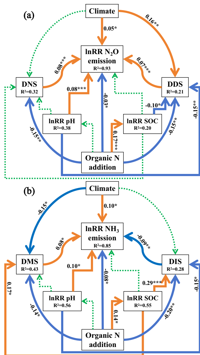
Fig. 3 | Multiple drivers of reactive nitrogen gas emissions under organic substitution. Structural equation models showing the drivers of N 2 O emissions (a) and NH 3 (b) under organic substitution. Orange solid lines indicate significantly positive relationships, blue solid lines indicate significantly negative relationships, and green dashed lines indicate non-significant relationships. Numbers adjacent to lines are standardized coefficients. R 2 values indicate the proportion of variance explained for each endogenous variable. DMS is synchrony deviation of mineralization, DIS is synchrony deviation of immobilization, DNS is synchrony deviation of nitrification, and DDS is synchrony deviation of denitrification. InRR N 2 O emission is the effect size of N 2 O emission under organic substitution; InRR NH 3 emission is the effect size of NH 3 emission under organic substitution. InRR pH is the effect size of pH under organic substitution. InRR SOC is the effect size of soil organic carbon under organic substitution. Climate represents a composite climatic variable comprising mean annual temperature and mean annual precipitation. Organic N addition represents the organic nitrogen addition rate. * p < 0.05; ** p < 0.01; and *** p < 0.001.
