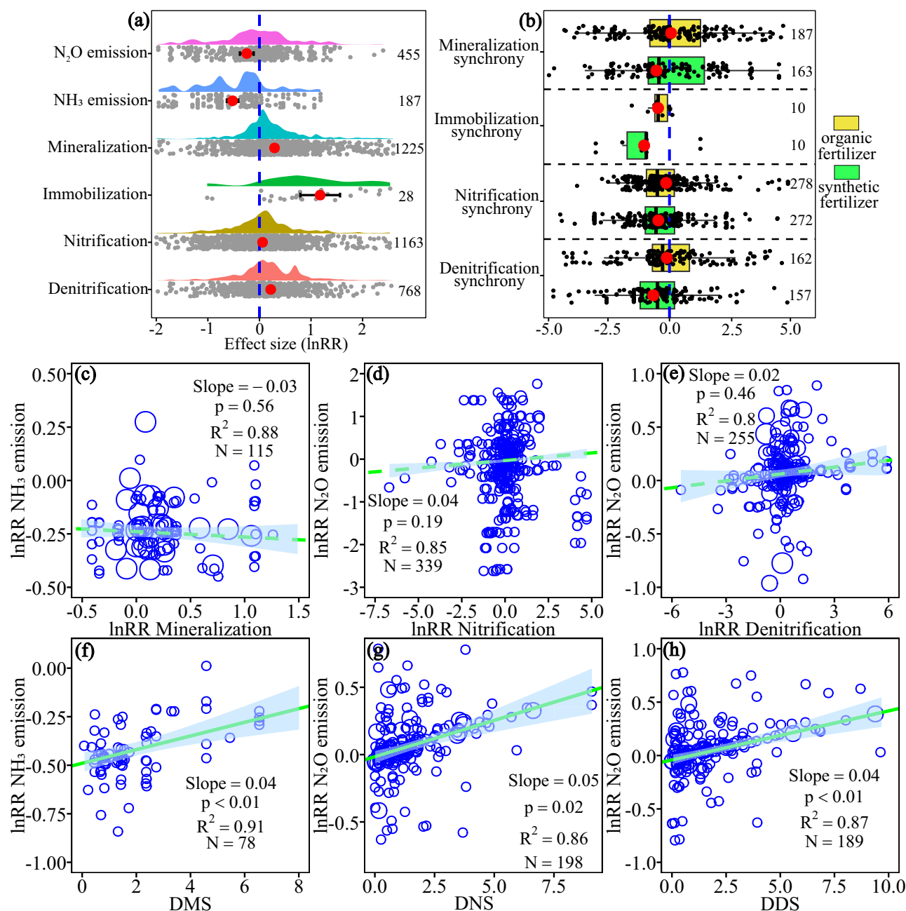
Fig. 2 | Effects of organic substitution on reactive nitrogen gas emissions and nitrogen process synchrony. Changes in reactive nitrogen gas emissions and nitrogen processes under organic substitution (a) and comparison of synchrony of four nitrogen processes between organic substitution and synthetic fertilizer (b), as well as bivariate relationships of reactive nitrogen gas emissions against nitrogen processes (c–e) and synchrony deviations of nitrogen processes (f–h). In a, dots with error bars are the mean values \pm 95% confidence intervals. The vertical dashed line denotes a zero reference, and the response ratios differed significantly from zero when the 95% confidence intervals did not overlap with the zero reference. Black points represent individual observations. Numbers to the right of each dot are the sample sizes. In b, green boxplots are the synchrony of nitrogen processes under synthetic fertilizer relative to a no fertilizer control, and yellow boxplots are
