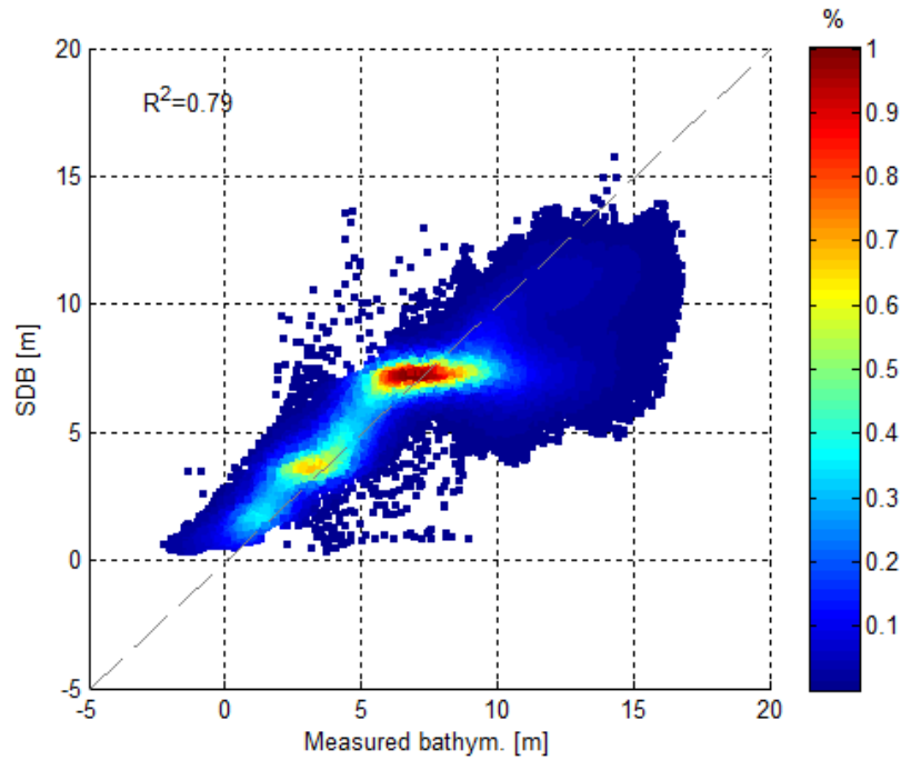
Figure 20: Scatterplot between measured and satellite derived bathymetry. The scale of colors indicate points' density, in percent.
