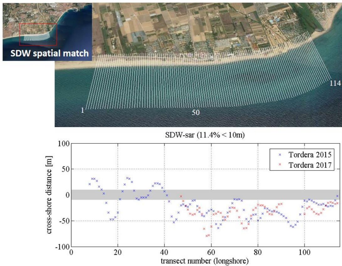
Figure 14: Cross-shore transects along the coast of Malgrat – Tordera Delta (a) and the distance between waterlines obtained from in-situ measurements and SDW-sar (b). The gray area indicates the range between \pm 10 m.
