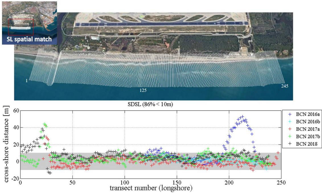
Figure 13: Cross-shore transects displaced in the area where the shorelines match (upper panel) and distance verified between measured and satellite-based shorelines in each of those transects. The gray area indicate the range between \pm 10 m.
