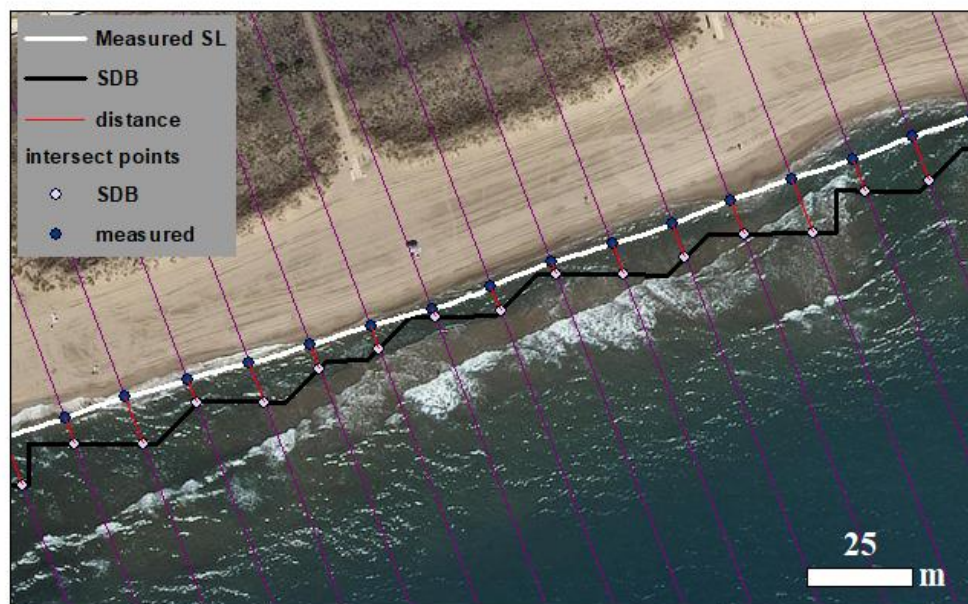
Figure 12: Intersect points and distance between measured and satellite-based shorelines.
