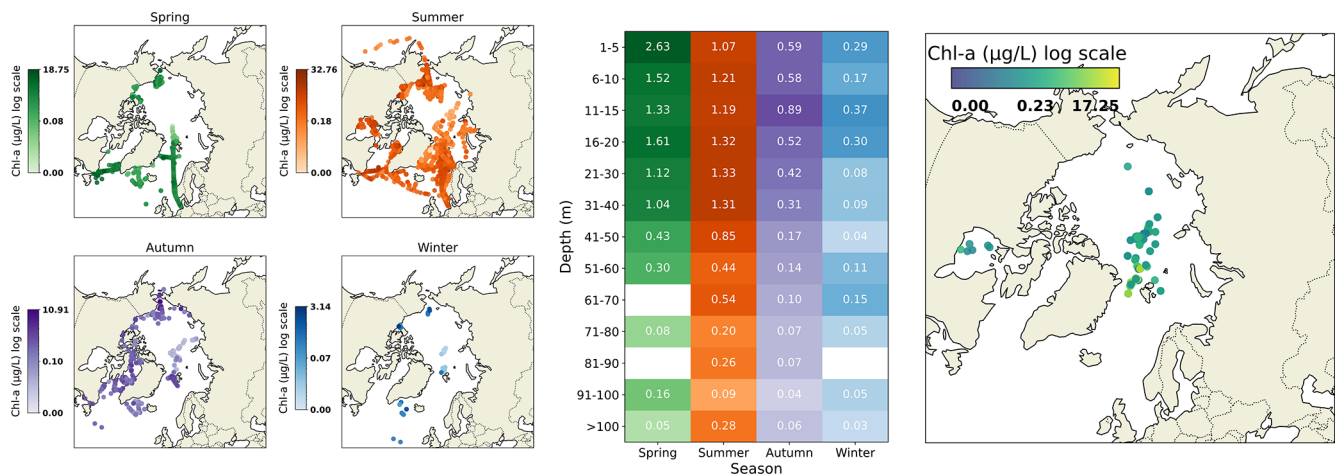
Figure 5. (a) Spatial distribution of all measured Chl a water samples in each season, shown as subplots for spring, summer, autumn and winter. Color mapping uses logarithmic scale, but the values themselves are not log-transformed. (b) Mean Chl a concentration as function of depth range (rows) and season (columns). Color indicates the average value for each depth/season bin. Missing color indicates that data is not available. (c) Spatial distribution of all measured Chl a for sea-ice samples.
