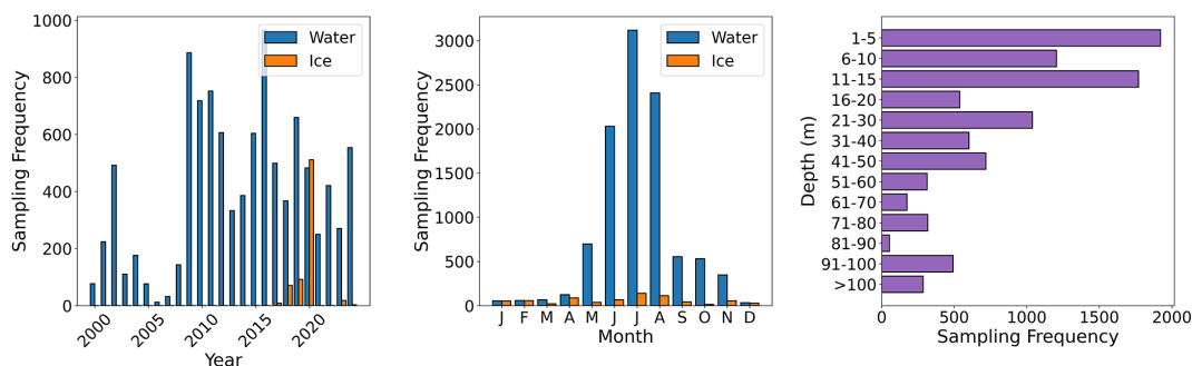
Figure 3. Leftpanel: yearly sampling frequency for water column and sea-ice samples, middle panel: monthly sampling frequency and right panel: number of water samples observations per depth bin. Note that for sea-ice samples, the vertical distribution is not presented due to inconsistencies in the ice core sampling methods among the different campaigns.
