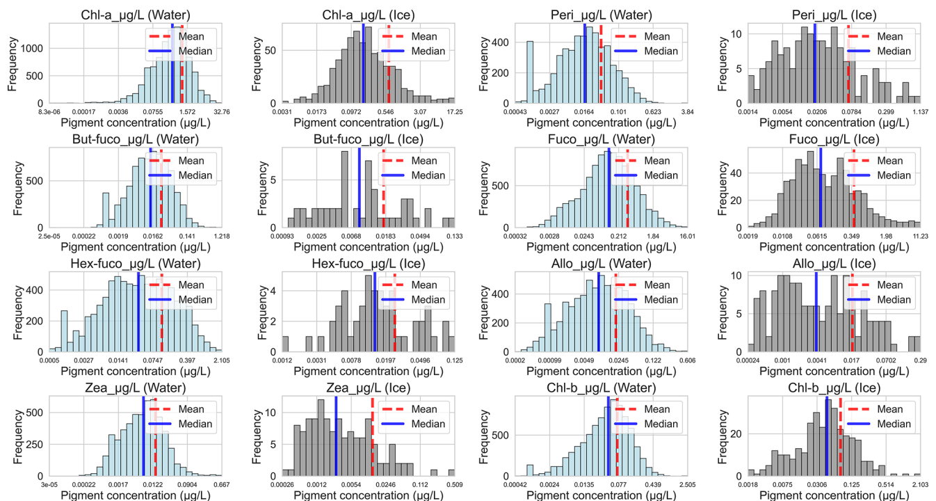
Figure 6. Frequency histograms displaying log-scaled pigment concentrations. Water samples are shown in blue and sea-ice samples are shown in grey. x axis represents actual pigment concentrations. Note the different ranges for y axis comparing water and sea-ice samples.
