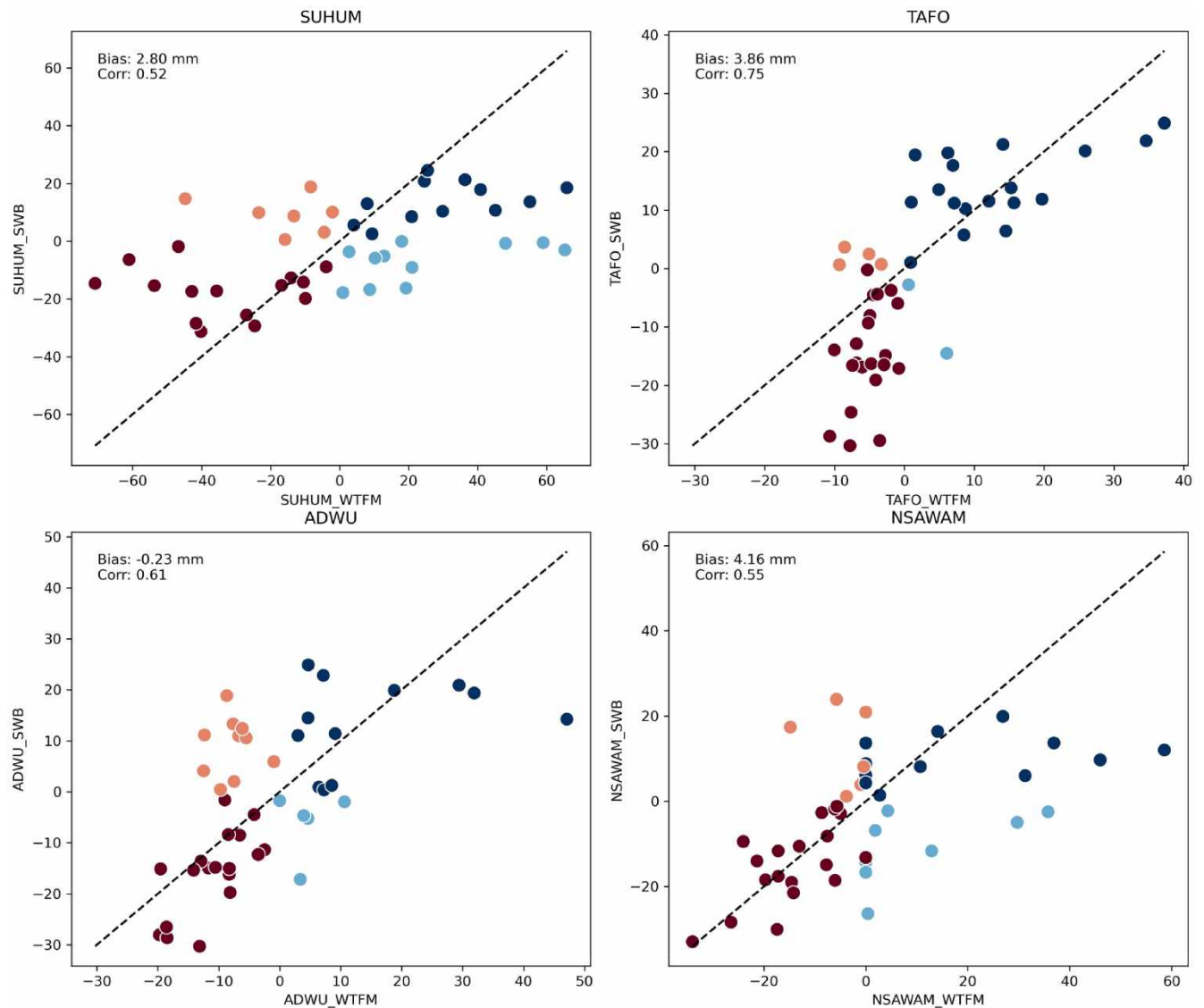
Figure 8 | Scatter plot of recharge estimates from the WTFM and the SWB method for Suhum, Tafo, Adwumako, and Nsawam. The clusters are color-coded as follows: -2 (deep red): both methods yield negative recharge; -1 (light red): WTFM negative and SWB positive; 1 (light blue): WTFM positive and SWB negative; 2 (deep blue): both methods yield positive recharge. The plot illustrates the agreement and disagreement between the two methods, influenced by soil properties, seasonal rainfall, and aquifer dynamics.
