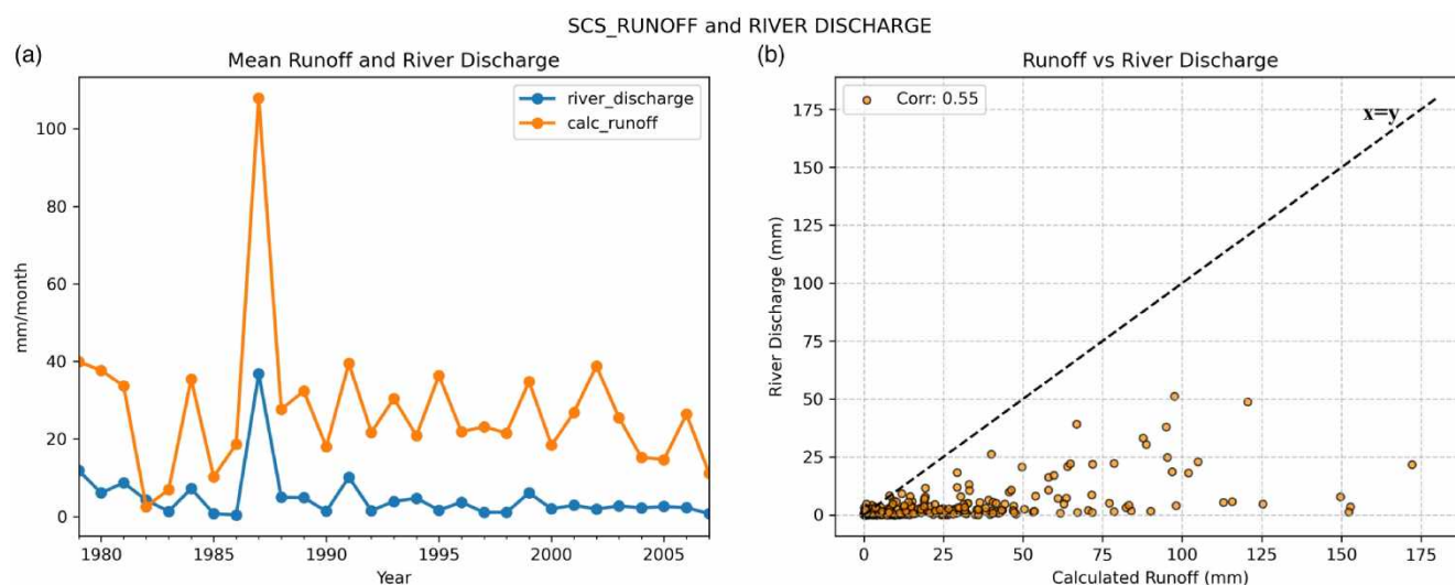
Figure 7 | Comparison between the mean SCS-calculated runoff (orange line) and river discharge (blue line) over time (a) and their correlation (b), where the scatter points represent the relationship between calculated runoff and river discharge, with the x = y line.
