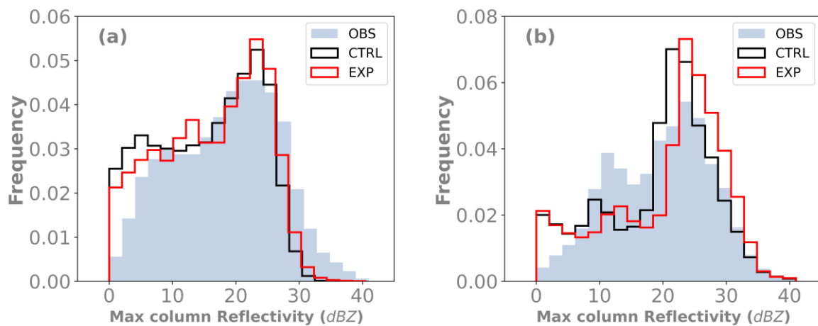
Fig. 8: Comparison of histograms of observed and modelled maximum radar reflectivity (dBZ) for the Alps on (a) 18 UTC 12 Jan 2019 and (b) 18 UTC 01 Dec 2023. The modelled outputs are from the CTRL and EXP simulations.
