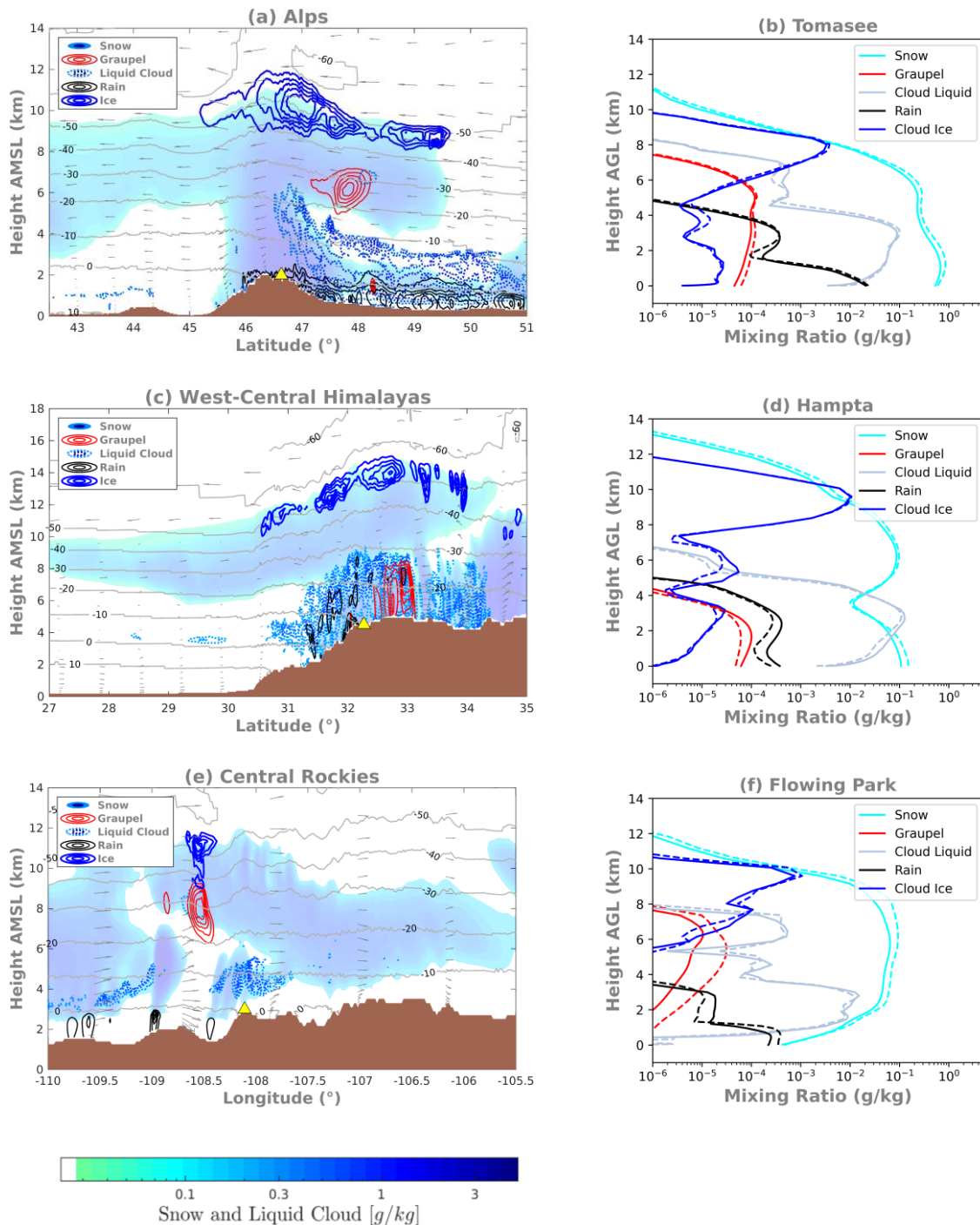
Fig. 9: Latitude-height transects of modelled hydrometeor mixing ratios ( \text{g kg}^{-1} ) through (a) Tomasee at 18 UTC 13 Jan 2019, (c) Hampta at 18 UTC 04 Jan 2022, and (e) Longitude-height transect of modelled hydrometeor mixing ratios ( \text{g kg}^{-1} ) through Flowing Park at 06 UTC 02 Feb 2024. The outputs are from the EXP simulation, and includes snow, graupel, liquid cloud, rain, and ice hydrometeors. Note that snow (filled
