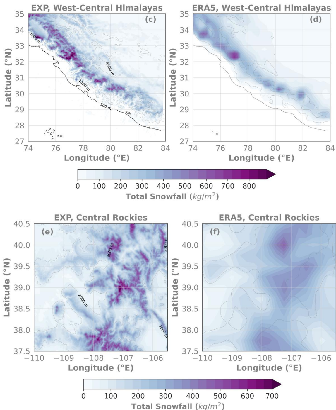
Fig. 10: Comparison of modelled and ERA5 total seasonal accumulated snowfall ( \text{kg m}^{-2} ) for the winter period of 2023-2024 for the (a,b) Alps and (e,f) central Rockies, and 2021-2022 for the (c-d) west-central Himalayas. The modelled outputs are from the EXP simulations. Also shown are the model orography (m; contours). Note that the snowfall for each region has a different scale.
