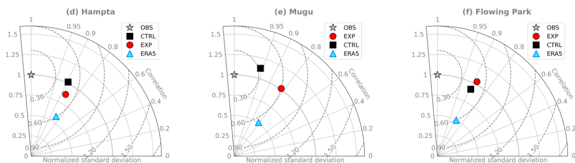
Fig. 4: Taylor diagrams of observed versus modelled snowfall at (a) Tomasee, (b) Rofental, (c) Ghepan, (d) Hampta, (e) Mugu, and (f) Flowing Park. The modelled outputs are from the CTRL (black) and EXP (red) simulations. Equivalent snowfall results from ERA5 are also shown (cyan). Radial distance indicates the normalised standard deviation (variability), azimuthal sectors represent the correlation coefficient, and concentric dashed contours centred on OBS denote the root mean square error (RMSE; \text{kg m}^{-2} ).
