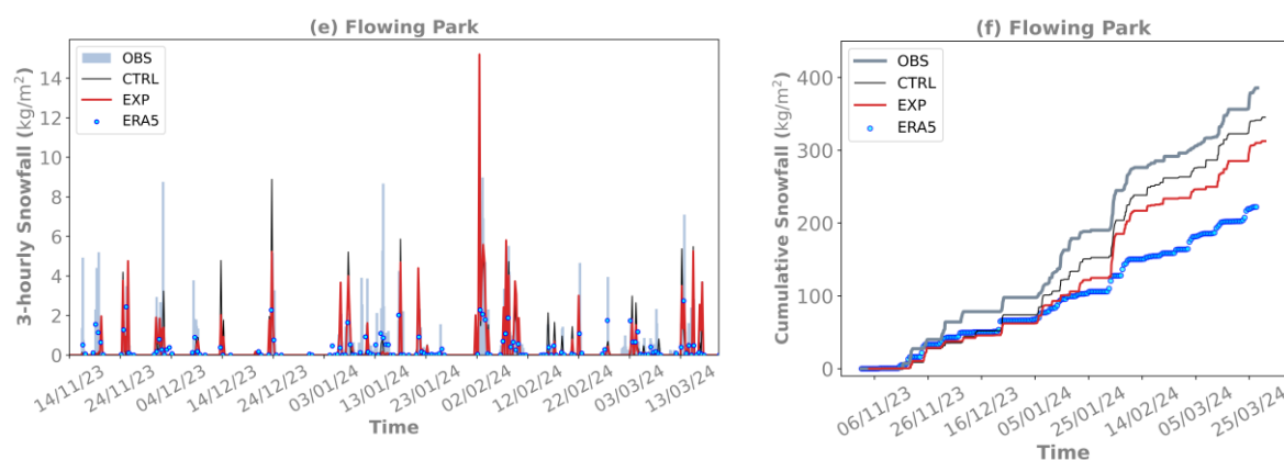
Fig. 6: Time series of observed and modelled (a,c,e) 3-hourly and (b,d,f) seasonal cumulative snowfall ( \text{kg m}^{-2} ) at (a,b) Tomasee, (c,d) Hampta and (e,f) Flowing Park. The modelled outputs are from the CTRL (black) and EXP (red) simulations. The results for Tomasee are for the period 01 Jan 2019 to 20 Mar 2019, Hampta for 02 Nov 2021 to 14 Mar 2022, and Flowing Park for 02 Nov 2023 to 01 Apr 2024. Equivalent snowfall totals from ERA5 are also shown (cyan).
