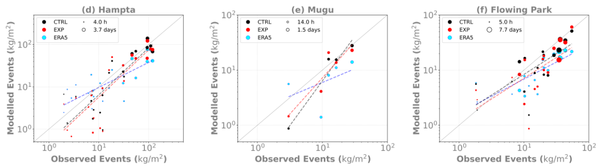
Fig. 2: Scatterplots of observed versus modelled snowfall totals ( \text{kg m}^{-2} ) for all events at (a) Tomasee, (b) Rofental, (c) Ghepan, (d) Hampta, (e) Mugu, and (f) Flowing Park. The modelled outputs are from the CTRL (black) and EXP (red) simulations. Equivalent snowfall totals from ERA5 are also shown (cyan). Event durations are estimated from the observed lake water pressure data at a temporal resolution of 10 mins and are represented by the size of the filled circles, with the range of durations varying by location, indicated by the smallest and largest circles for each site. The number of snowfall events for each location is listed in Table 1. Events are identified only if total snowfall amount exceeds 1 \text{ kg m}^{-2} for each event. The dashed lines represent lines of best fit.
