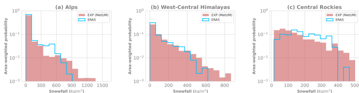
Fig. 11: Histograms of modelled and ERA5 total seasonal accumulated snowfall ( \text{kg m}^{-2} ) for the winter period of 2023–2024 for the (a) Alps and (c) central Rockies, and 2021–2022 for the (b) west-central Himalayas. The modelled outputs are from the EXP simulations upscaled to the ERA5 resolution of 0.25^\circ .
