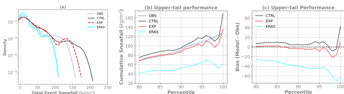
Fig. 5: (a) Comparison of density functions of observed and modelled snowfall (b) Upper-tail percentiles (80 th - 100 th ) of cumulative snowfall ( \text{kg m}^{-2} ) for observed and modelled snowfall events (c) Upper-tail bias between observed and modelled snowfall events. Modelled outputs are from the CTRL (black) and EXP (red) simulations. Equivalent snowfall from ERA5 is also shown (cyan).
