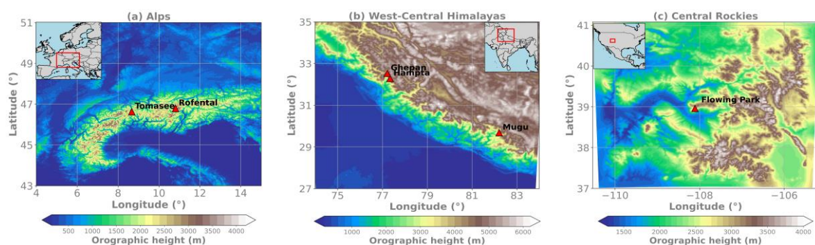
Fig. 1: Maps showing MetUM model domains and orography (m; shading) at 1.5 km grid spacing for the (a) Alps, (b) west-central Himalayas, and (c) central Rockies, with the positions of the lake-based snowfall measurement sites indicated by red triangles. Note that the orography in each of the panels have different ranges.
