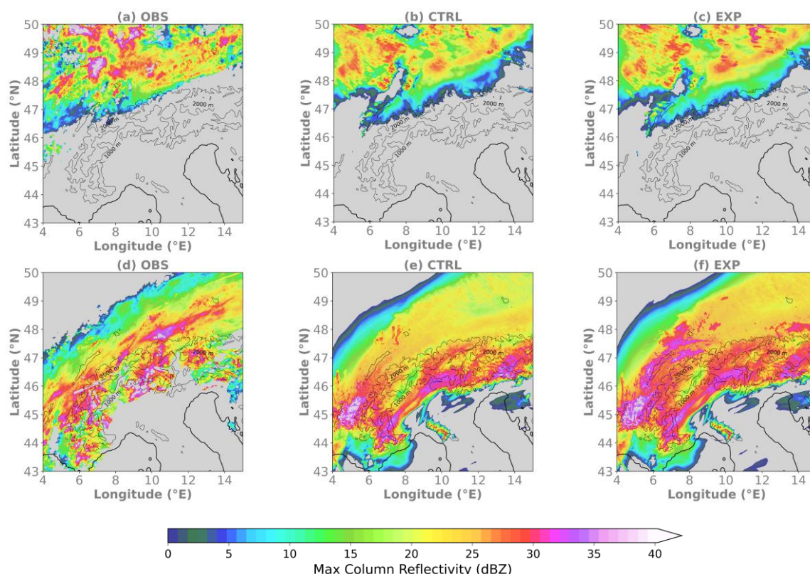
Fig. 7: Comparison of observed and modelled maximum radar reflectivity (dBZ; shading) for the Alps on (a-c) 18 UTC 12 Jan 2019 and (d-f) 18 UTC 01 Dec 2023. The modelled outputs are from the CTRL and EXP simulations. Also shown are the model orography (m; contours).
