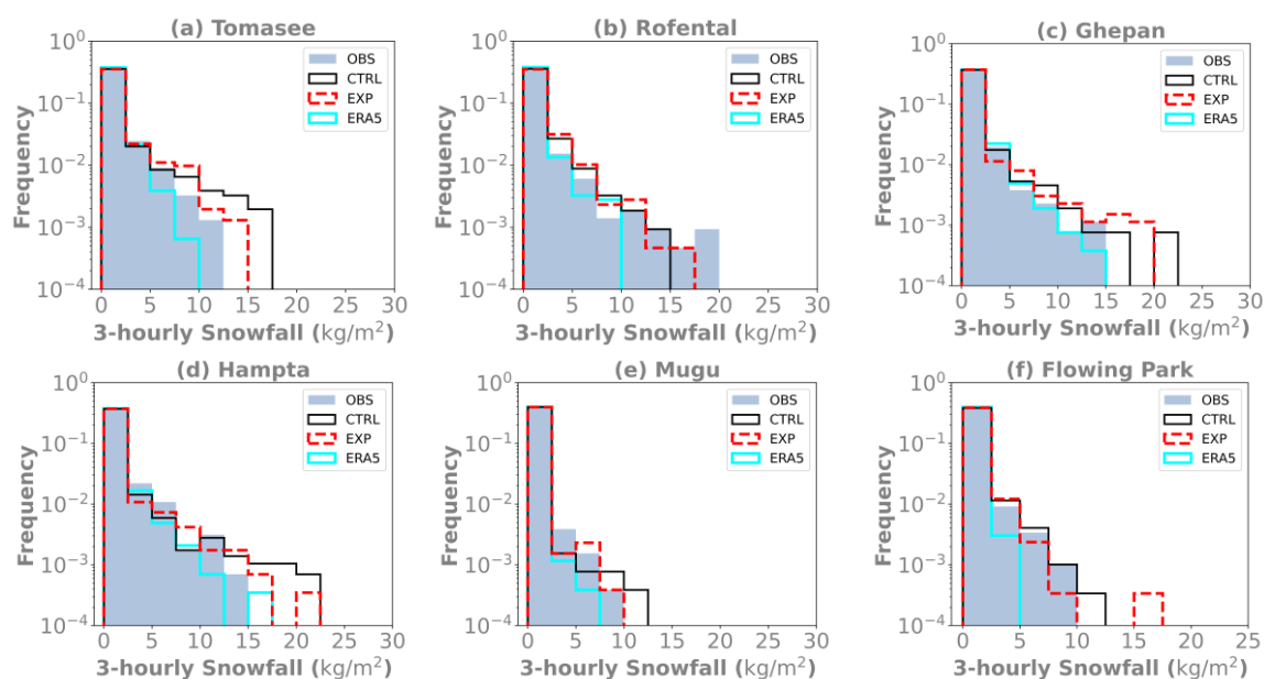
Fig. 3: Histograms of observed and modelled 3-hourly accumulated snowfall ( \text{kg m}^{-2} ) for all events at (a) Tomasee, (b) Rofental, (c) Ghepan, (d) Hampta, (e) Mugu, and (f) Flowing Park. The modelled outputs are from the CTRL (black) and EXP (red) simulations. Equivalent snowfall totals from ERA5 are also shown (cyan).
