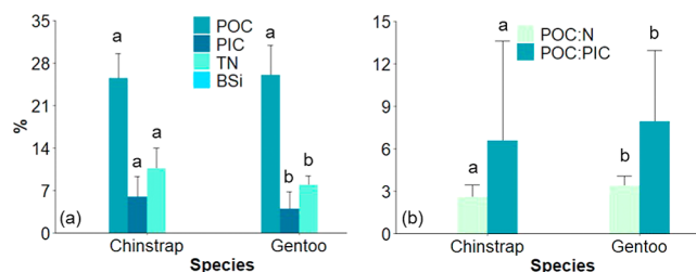
Figure 3. (a) Chemical particulate characterization expressed as % of their dry mass) of POC, PIC, TN, and BSi and (b) expressed as POC:N and POC:PIC ratios of Chinstrap and Gentoo penguin guano collected off the Antarctic Peninsula during the austral summers 2020/2021 and 2021/2022. Different letters indicate significant differences ( p < 0.05 ) between the two species.
