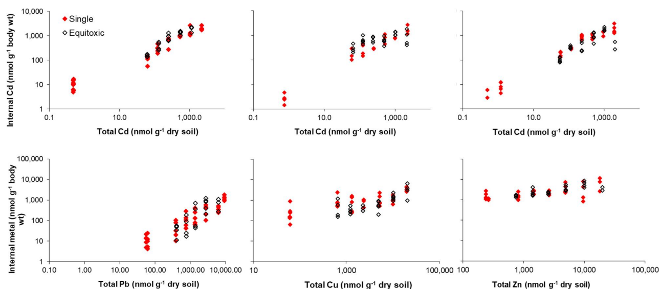
Figure 2 Concentrations of cadmium (top) and lead, copper, or (bottom) in Folsomia candida after 4 weeks exposure in LUFA 2.2 soil to binary mixtures of Cd with Pb (left), Cu (middle), and Zn (right), related to total soil concentrations. Results are presented for animals exposed to individual metals (Single) or to equitoxic mixtures (Equitoxic).
