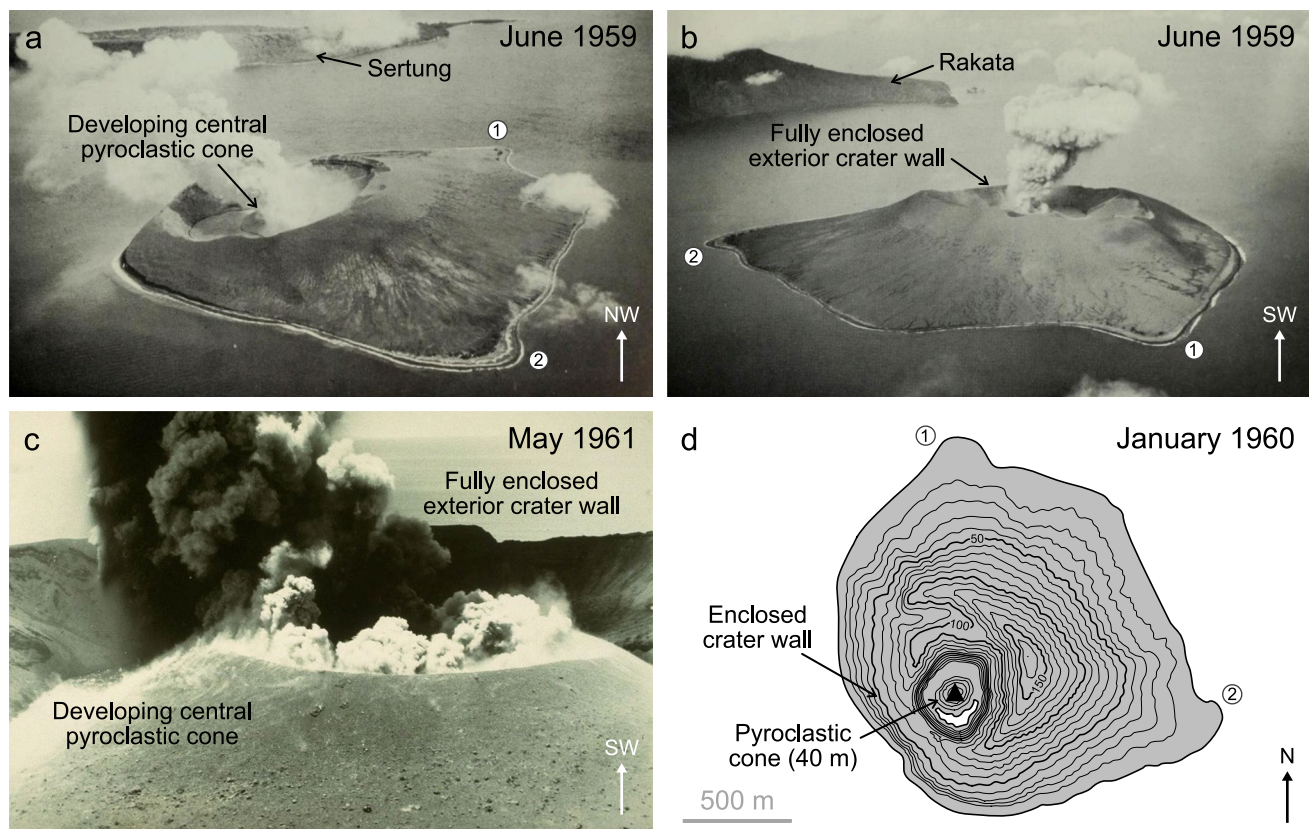
Fig. 7 End stage 2 to early stage 3: a and b Aerial photographs of Anak Krakatau in June 1959 showing the fully enclosed exterior crater wall and a small central pyroclastic cone (~25 m high) (Furneaux 1964). c Activity at the newly constructed pyroclastic cone (height
