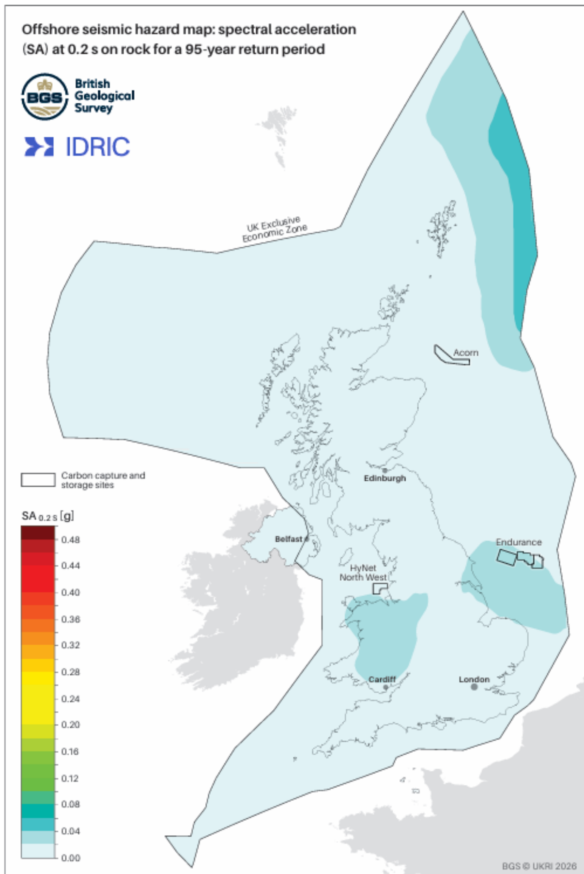
Figure 13 Hazard map for SA_{0.2 s} for a 95-year return period. The large, black polygon describes the UK offshore EEZ. BGS © UKRI 2026. Contains OS data © Crown copyright and database right 2026.
