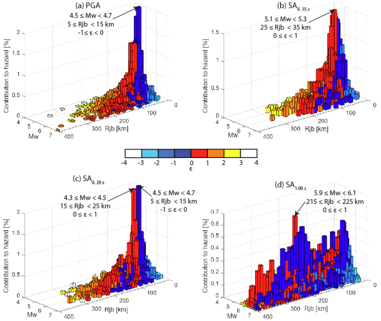
Figure 28 Disaggregation of the hazard for the Dover site and 2475-year return period by magnitude ( M_w ), Joyner-Boore distance ( R_{jb} ) and epsilon ( \epsilon ) for (a) PGA, (b) SA_{0.15s} , (c) SA_{0.20s} , and (d) SA_{1.00s} .
