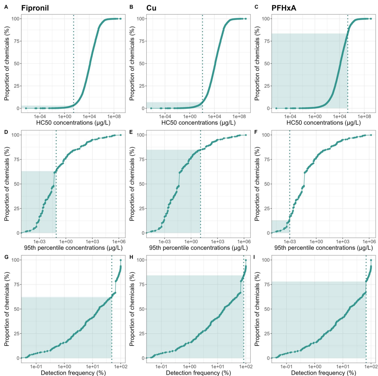
Figure 2 (A–C) Frequency distribution of HC_{50} values from acute EC_{50} toxicity data for aquatic species for all chemicals in the species sensitivity distribution database of Posthuma, van Gils, et al. (2019). (D–F) Frequency distribution of 95th percentile exposure concentrations and (G–I) frequency distribution of detection frequency for fipronil, copper (Cu), and perfluorohexanoic acid (PFHxA). The dashed line in each plot indicates where the HC_{50} , 95th percentile concentration, or detection frequency for each chemical falls relative to the value for all other chemicals. EC_{50} = half maximal effective concentration; HC_{50} = hazardous concentration for 50% of species.
