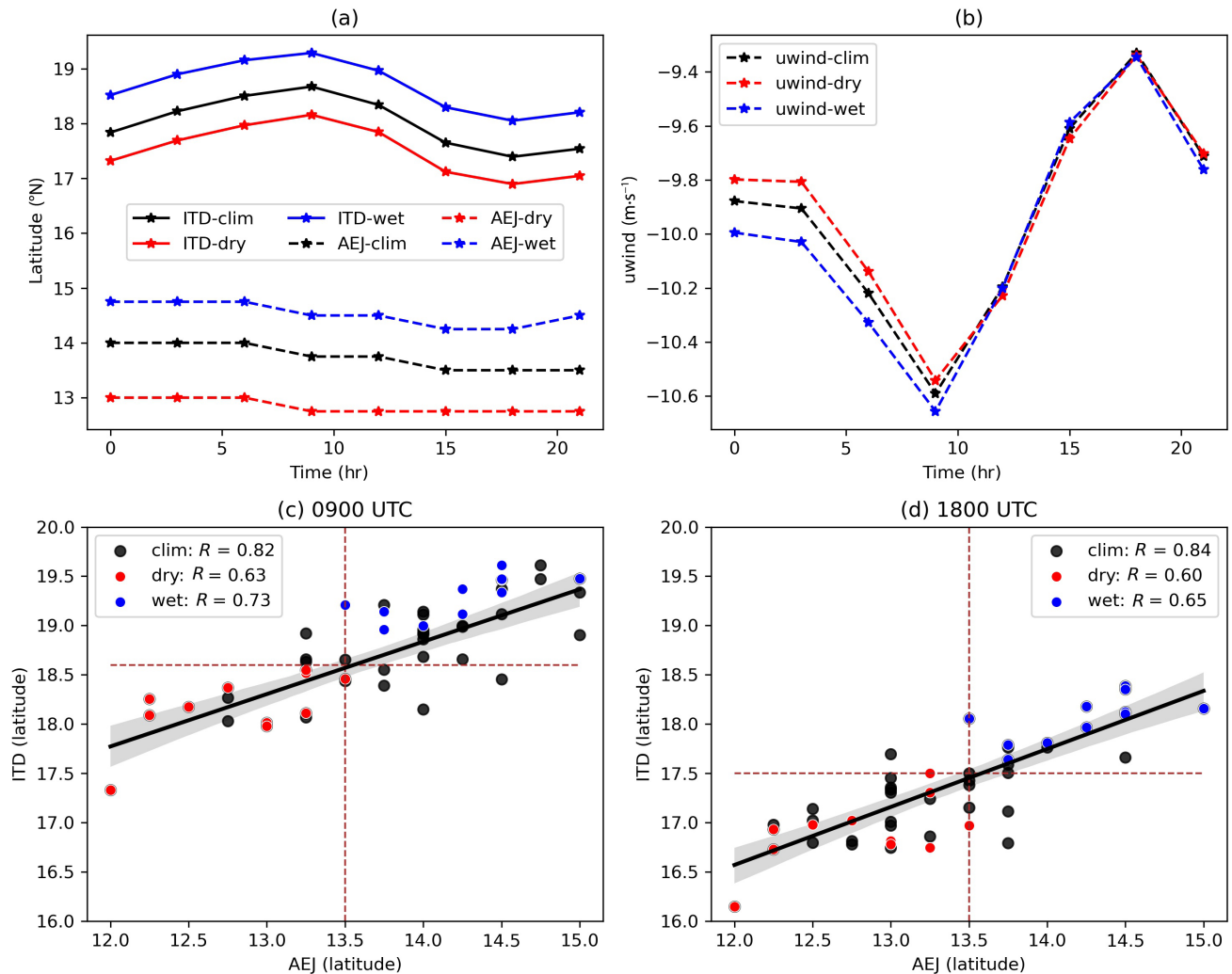
FIGURE 2 Zonally averaged (15°W to 10°E) diurnal (three-hourly) cycle for the climatology (clim) and wet and dry years, showing the (a) meridional variability of the intertropical discontinuity (ITD) and African easterly jet (AEJ), and (b) average of u -wind at 700–500 mb corresponding to the AEJ level. Regression of the ITD and AEJ at the times of (c) maximum (0900 UTC) and (d) minimum (1800 UTC) meridional limit using the Pearson correlation method. All coefficients are significant at P \leq 0.05 . Dashed vertical lines separate the ITD–AEJ under wet and dry regimes.
