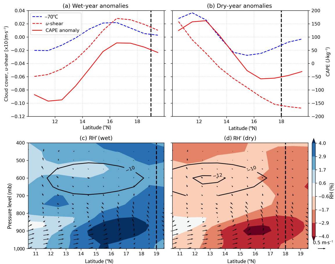
FIGURE 8 Meridional anomalies in -70^\circ\text{C} mesoscale convective system, convective available potential energy (CAPE), and shear for (a) wet and (b) dry years. (c, d) Anomalies in the surface to mid-tropospheric relative humidity (RH) in the (c) wet and (d) dry years. The lines of wind vectors, intertropical discontinuity, and African easterly jet are same as in Figure 7.
