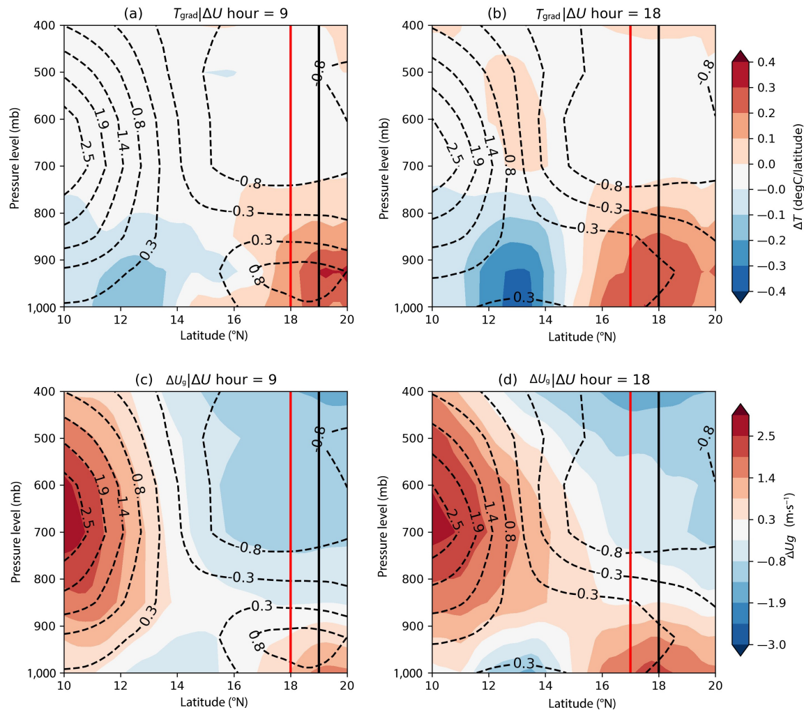
FIGURE 4 As Figure 3, but showing temperature gradient and zonal winds at (a) 0900 UTC and (b) 1800 UTC and (c, d) geostrophic wind at same times. The vertical solid vertical lines represent the location of the intertropical discontinuity for wet (black) and dry (years).
