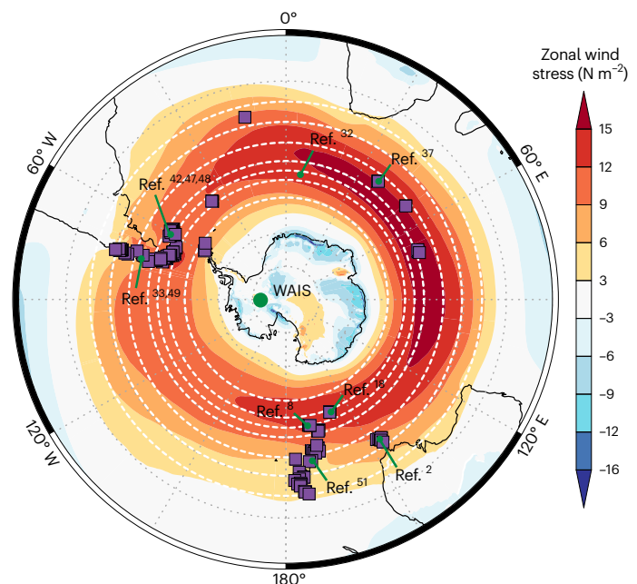
Fig. 1 | Zonal winds and study site locations. Zonal wind stress at 850 hPa (averaged 2015–2020) from European Reanalysis ERA5 64 , with the locations of basal peat sites indicated by purple squares (not all sites are distinguishable due to overlap). White dashed lines indicate the latitudinal boundaries (35° S, 40° S, 45° S, 50° S, 52.5° S, 55° S and 60° S). The locations of selected proxy records discussed in the text are indicated by the green circles: Anderson et al. 32 ; Nel et al. 37 ; Saunders et al. 18 ; Fletcher et al. 2 ; McGlone et al. 8 ; Tielidze et al. 51 ; Davies et al. 33 ; Moreno et al. 49 ; Monteath et al. 42 ; Spoth et al. 48 ; Scaife et al. 47 ; WAIS; West Antarctic Ice Sheet Divide Core 65 .
