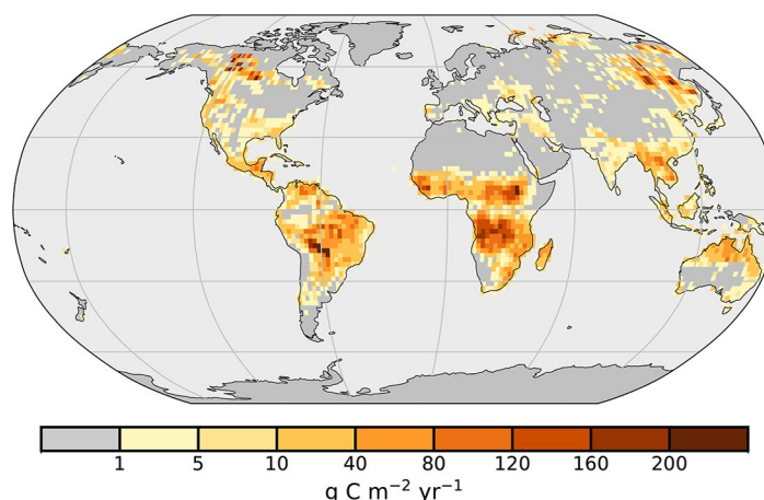
Fig. 2.87. Global map of fire activity in 2024 in terms of carbon consumption (g C m -2 yr -1 ). (Source: Copernicus Atmosphere Monitoring Service Global Fire Assimilation System version 1.4 [CAM5-GFASv1.4].)
