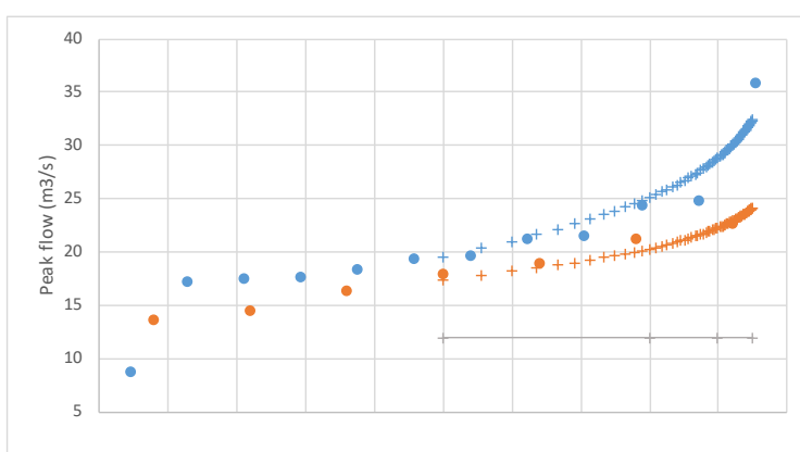
Figure 9 - a Generalised Extreme Value distribution (+) is fitted to observed annual maxima (●) plotted using Gringorten plotting positions for each site. Blue: pre-2013, orange: post-2013. Given the short record lengths, uncertainties are large.
