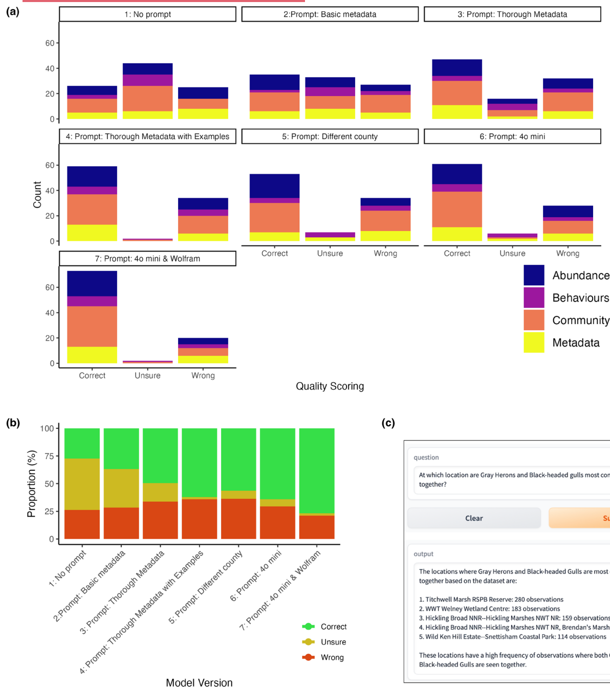
FIGURE 2 Evaluation of different prompts attached to a LangChain SQL agent. (a) The counts of correct, unsure and incorrect answers generated by the different models, coloured by the different ecological query categories. (b) The changing proportion of correct:unsure:incorrect over time as the model was iteratively improved. (c) A correct user query and model-generated answer from the final version of the model, visualised in a Gradio UI.
