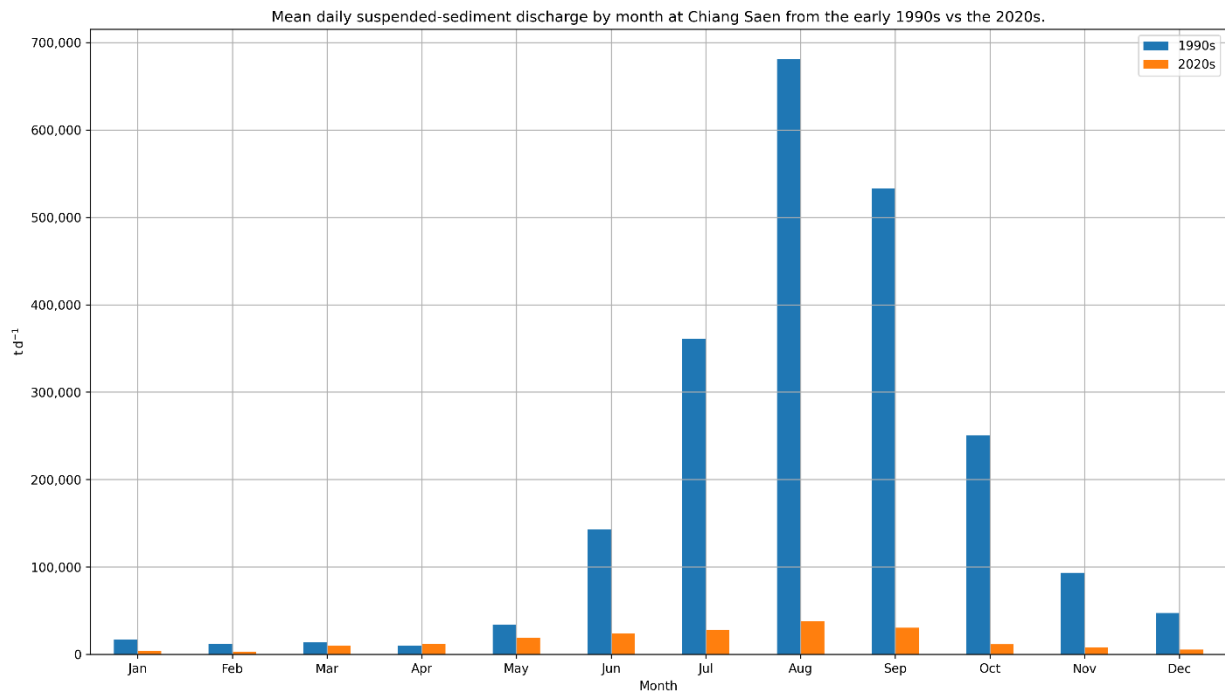
Figure 5. Suspended sediment discharge data from Chiang Saen, Chiang Rai Province, northern Thailand.
