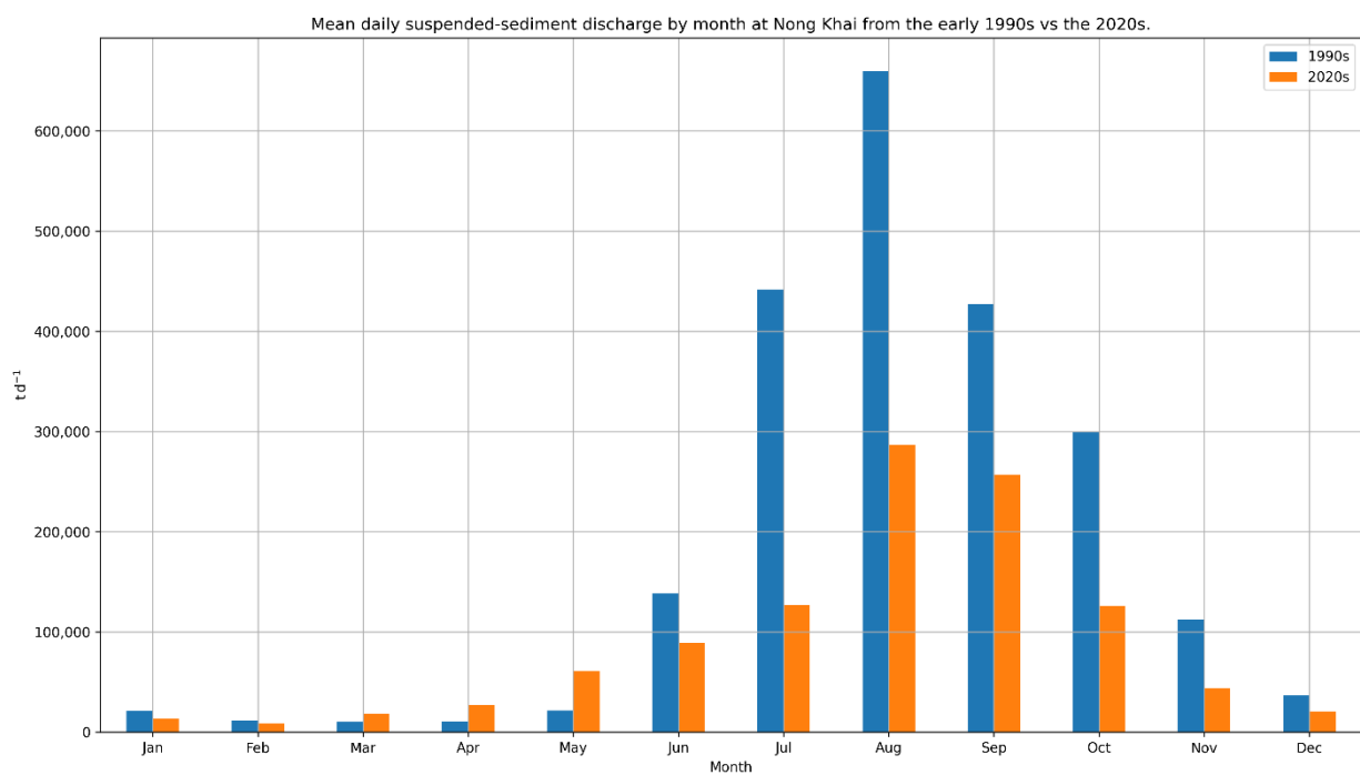
Figure 6. Suspended sediment discharge data from Nong Khai, Nong Khai Province, northeastern Thailand.
