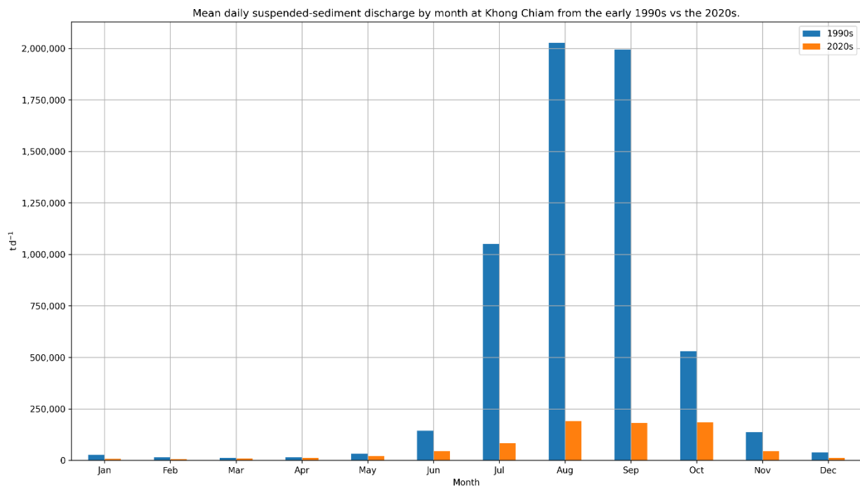
Figure 7. Suspended sediment discharge data from Khong Chiam, Ubon Ratchathani Province, northeastern Thailand.
