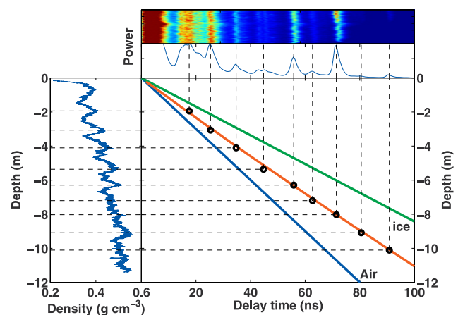
Figure 2. The relationship between ASIRAS radar power return and the snow/firn density profile from the neutron-scattering probe. (left) The density profile at site T 21 on the EGIG line. The prominent peaks in density are interpreted as annual winter horizons. (top) The power return in the region of T 21. The power is presented as both a trace showing the mean of 30 adjacent traces, and a color plot showing approximately 1 km around T 21. (middle) Travel-time versus depth; to compare the radar return to the density profile, we calculate the wave speed in snow using a mixing model [Looyenga, 1965]. The expected depth-travel time curve, calculated with these density data, is shown by the red line, and depth-travel time curves calculated for solid ice and air are plotted as green and blue lines. Lines drawn from peaks in the density profile intersect with lines drawn from peaks in the power return at locations marked by the small circles. These locations fall along the expected depth-travel time curve, indicating that the peaks in the power return are associated with annual high density layers.
