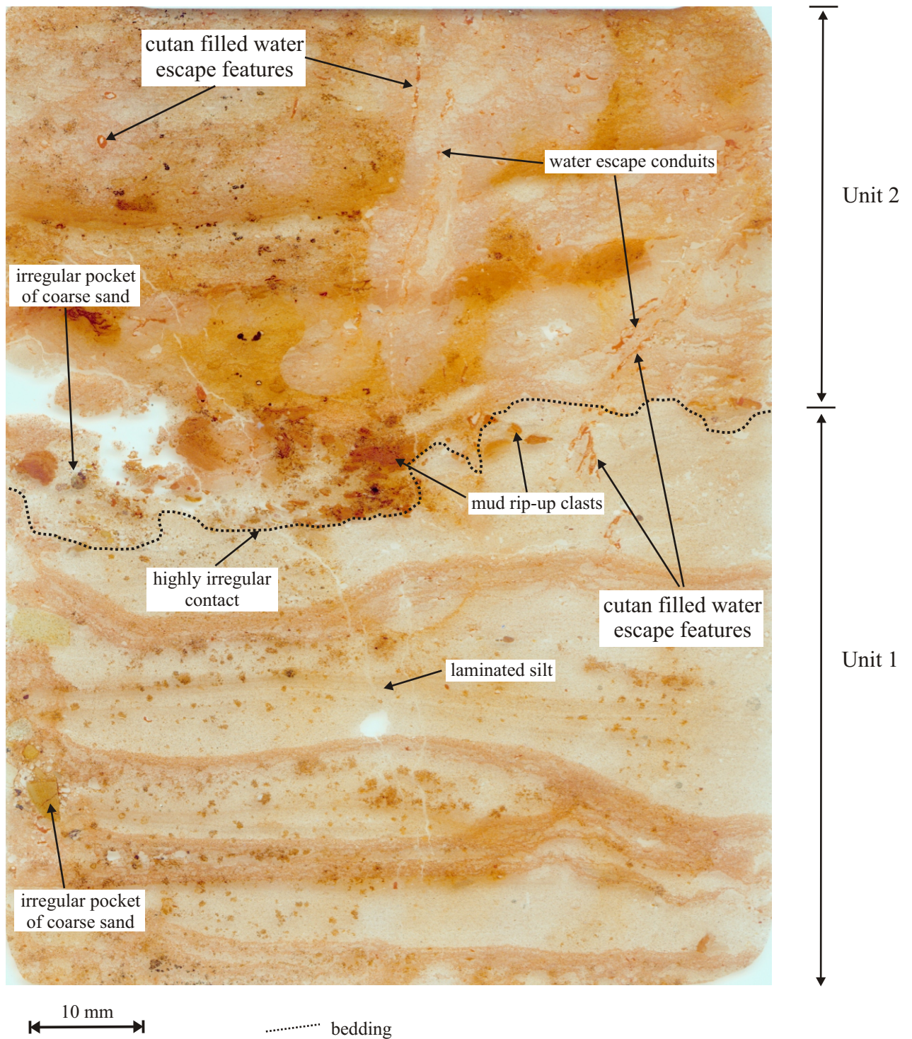
Fig. 8. Annotated scanned image of sample N2846.
