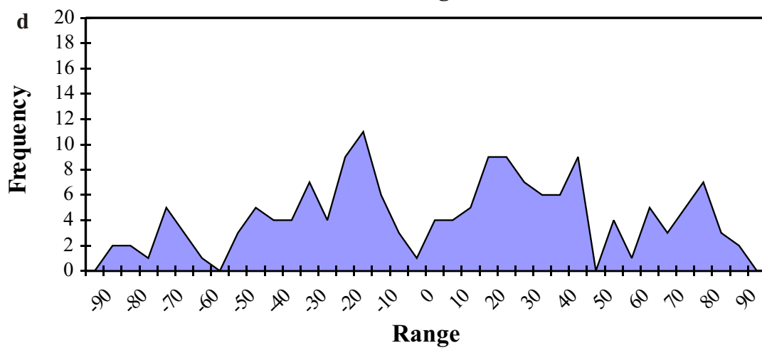
Fig. 15. Diagram showing clast orientation data for sample N2849. (a) plot of aspect ratio versus orientation of long axis. (b) histogram showing variation in clast aspect ratio. (c and d) plots
