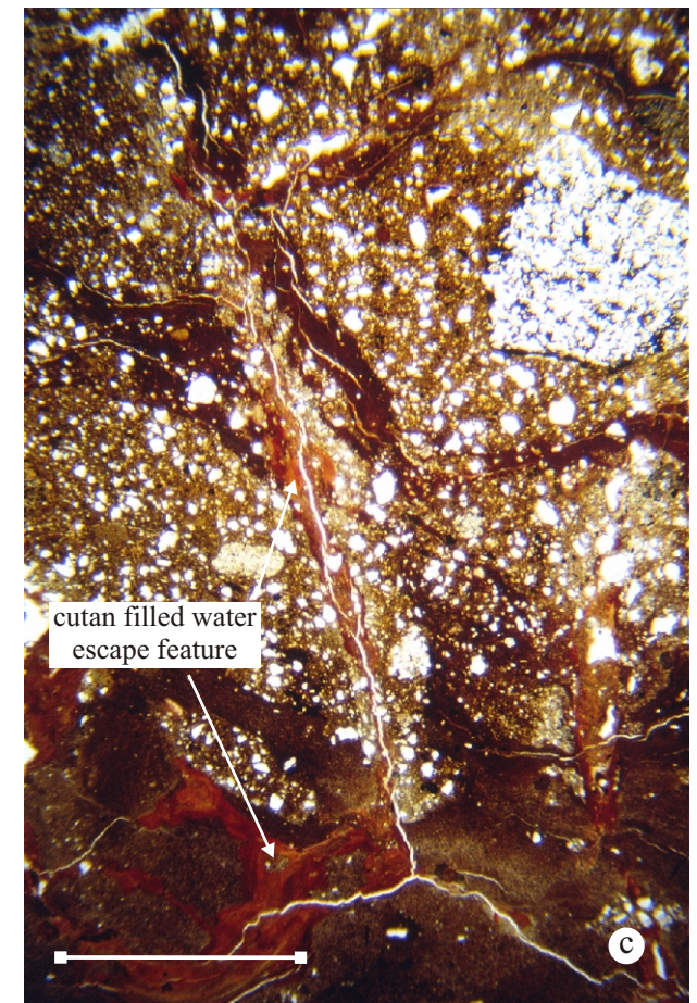
Plate 4. (a) Rounded to irregular till pebbles within a clay matrix (Sample N2842, plane polarised light, scale bar = 1 mm). (b) Rounded to irregular till pebbles within a clay matrix which possess a well developed plasmic fabric (Sample N2842, crossed polarised light, scale bar = 1 mm). (c) Lower magnification view of water escape conduit cross cutting diamicton layer rich in rounded till pebbles. Late-stage fluid flow concentrated into distinct pathways resulting in the deposition of orange-brown clay cutan (Sample N2842, plane polarised light, scale bar = 4 mm).
