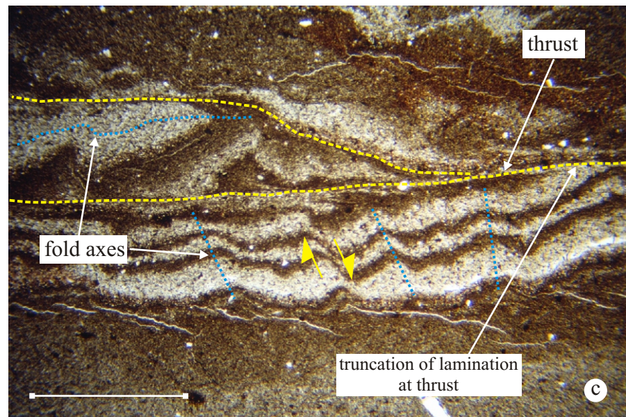
Plate 1. (a) Recumbent fold deforming laminated silt and clay. Overturned limb of fold is truncated by a small-scale thrust fault (Sample N2840, plane polarised light, scale bar = 4 mm). (b) Recumbent, rootless fold deforming silt within partially fluidised silt and clay (Sample N2840, plane polarised light, scale bar = 4 mm). (c) Disrupted laminated silt and clay deformed by small-scale crenulation-style folds and thrust faults (Sample N2840, plane polarised light, scale bar = 4 mm).
