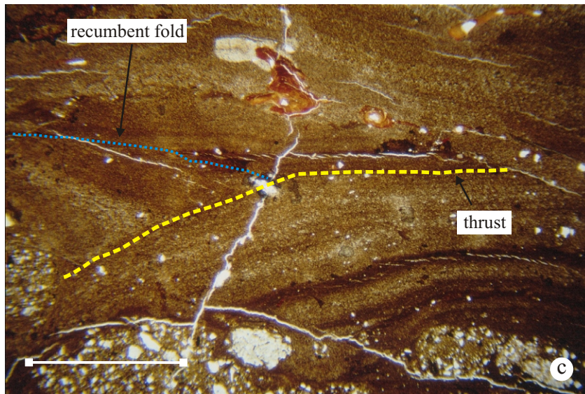
Plate 6. (a) Rounded to irregular till pebbles within a clay matrix (Sample N2842, plane polarised light, scale bar = 1 mm). (b) Rounded to irregular till pebbles within a clay matrix which possess a well developed plasmic fabric (Sample N2842, crossed polarised light, scale bar = 1 mm). (c) recumbent fold structure in hanging wall of thrust fault deforming laminated clay and silt (Sample N2842, plane polarised light, scale bar = 1 mm).
