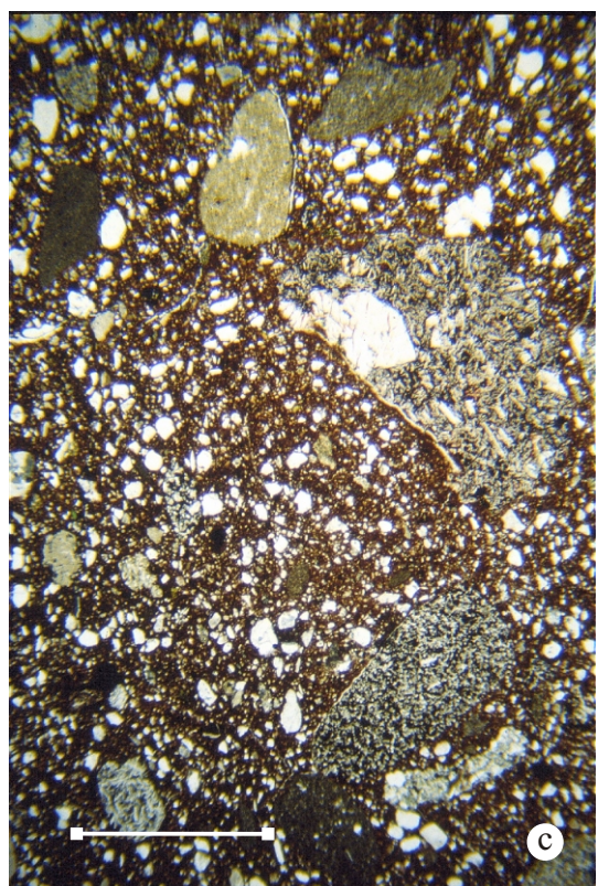
Plate 10. (a) patch of fluidised sand cross cutting laminated silt resulting in localised disruption of bedding (Sample N2846, plane polarised light, scale bar = 4 mm). (b) clay cutan filling late-stage water escape features (Sample N2846, plane polarised light, scale bar = 4 mm). (c) poorly sorted clast-rich diamicton (Sample N2848, plane polarised light, scale bar = 4 mm). (d) rounded bioclastic limestone clast in diamicton (Sample N2848, plane polarised light, scale bar = 4 mm).
