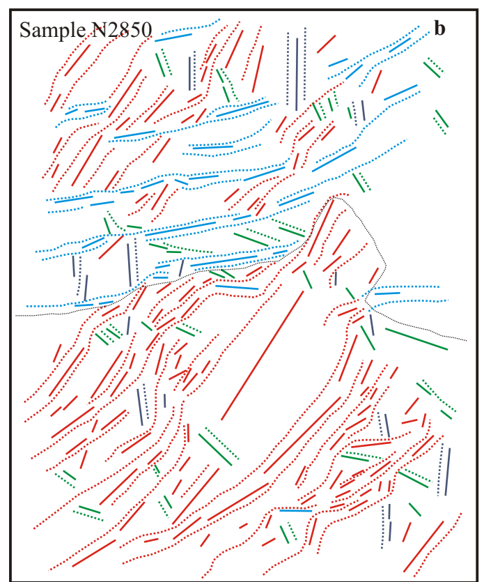
Fig. 21. (a) Diagram showing the orientation of the long and short axes of coarse sand to pebble sized clasts within sample N2850. (b) Interpreted pattern of long axis orientation within sample N2850.
