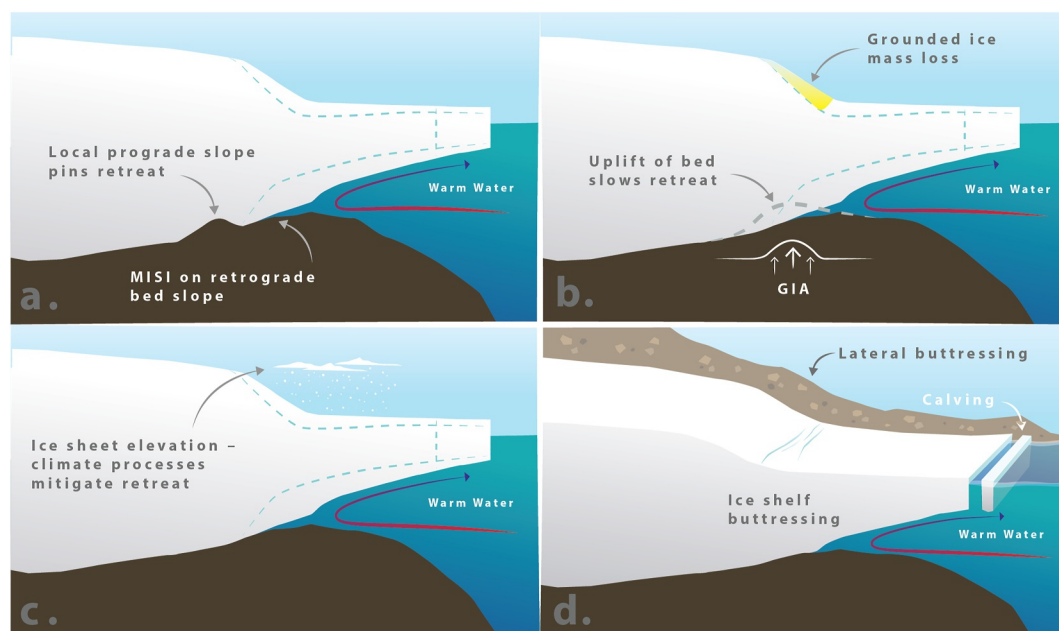
Figure 12. Hypothesized mechanisms that impact the stability of a marine-ice-sheet grounding line on a retrograde bed slope (i.e., marine ice sheet instability (MISI)-prone grounding line) under the influence of a warming ocean. In each panel, the solid strokes outline the ice-sheet geometry today and the dashed strokes outline the ice sheet geometry in the future. (a) Retreat onto significant topography can temporarily or permanently prevent MISI, depending on changes in climate forcing. (b) Solid-earth uplift in response to ice mass unloading (i.e., glacial isostatic adjustment) can slow (or even prevent) grounding line retreat. (c) Ice-atmosphere interactions, including the dependence of surface mass balance and surface melt on the ice surface elevation and temperature can stabilize the grounding line on a retrograde bed. (d) Where a marine ice sheet is in an embayment, a grounding line lying on a retrograde bed may be stable or unstable, depending on lateral buttressing and boundary conditions, including calving.
