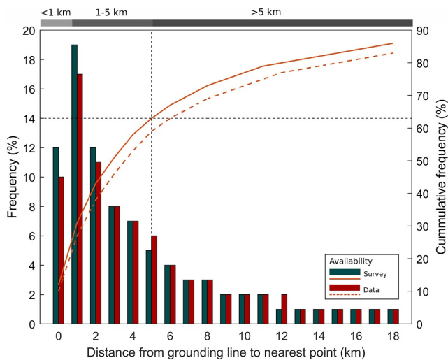
Figure 20. Histograms showing the ice-penetrating radar survey and bed-elevation data availabilities in the vicinity of the RINGS/Bedmap3 grounding line. Abscissa show the distance from the grounding line to the closest survey or data points. Both cases analyzed data with precise locations collected with GPS or GNSS since 1990s. Survey availability analyzed using both classes 2 and 3; the class 2 indicates locations where the bed echo is not identified though the survey is made, whereas the class 3 indicates locations where the bed echo is successfully identified (Figures 14b and 19, and Section 4.3). Data availability analyzed using only the class 3.
