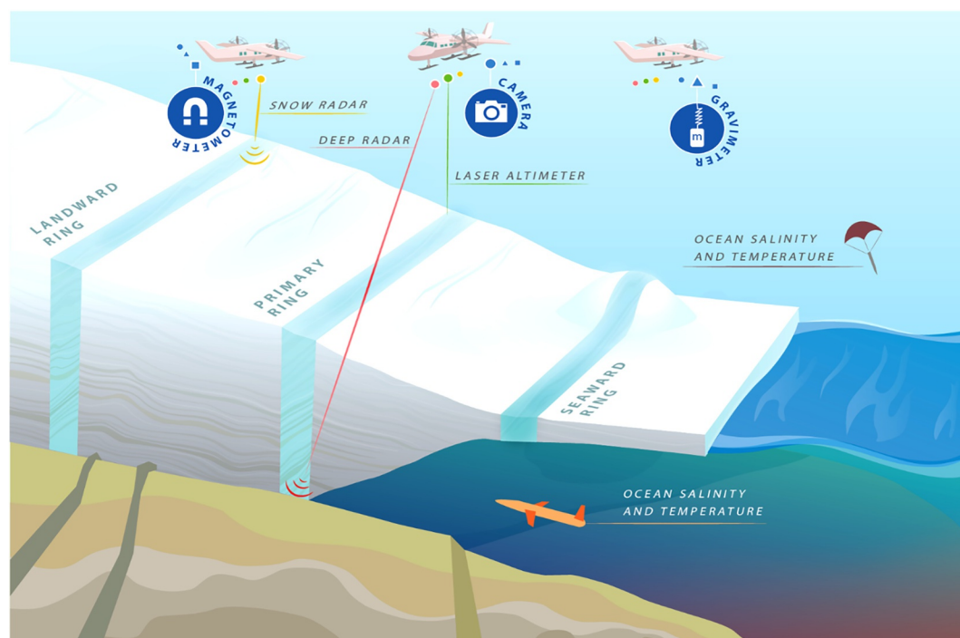
Figure 13. Schematic of airborne surveys targeting the coastal zone of Antarctica, including ice-sheet terminus, the vicinity of the grounding zone, ice shelves, and open or sea-ice-covered ocean. Three profile locations in the coastal zone are here called landward ring, primary ring and seaward ring, to reflect the need of circum-Antarctic surveys (Section 5). All instruments are valuable for surveys at three rings locations; three airplanes illustrate different applications and priorities of these instruments.
