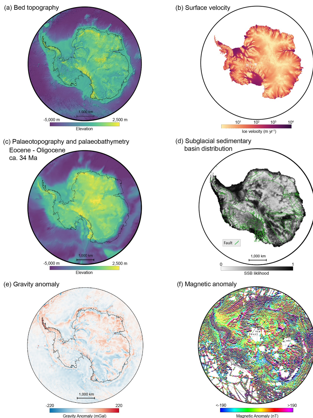
Figure 7. Overview of the Antarctic Ice Sheet. (a) Contemporary bed topography (Dorschel et al., 2022; Morlighem et al., 2020). (b) Ice-surface flow speed. (c) Modeled paleo bed topography when the AIS was initiated first time around 34 Million years ago (Ma) (Hochmuth et al., 2020; Paxman et al., 2019). To compare paleo and contemporary bed topography, plate rotation is removed. Such motion is approximately grid eastward in the past 34 Ma. The contemporary grounding line is outlined for geographical reference. (d) Subglacial sedimentary basin distribution likelihood (L. Li et al., 2022a) with major fault systems (Aitken et al., 2014; Cox et al., 2023; Tankersley et al., 2022). (e) Gravity anomaly (Scheinert et al., 2016). (f) Magnetic anomaly (Golynsky et al., 2018). White blanks represent large data gaps that cannot be interpolated from airborne surveys and satellite data.
