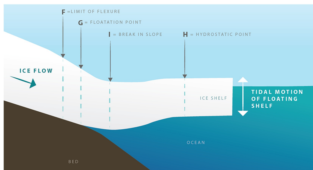
Figure 10. Elements of the grounding zone. The point F marks the limit of flexure (hinge line), G the point at which the ice begins to float (i.e., grounding line), I the break in ice surface slope, and H the point where ice is freely afloat. This figure is adapted from Fricker et al. (2002).
