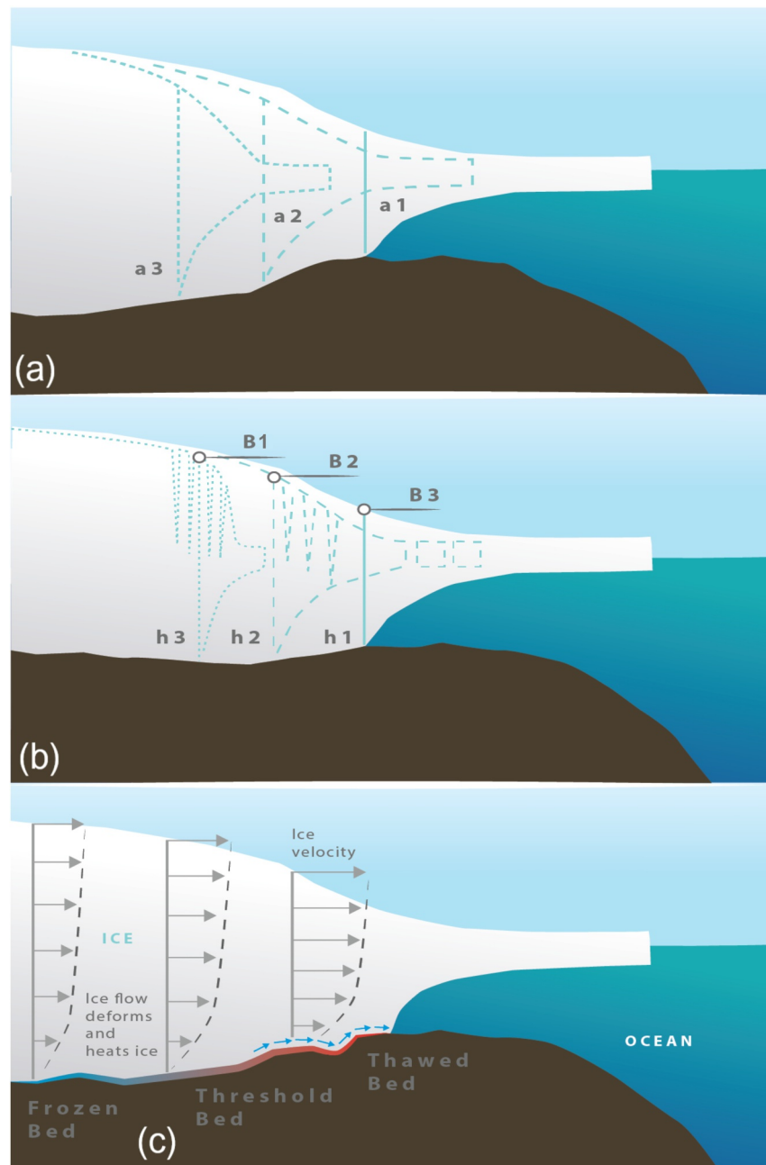
Figure 11. Three mechanisms of ice-sheet instability. The solid strokes in the all panels outline the ice-sheet geometry today and the dashed strokes in panels (a) and (b) outline the ice sheet geometry in the future. (a) Marine ice sheet instability (MISI) that can occur when the grounding line is located on a retrograde (inland lowering) slope of the bed under sea level. As the grounding line retreat, ice thickness increases so that the cross-sectional area a of the terminus to the ocean increases: a_3 > a_2 > a_1 . (b) The proposed marine ice cliff instability (MICI) that can occur regardless of the bed slope directions when the ice-sheet terminus is a very tall cliff which cannot be stabilized. As the terminus retreats, height h of the ice-sheet terminus above sea level becomes larger ( h_3 > h_2 > h_1 ), resulting in more readily calving and reduced buttressing B : B_3 < B_2 < B_1 . (c) Thermo-frictional feedback to melt the base of the ice sheet as flow speed increases toward the grounding line.
