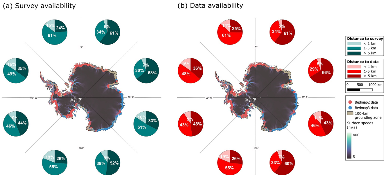
Figure 19. Overview of ice-penetrating radar survey availability (a) and bed-elevation data availability (b) across the Antarctic Ice Sheet in the coastal zone (marked right brown), within 100 km landward from the RINGS/Bedmap3 grounding line (Section 4.1). This analysis is based on the syntheses by Bedmap2 (Fretwell et al., 2013) and Bedmap3 (Frémand et al., 2023) data, but only using data with precise locations using GPS or GNSS since 1990s. Survey availability shows the reported survey locations regardless of the bed detection (class 2 and class 3 in Figure 14), whereas data availability shows only the survey with valid bed elevation data (class 3 in Figure 14). See full discussion of these classes in Section 4.3. It is usual that one survey profile includes both classes and missing bed echo at some locations. On the maps, the Bedmap2 data is overlaid on top of the Bedmap3 data. Background further inland shows surface flow speeds from the MEaSUREs data set (Rignot et al., 2017). For each 45-degree meridian, regional survey (a) and data (b) availabilities are shown.
