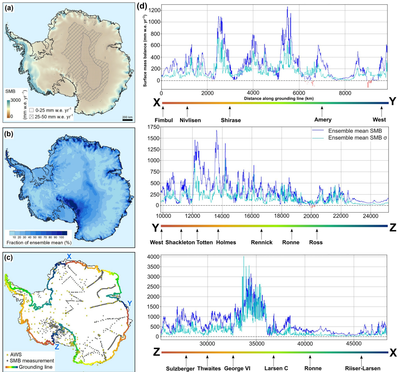
Figure 5. Modeled annual surface mass balance (SMB) averaged between 1987 and 2015, together with the locations of SMB observations and automatic weather stations (AWSs). (a) Ensemble mean of five model results (see Section 2.4.2 for all model names). (b) Ensemble standard deviation of these modeled SMB. These models have variable model-cell sizes (12.5–50 km) so all model results were interpolated to 12.5 km model cells (Mottram et al., 2021). (c) Locations of existing SMB data (gray dots) collected with snow stakes and firn/ice cores (Y. Wang et al., 2021). The location of AWSs are shown with yellow dots (Y. Wang et al., 2023). The color code along the grounding line gives a location reference for panels (d). (d) Ensemble mean (blue or red when negative) and standard deviation (green) of SMB at the grounding line. Note that the three panels are not scaled. The ends of these three profiles are shown with the letter X, Y, and Z and color bars indicate locations between these XYZ-labeled locations. Major ice shelves are labeled.
