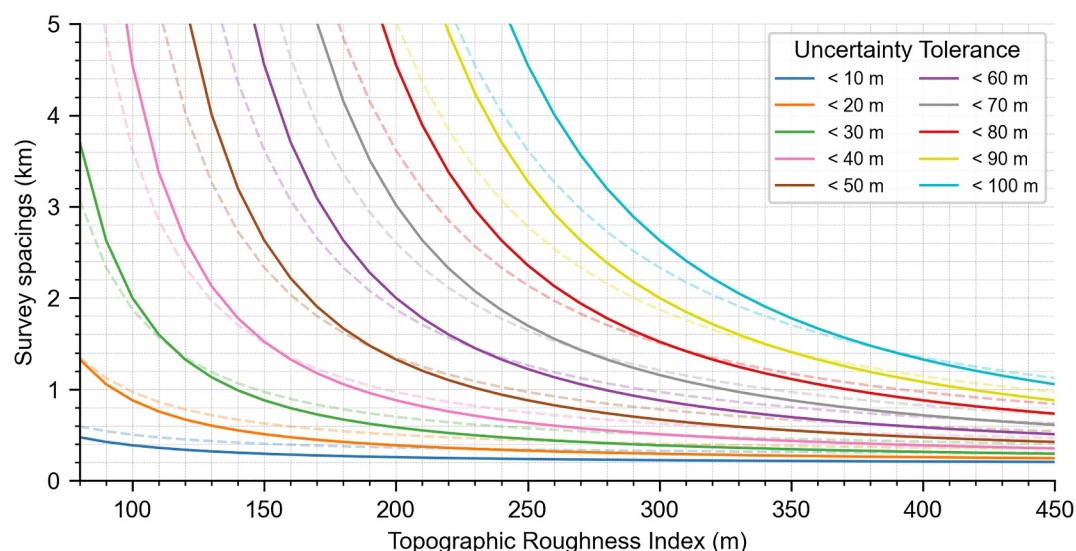
Figure 29. Survey spacings required to constrain bed elevation within various uncertainty tolerances, as a function of topographic roughness index, estimated using the parameterizations presented in Figure 28. Dashed curve shows this relationship derived near Dome Fuji, inland East Antarctic Ice Sheet (Shackleton et al., 2023).
