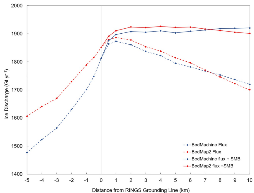
Figure 22. Ice discharge from the Antarctic Ice Sheet determined for flux gates that are stepwise migrated by 0.5 or 1 km on either side of the RINGS/Bedmap3 grounding line, excluding ice rises. Dashed lines show ice flux through a given flux gate, whereas solid lines on the landward side show estimated discharge at the grounding line after adding modeled surface mass balance (SMB) in the area between the grounding line and the flux gate. Blue lines are based on ice velocity from ITS_LIVE (Gardner et al., 2018) and ice thickness from Bedmachine version 3 (Morlighem et al., 2020), whereas red lines are based on ITS_LIVE and Bedmap2 (Fretwell et al., 2013). For SMB correction, we selected the ensemble model with median SMB from five regional climate model results (Mottram et al., 2021). The hydrostatic line is located 4.3 km seaward of the grounding line on average.
