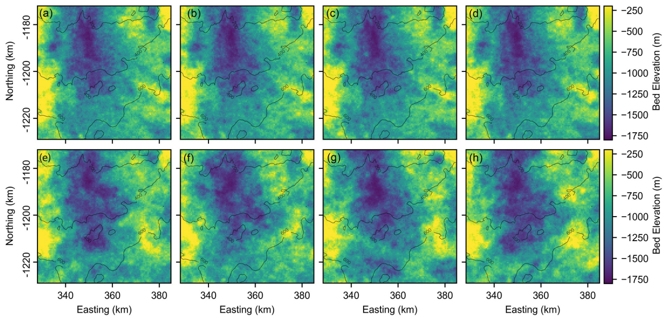
Figure 26. Stochastic simulations of bed topography in the vicinity of the Recovery Glacier outlet using 2.5-km spacing (upper row; panels a–d) and 10-km spacing (lower row; panels e–h) radar data. These radar profiles were acquired along grid east-west lines without any tie lines (Figure 27). The 10-km spacing data set was made by using every fourth profile in the original 2.5-km spacing data (Corr et al., 2021). Four columns correspond to four snapshots of simulations. Videos showing all 100 results are available (Shackleton & Matsuoka, 2025).
