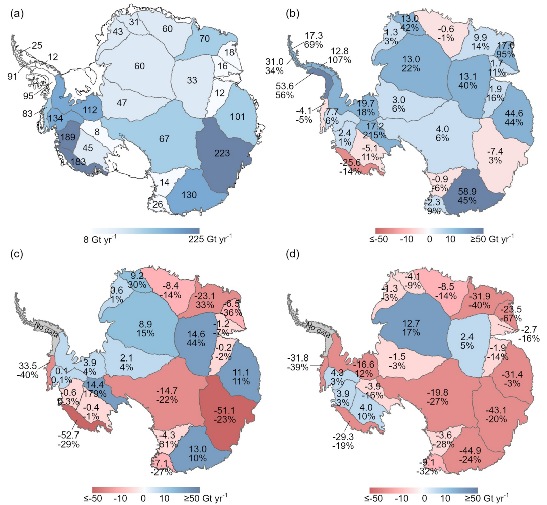
Figure 4. Comparison of recent ice-discharge estimates for 27 drainage basins of the Antarctic Ice Sheet (AIS). (a) Estimates for the year 2015 based on surface velocities from Landsat-8 across flux gates set close to available radar-data locations (Gardner et al., 2018). (b) Differences between Gardner et al. (2018) and Rignot et al. (2019) as excesses beyond the estimates by Gardner et al. (2018), both in values and fractions in percentage relative to Gardner et al. (2018). Rignot et al. (2019) provide time series of ice discharge based on measured surface velocity and estimated ice thickness at the grounding line, and year 2015 is reported as Supplementary Information for 68 basins which are here consolidated into the 27 basins defined by Zwally et al. (2002) and used by Gardner et al. (2018), although their boundaries do not exactly match. Panel (c) same as (b) but showing the differences between Gardner et al. (2018) and Miles et al. (2022) for the year 2015. (d) Differences between Rignot et al. (2019) and Miles et al. (2022) as excesses beyond the estimates by Rignot et al. (2019), both in values and fractions in percentage relative to Rignot et al. (2019) for the 18-year period between 1999 and 2017, the period that both studies cover. The values are converted to the unit of \text{Gt yr}^{-1} for comparison.
