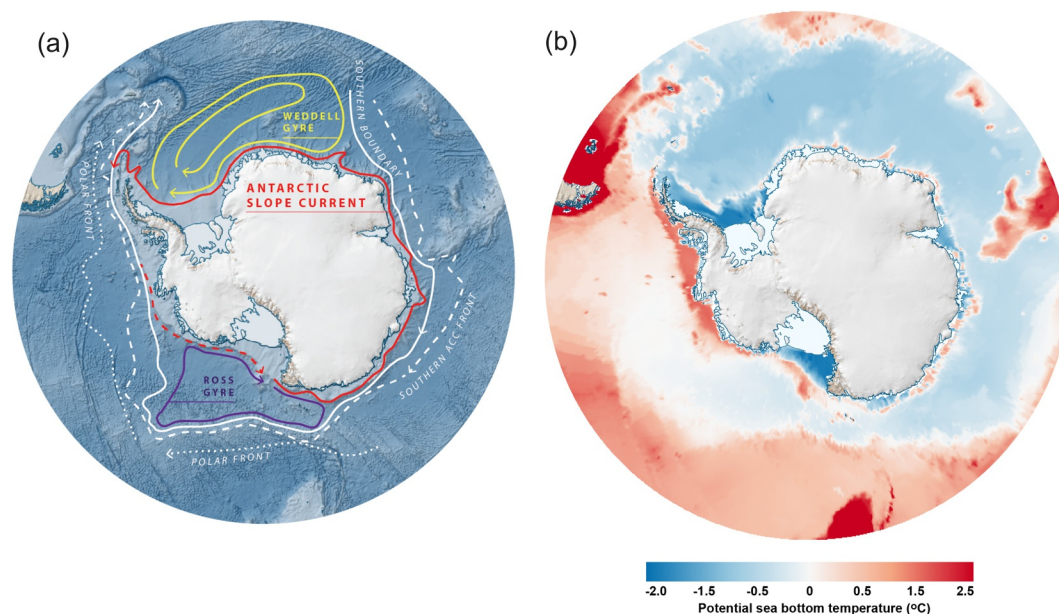
Figure 8. Southern Ocean circulation regimes and bottom temperature. (a) Circulation regime of the Antarctic margins. The Antarctic Slope Current (ASC, red) is depicted as a near-circumpolar, anticyclonic (westward) feature appearing at the shelf break in East Antarctica and the Weddell Sea. Uncertainty regarding the initiation of the ASC is indicated by the dashed line in the Bellingshausen and Amundsen Seas, as well as the western Ross Sea. Along the West Antarctic Peninsula, a slope current flows eastward, along with the southern boundary of the Antarctic Circumpolar Current (ACC). Interactions with the Weddell (yellow) and Ross (purple) Gyres (based on Armitage et al. (2018)), as well as the southern fronts of the ACC (white; based on Orsi et al. (1995)) are highlighted by their proximity to the ASC in various locations around the Antarctic margins (e.g., east of the Cosmonauts Sea). Also shown are sub-Antarctic Front and Polar Front. This figure is adapted from A. F. Thompson et al. (2018). (b) Ocean bottom temperatures around Antarctica based on the WOCE global hydrographic climatology (Noble et al., 2020). Note the existence of two primary regimes: a warmer sector in west Antarctica (the western Peninsula, Bellingshausen Sea, and Amundsen Seas, between 60°W and 120°W) and a colder sector around the rest of the continent. Continental Shelf edge is well visualized with the location of Antarctic slope current in panel (a). The basemap of these panels is made with Quantarctica (Matsuoka et al., 2021).
