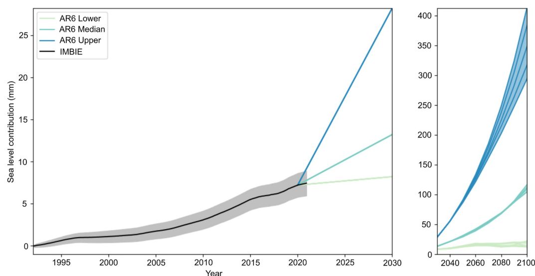
Figure 3. Comparison of observed Antarctic contributions to the sea level from 1993 to 2022 compiled by Ice Sheet Mass Balance Inter-Comparison Exercise (Otosaka et al., 2023) and modeled future Antarctic contributions compiled by the Intergovernmental Panel on Climate Change AR6 from 2020 to 2100 (Fox-Kemper et al., 2021). For observed data, the solid curve and gray shading show reconciled mean and standard deviation. For projections, lines show the 10th percentile (309–428 mm by 2100), median (103–115 mm), and 90th percentile (8–17 mm) of the projected Antarctic contributions for five emission scenarios: very low (SSP1–1.9), low (SSP1–2.6), intermediate (SSP2–4.5), high (SSP3–7.0), and very high (SSP5–8.5). Despite the difference between the emission scenarios, the 10th percentile, median and 90th percentile from all emission scenarios display three distinct clusters for each. This demonstrates that the primary source of projection uncertainty stems from the variability in the modeled physical systems of the Antarctic Ice Sheet (AIS) and our limited knowledge of the AIS, rather than from uncertainties related to emissions.
