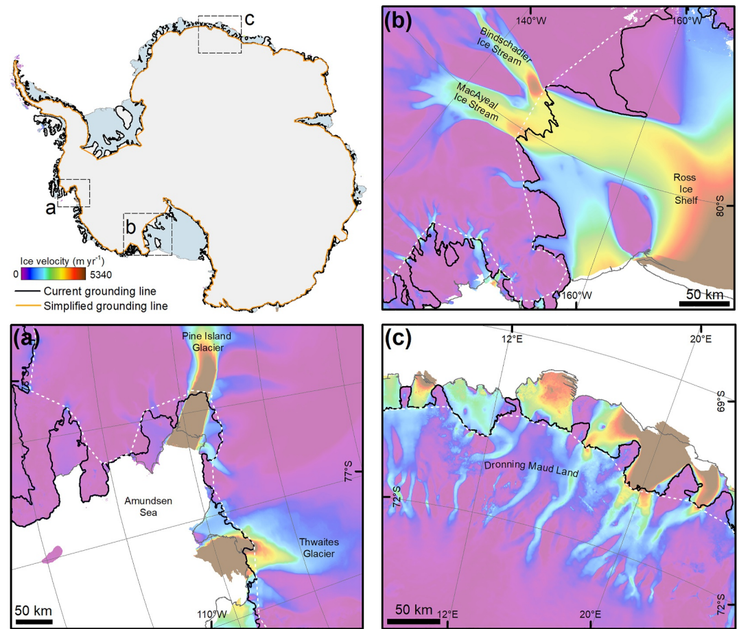
Figure 18. The proposed flux gate (primary ring) at the simplified grounding line of the Antarctic Ice Sheet (AIS) (orange, Section 4.1) and contemporary RINGS/Bedmap3 grounding line of the AIS (black, Section 4.2). RINGS/Bedmap3 grounding line is also defined for ice rises but not shown in this map. (a–c) Regional views of these grounding lines together with ice-flow speed (Gardner et al., 2018). Here, RINGS/Bedmap3 grounding line of the AIS is shown with black, whereas the simplified grounding line is shown with white dotted lines.
