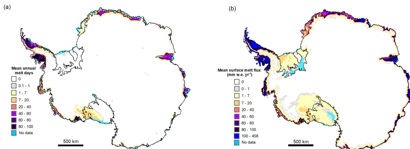
Figure 6. Mean annual melt days and melt flux derived from satellite data between 1979 and 2020. (a) Derived from passive microwave observations (Johnson et al., 2022). (b) Derived from microwave scatterometer (Trusel et al., 2013).
