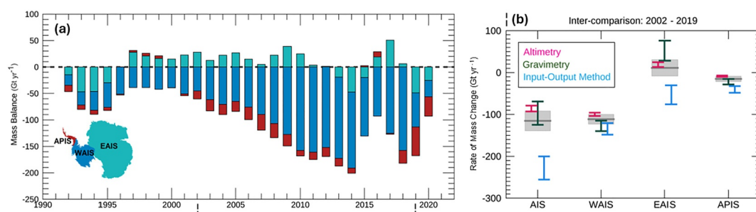
Figure 2. Recent mass balance of the Antarctic Ice Sheet in three regions of the West Antarctic Ice Sheet (WAIS), East Antarctic Ice Sheet (EAIS), and Antarctic Peninsula (AP) compiled by Ice Sheet Mass Balance Inter-Comparison Exercise (IMBIE, Otosaka et al., 2023). (a) Annual mass balance from 1992 to 2020. (b) Inter-comparison of the rate of mass change between 2002 and 2019 derived with the altimetry, gravity, and input-output methods. Gray line and box show IMBIE's reconciled value and uncertainty.
