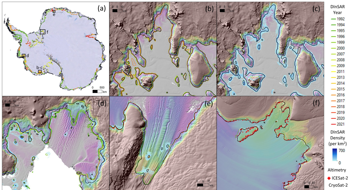
Figure 17. Grounding lines of the Antarctic Ice Sheet. The RINGS/Bedmap3 grounding line is shown with black curve in all panels together with various grounding line products. (a) Historic differential interferometric synthetic aperture radar (DInSAR) grounding line data colored by year (Floricioiu et al., 2021; Rignot et al., 2016). Background images are the LIMA, Landsat image mosaic of Antarctica (Bindschadler et al., 2008). The locations of (b–f) are indicated with black frames in (a). (b) Historic DInSAR data for the inner parts of the Sulzberger Ice Shelf. (c) Heatmap derived from the density of DInSAR grounding lines from Sentinel-2 data in 2018 (Mohajerani et al., 2021a), also for the inner parts of the Sulzberger Ice Shelf. (d) All DInSAR data for the ice shelf of the Pine Island Glacier. (e) All DInSAR data for the grounding zone of the Jutulstraumen Glacier. (f) All DInSAR data for the southeastern part of the Filchner Ice Shelf and additional grounding line data from altimetry using ICESat-2 (red dots, T. Li et al., 2022) and CryoSat-2 (white line, G. J. Dawson & Bamber, 2020). The background of (b–f) the REMA surface elevations (Howat et al., 2019) shown in transparent color scale (0–200 m elevation) over a hillshade plot that is exaggerated by a factor five in the vertical scale.
