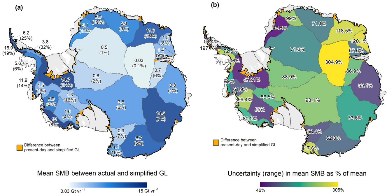
Figure 24. Magnitude and uncertainty of the surface mass balance (SMB)-correction term of the ice discharge. Ice-discharge from Antarctica is a combination of this SMB-correction term and ice discharge measured at the simplified grounding line. (a) Ensemble-mean SMB modeled by five regional climate models (RCMs) (Figure 5a) integrated over the fringe regions (yellow) bounded by the RINGS/Bedmap3 grounding line and the RINGS simplified grounding line. The values are ensemble mean SMB ( \text{Gt yr}^{-1} ) and percentage of this SMB to the mean of the two ice-discharge estimates at the simplified grounding line using Bedmap2 (Fretwell et al., 2013) and Bedmachine (Morlighem et al., 2020) bed elevations together with the ITS_LIVE velocity data (Gardner et al., 2018). (b) The range of modeled SMB using five RCMs (Section 2.4.2) integrated over the fringe regions (yellow), shown as a relative value to the ensemble-mean SMB (a).
