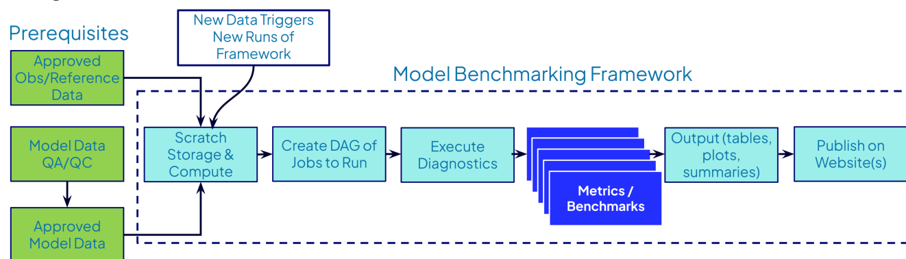
Figure 1. The high-level workflow for the Rapid Evaluation Framework (REF) run on Earth System Grid Federation (ESGF) nodes, shown here, combines quality-assured model output with a collection of observational reference data to initiate execution of relevant diagnostics and generation of tabular and graphical representations of a variety of metrics. The results are then published on websites for community use. Figure available at https://doi.org/10.5281/zenodo.15594502 (Hoffman et al., 2024).
