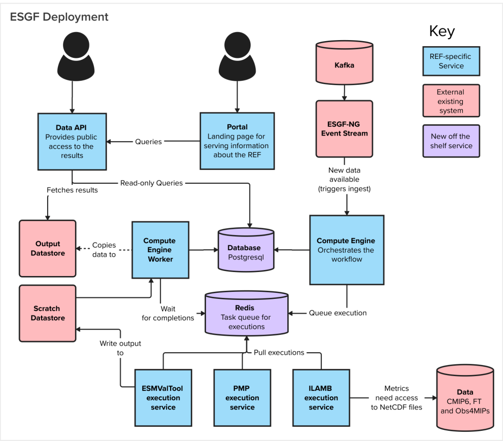
Figure 2. This detailed workflow diagram identifies key services provided by the REF and their relationships with external services and off-the-shelf components for the ESGF deployment. Figure available at https://doi.org/10.5281/zenodo.15595006 (Lewis et al., 2025b).
