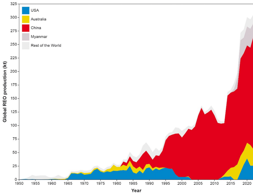
Figure 12 Historical world REE oxide production by country. Data updated by G M Mudd from Weng et al. (2015) using BGS (Idoine et al., 2024) and USGS (U.S. Geological Survey, 2024a, b) data, including historical editions of these reports, and (Anonymous, 1942a)). BGS © UKRI.
