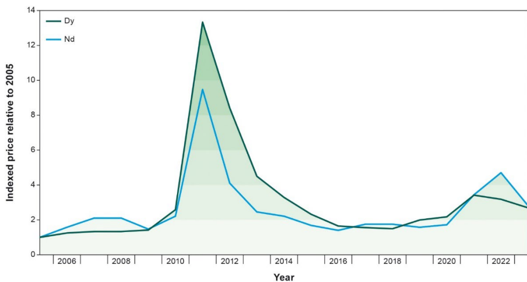
Figure 13 Average annual prices for Dy and Nd indexed to 2005. Data from USGS (U.S. Geological Survey, 2024a, b). Note: average annual prices do not show price changes at monthly or shorter time scales. BGS © UKRI.
