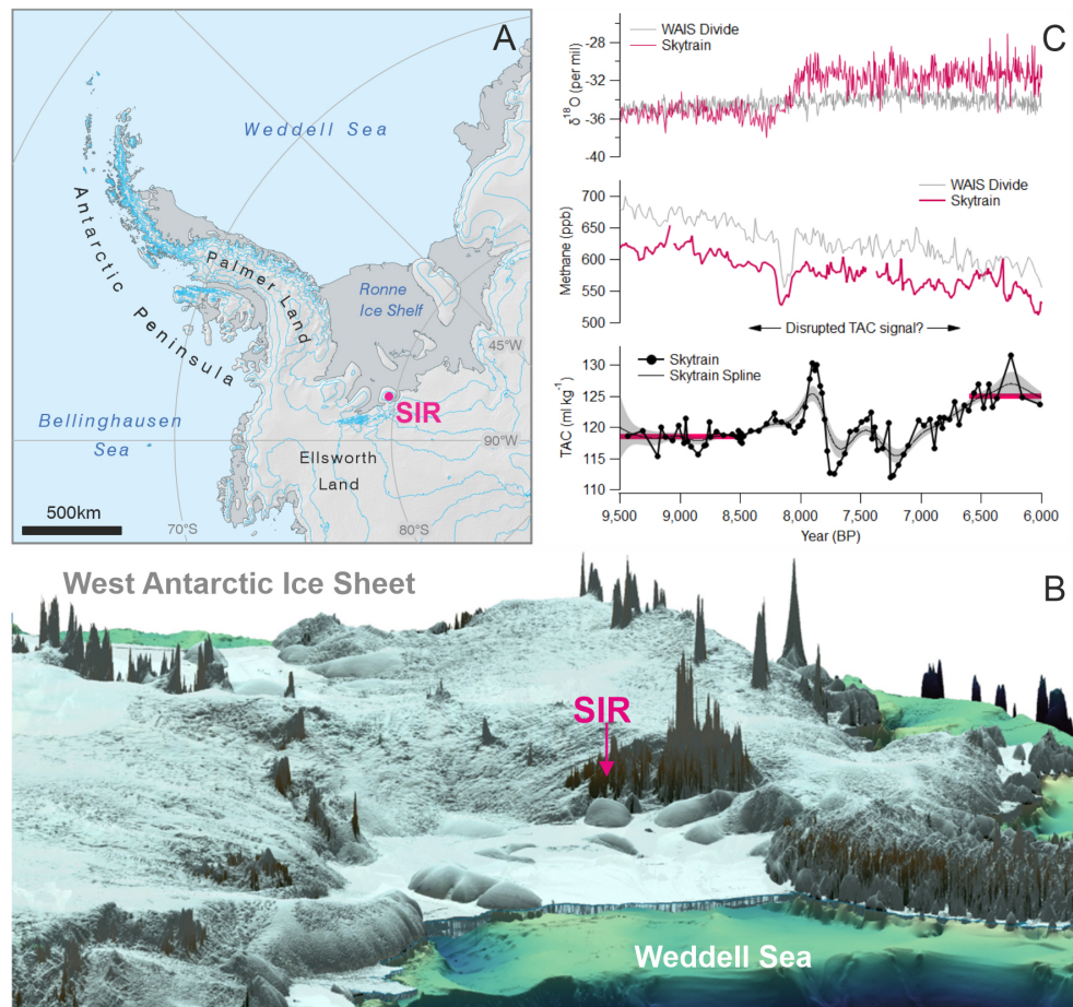
Figure 1. Present day location map of Skytrain Ice Rise (panel A, “SIR”) and shown in a 3D topographic context (panel B, Greene et al., 2017; Morlighem et al., 2020) with SIR sitting at the interface between the floating Ronne Ice Shelf and the outward flowing continental ice sheet of West Antarctica. Panel C highlights the elevation loss event, over ~200 years at ~8 ka, observed in the Skytrain ice core records, with a significant jump in water isotopes (presented on the ST22 ice age scale) caused by ice elevation loss and subsequent temperature increase at the site (Grieman et al., 2024). Comparatively, records from the central WAIS, indicated by the WAIS Divide ice core record (Fudge et al., 2013), remain relatively stable. The TAC record from Skytrain (presented on the ST22 gas age scale), which is expected to indicate elevation at SIR during the ice mass change, shows a complex oscillating signal after 8 ka which is too great to be an elevation signal, and does not re-stabilise until significantly later, ~6.5 ka. Also shown are the CH 4 record from Skytrain (on the ST22 gas age scale) and WAIS Divide (Rhodes et al., 2015; Buizert et al., 2015). Note that the vertical scaling is exaggerated in panel (B), but for reference, at time of ice core drilling, SIR was ~784 m elevation above sea level and ~688 km from the ice shelf edge.
