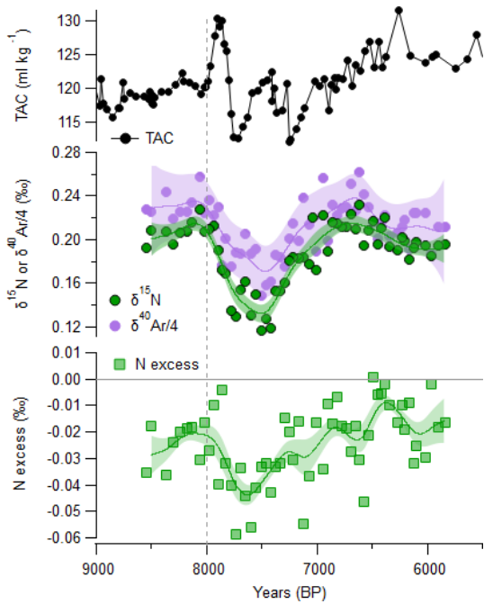
Figure 2. Values of \delta^{15}\text{N} and \delta^{40}\text{Ar} from the Skytrain ice core (middle panel) throughout the rapid elevation change at the site \sim 8 ka (dashed line), plotted against the previously published TAC data (top panel) (Grieman et al., 2024). Smoothing splines are also presented (see methods), with uncertainty bands becoming large at the ends of the dataset due to a lack of constraining data points beyond here. Also shown is the calculated N_{\text{excess}} . All records are presented on the ST22 gas age scale.
