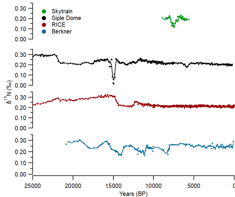
Figure 5. \delta^{15}\text{N} profiles from previously measured coastal WAIS ice cores, Skytrain (this study), Siple Dome (as published in Morgan et al., 2022), RICE (as published in Lee et al., 2020) and Berkner (as published in Capron et al., 2013).
