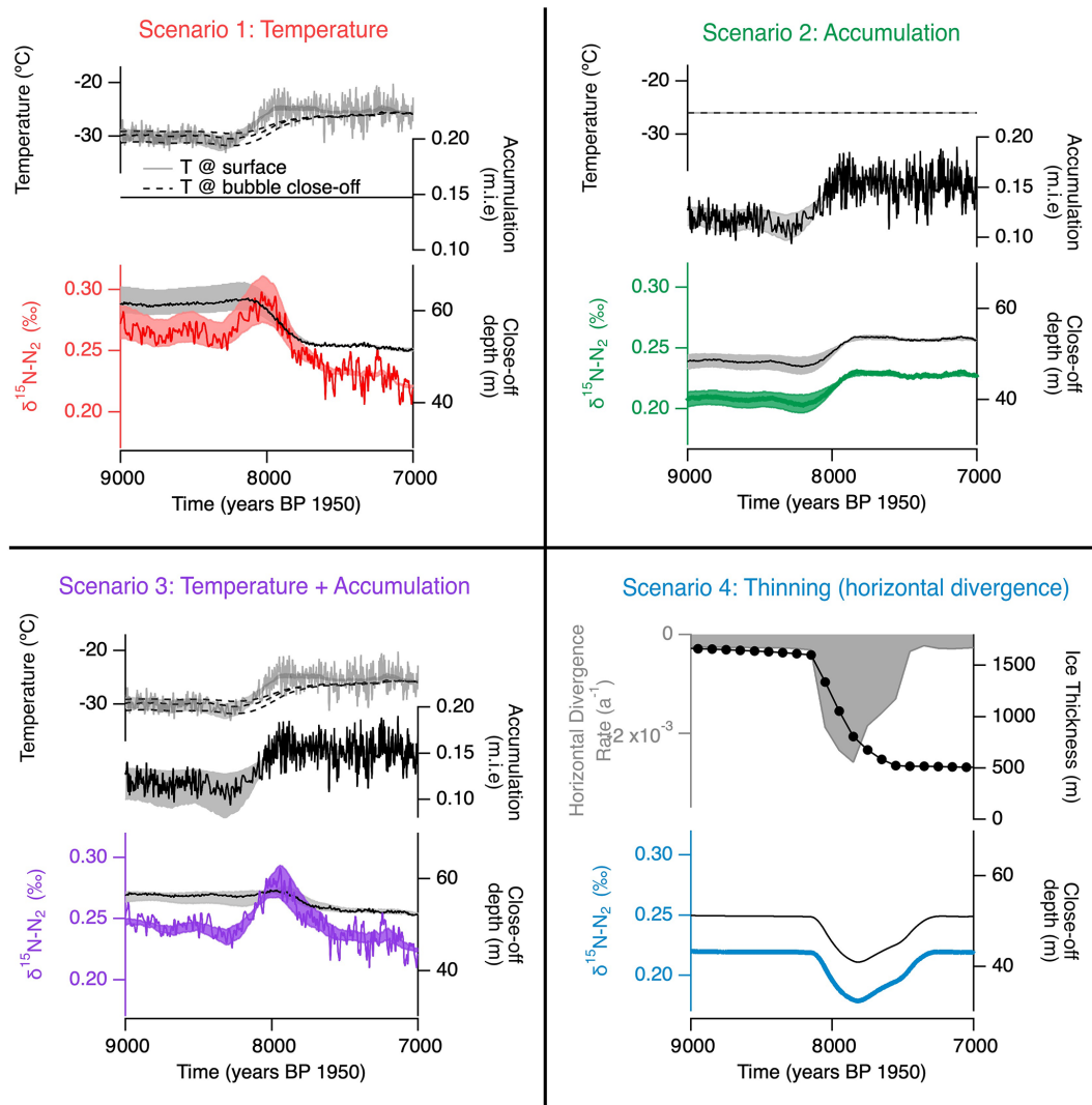
Figure 3. Factorial Experiments using the CFM to disentangle the potential drivers of \delta^{15}\text{N} variability at SIR. Panels show changes in temperature-only (red), accumulation-only (green) and a combination of temperature and accumulation (purple) with the two forcings of surface temperature (light grey) and accumulation (solid black). Also shown in these panels are the predicted temperature at bubble close-off (dashed black), the close-off depth (solid black) and the \delta^{15}\text{N} (coloured coded to the given experiment). Panel 4 shows the prediction using just the horizontal divergence calculated from PISM plus constant accumulation rate (filled in grey).
