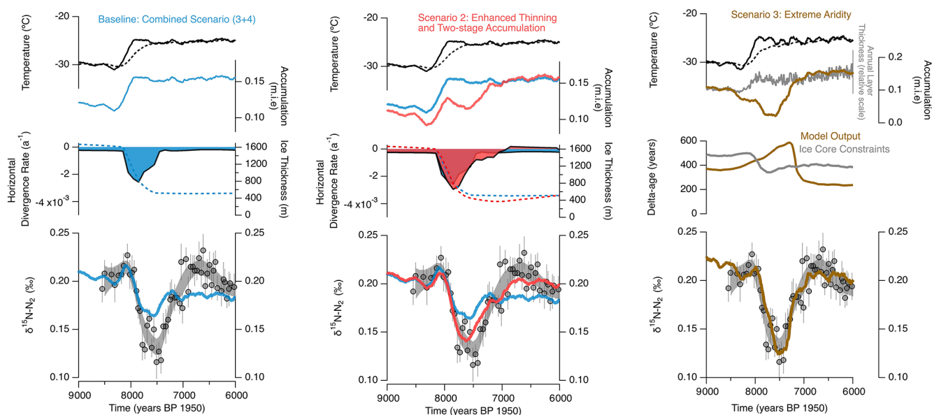
Figure 4. Optimising the model parameters to best fit data, where temperature, accumulation (top plot in each panel) and horizontal divergence rates (middle plot) are adjusted so that the model output of the absolute values of \delta^{15}\text{N} and duration of the reduction in \delta^{15}\text{N} more closely match the measured data (lower plot in all panels). The left panel shows our “baseline” scenario, that of the temperature, accumulation, and horizontal divergence previously suggested by our measured datasets, from which to build. The middle panel introduces a two stage change in accumulation and enhances the horizontal divergence rate and duration, and the right panel presents a scenario of extreme aridity to demonstrate a period of net ablation.
