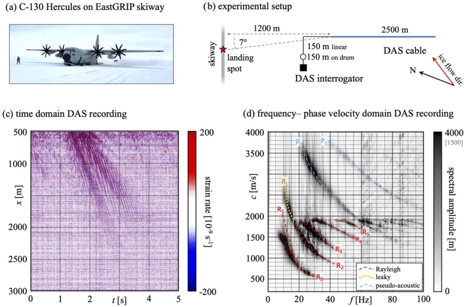
Figure A1. Airplane landing data. (a) Photograph of the C-130 Hercules, shortly after landing near the EastGRIP camp. (b) Geometry of the 3000 m long fibre-optic cable. The last ~2500 m are nearly straight, forming an angle of \sim 7^\circ to the estimated landing spot. (c) Time-domain DAS recordings on the last 2500 m of the cable. (d) Amplitude spectrum of the data in the frequency–phase velocity domain. Marked features include multiple Rayleigh modes ( R_i ), a leaky mode ( R_L ) and pseudo-acoustic modes ( P_0 ). Frequencies above 60 Hz are shown with a lower colour bar saturation, for better visibility.
