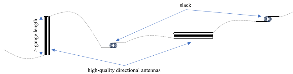
Figure 5. Schematic surface cable layout. The cable (grey dashed lines) includes looped sections (black solid lines) that serve as high-quality directional antennas or provide slack, especially needed on moving glaciers.
