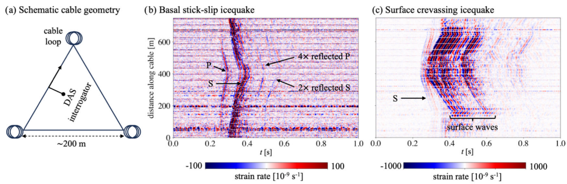
Figure 10. Examples of a basal stick-slip icequake and a surface crevassing icequake recorded on Rhône Glacier, Swiss Alps. (a) Schematic illustration of the triangular cable layout, including loops in each of the corners. Grey numbers are distance along the fibre. (b) Recording of a basal stick-slip icequake, including multiply reflected P and S waves. (c) Recording of a surface crevassing event, dominated by dispersed surface waves.
