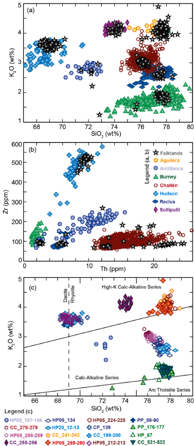
Fig. 3. (a) Major (EMPA) and (b) trace element (LA-ICP-MS) data from the Falkland Island cryptotephra deposits plotted against data from the South American BOOM database (Fontaine et al., 2023; references therein). Additional comparative data are from Panaretos et al. (2021) and Monteath et al. (2019). Note that LA-ICP-MS data is not available for all South American volcanoes or cryptotephra deposits from HP05. (c) Major element data from the Falkland Island cryptotephra deposits plotted following K 2 O v SiO 2 nomenclature after Peccerillo and Taylor (1976).
