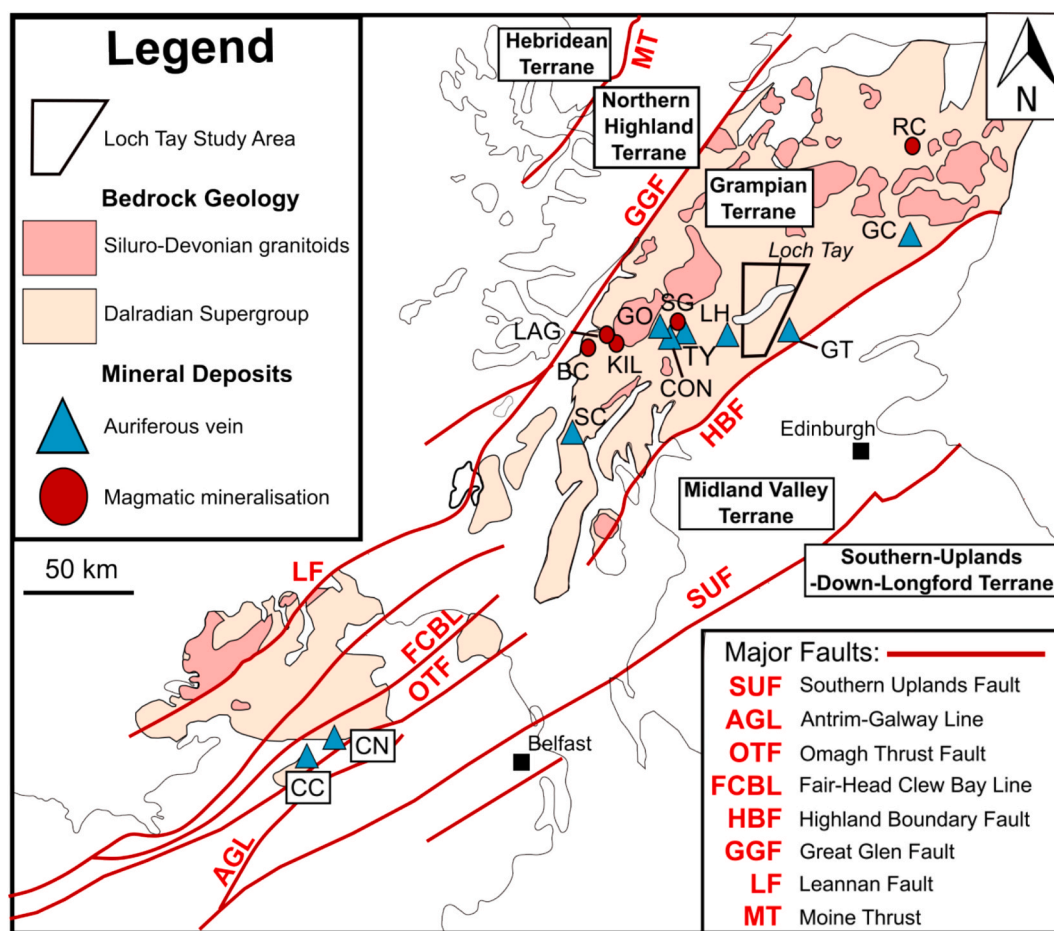
Fig. 1. Gold-bearing veins and magmatic gold mineralization in the Grampian Terrane (Shaw et al., 2022). The following abbreviations have been used: RC = Rhynie Chert (Baron et al., 2004), GC = Glen Clova (Smith et al., 2003), GT = Glen Turret (Smith et al., 2003), LH = Locheearnhead (Smith et al., 2003), TY = Tyndrum (Curtis et al., 1993), CON = Cononish (Rice et al., 2012), SG = Sron Garbh (Graham et al., 2017), GO = Glen Orchy (Hill et al., 2013), LAG = Lagalochoan (Zhou, 1987), KIL = Kilmelford (Zhou, 1988), BC = Beinn nan Chaorach (Smith et al., 2003), SC = Stronchullin (Naden et al., 2010), CN = Curraghinalt (Rice et al., 2016), CC = Cavanacaw (Parnell et al., 2000). Furthermore, there are several occurrences of polymetallic mineralization around Loch Tay (Fig. 2), the outline of which is represented approximately using white infill.
