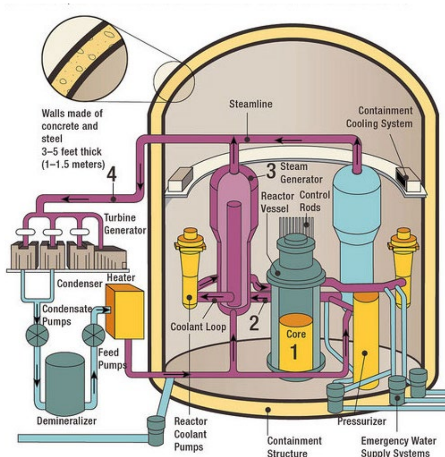
Figure 2 Salient components of a PWR (Nuclear Regulatory Commission, 2023). © NRC
