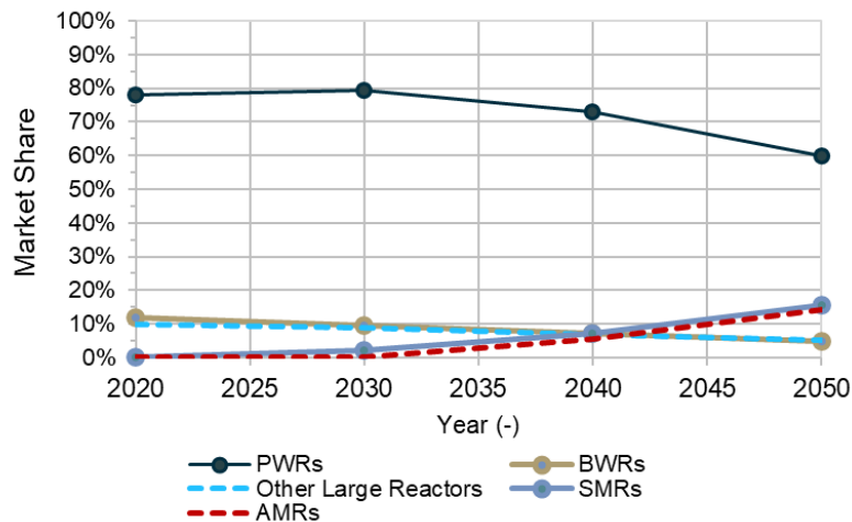
Figure 13 Global nuclear subtechnology market share to 2050. BGS © UKRI.
