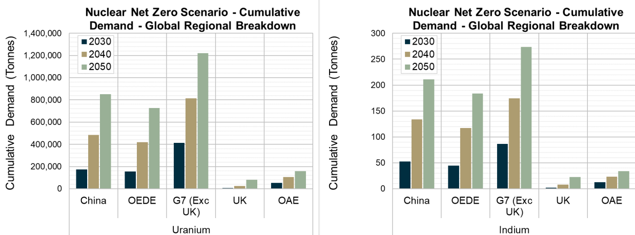
Figure 15 Cumulative material demand for selected elements (in tonnes) embedded in nuclear in the UK, China, G7 (excluding UK), OEDE and OAE in 2030, 2040 and 2050. The data for the non-UK demand projections are based on IEA data (International Energy Agency, 2022). Data for the other materials is presented in Appendix C. BGS © UKRI.
