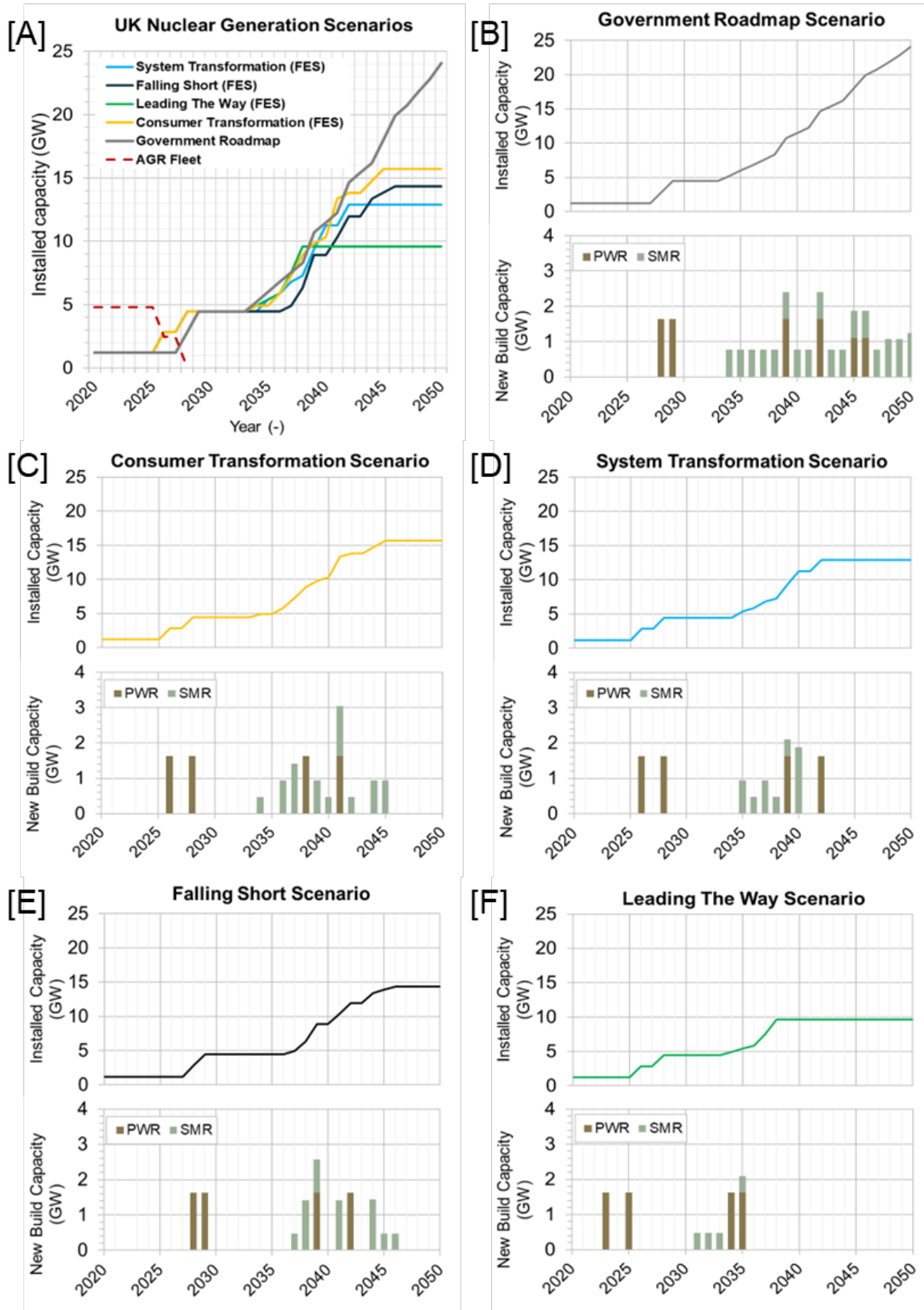
Figure 10 UK nuclear deployment scenarios, showing A: the full set of five scenarios; B: Government Roadmap; C: 'Consumer transformation'; D: 'System transformation'; E: 'Falling short'; F: 'Leading the way' (FES). (UK Government, 2024a; National Grid, 2023). BGS © UKRI.
