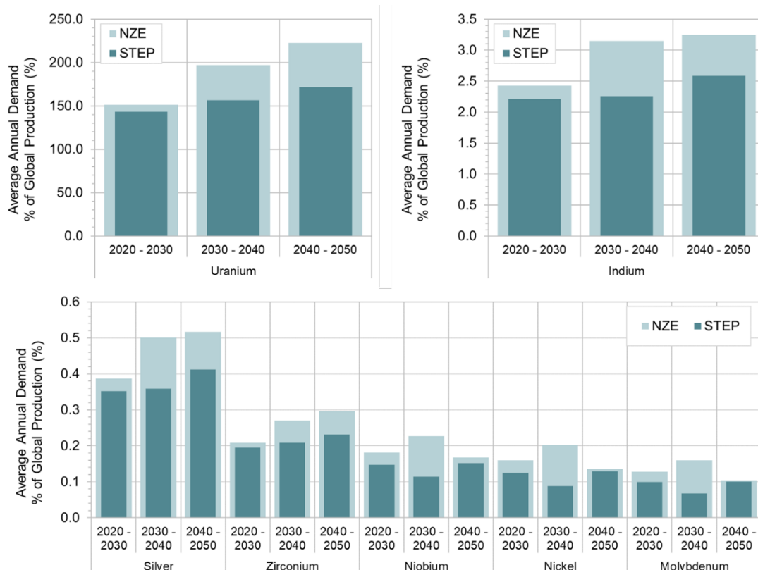
Figure 14 Average annual global demand as a percentage of current global metal production for materials with highest relative demand in nuclear technologies. Outputs based on two scenarios: NZE and STEP from IEA analysis (International Energy Agency, 2022) BGS © UKRI.
