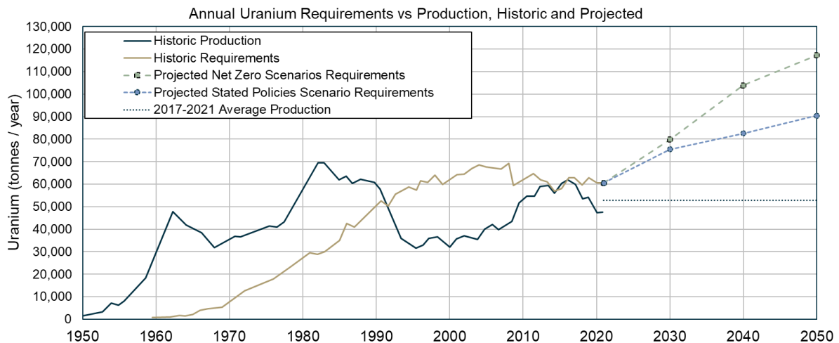
Figure 16 Historic and projected annual requirements and demand for uranium. Historic data from NEA and IEA (Nuclear Energy Agency, International Atomic Energy Agency, 2022). Projected requirements: DAS Ltd analysis. BGS © UKRI.
