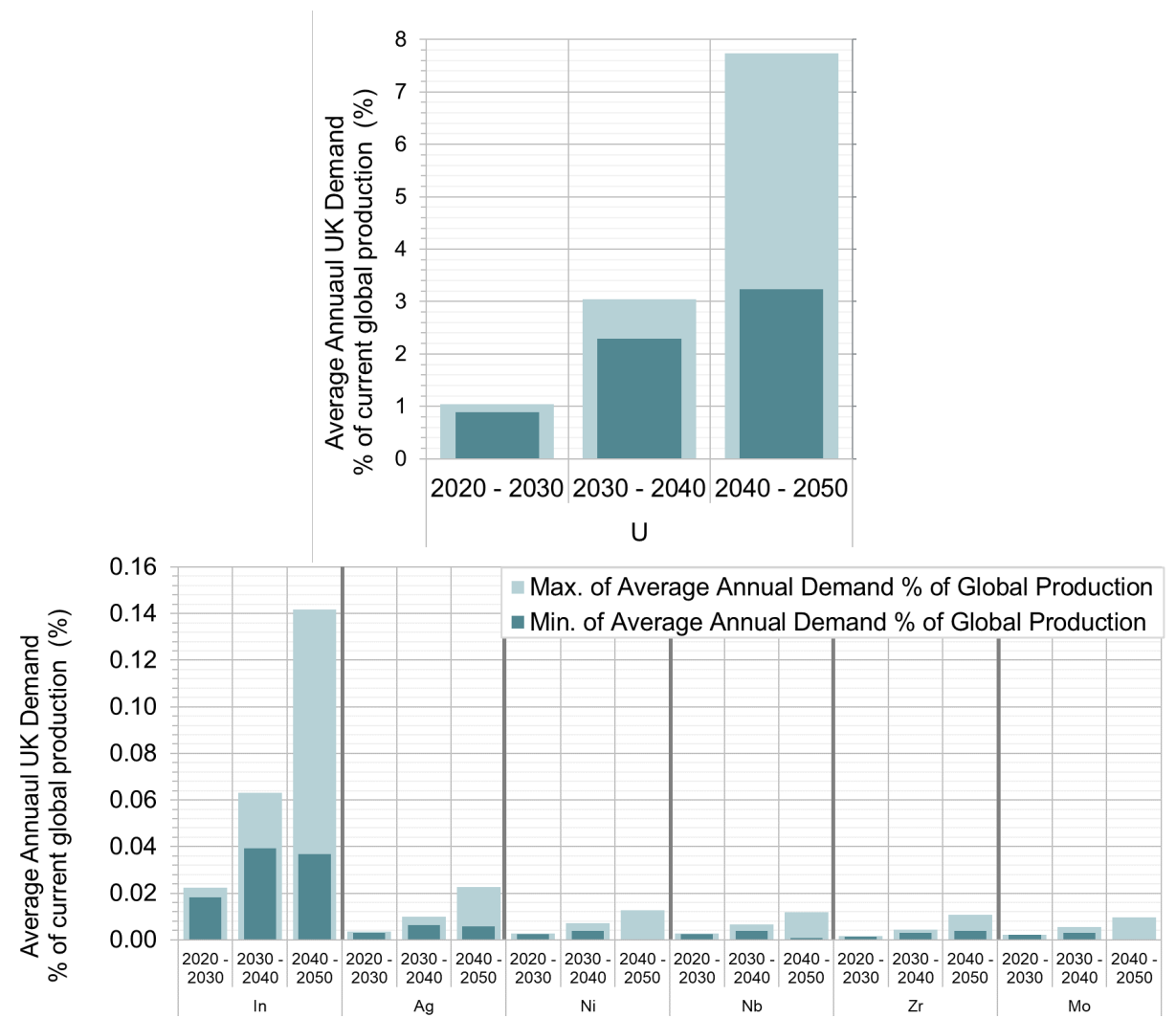
Figure 12 Average annual UK demand to 2030, 2040, 2050 as a percentage of current global metal production (five-year average, 2017 to 2021). The minimum and maximum values represent outputs of the different scenarios. BGS © UKRI.
