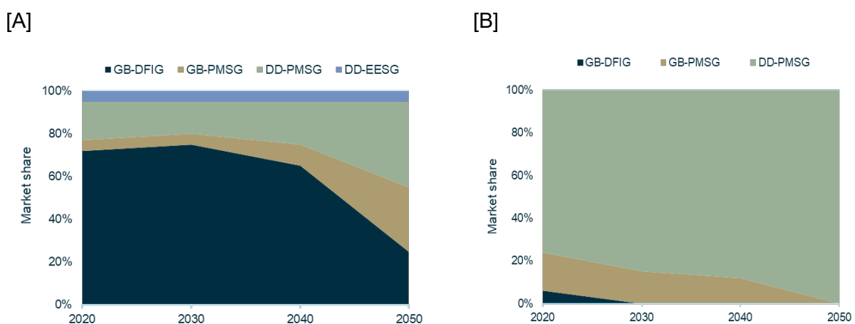
Figure 10 Evolution of the wind turbine market [A] onshore and [B] offshore between 2020 and 2050, showing the technology transformation that is likely to take place (European Commission et al., 2020b, Liang et al., 2023). The market shares shown were used in the material demand calculations. GB-DFIG: Gearbox double-fed induction generator; GB-PMSG: gearbox permanent magnet synchronous generator; DD-PMSG: direct drive permanent-magnet synchronous generator; DD-EESG: direct drive external excitation synchronous generator. BGS © UKRI.
