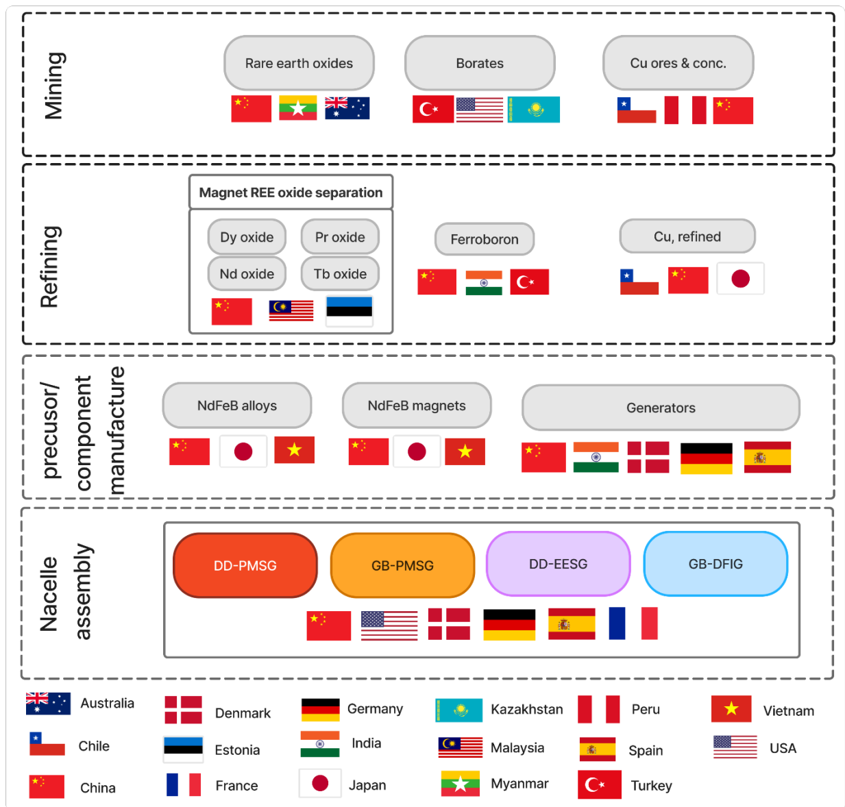
Figure 4 Geographical production concentration in the wind turbine supply chain. All steps show the top three producers, from left to right, except for ferroboron, and for the manufacture of generators and wind turbines where the flags highlight key producers, but their order does not reflect their respective market share. Materials at the mining stage and Cu at the refining stage are based on quantitative data for 2017 to 2021 from the BGS World Mineral Statistics Database (Idoine et al., 2023). The top three producing countries of REOs at the refining stage and the NdFeB alloy production are from Adamas Intelligence Inc. (2022); magnet manufacturing data are based on data from Smith et al. (2022). Production shares of generator and wind turbine manufacturing countries are based on data from Hutchinson and Zhao (2023). REE: rare earth elements; DD: direct drive; GB: gearbox; PMSG: permanent-magnet synchronous generator; EESG: electrically excited synchronous generator; DFIG: double-fed Induction generator. BGS © UKRI.
