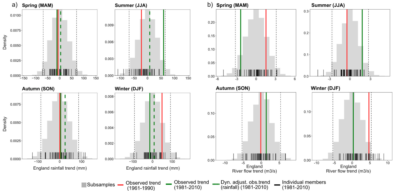
Fig. 3. Linear trend in a) mean seasonal rainfall and b) seasonal river flows over 30-year periods averaged for catchments in England. The grey shaded distribution represents the probability distribution of 10,000 sub-samples of 30-year length and the short solid black lines represent the linear trend of each ensemble member over the 1981–2010 period. The short solid black lines do not relate to values on the y-axis. The solid red and green lines represent the observed trend in rainfall and “simulated observed” trend for river flows over the 1961–1990 and 1981–2010 period respectively. The dashed green line represents the dynamically adjusted observed rainfall trend (observed minus dynamically reconstruction trend) for the 1981–2010 period. The dashed black lines represents the 2.5–97.5th percentiles, covering 95% of the model distribution. (For interpretation of the references to colour in this figure legend, the reader is referred to the web version of this article.)
