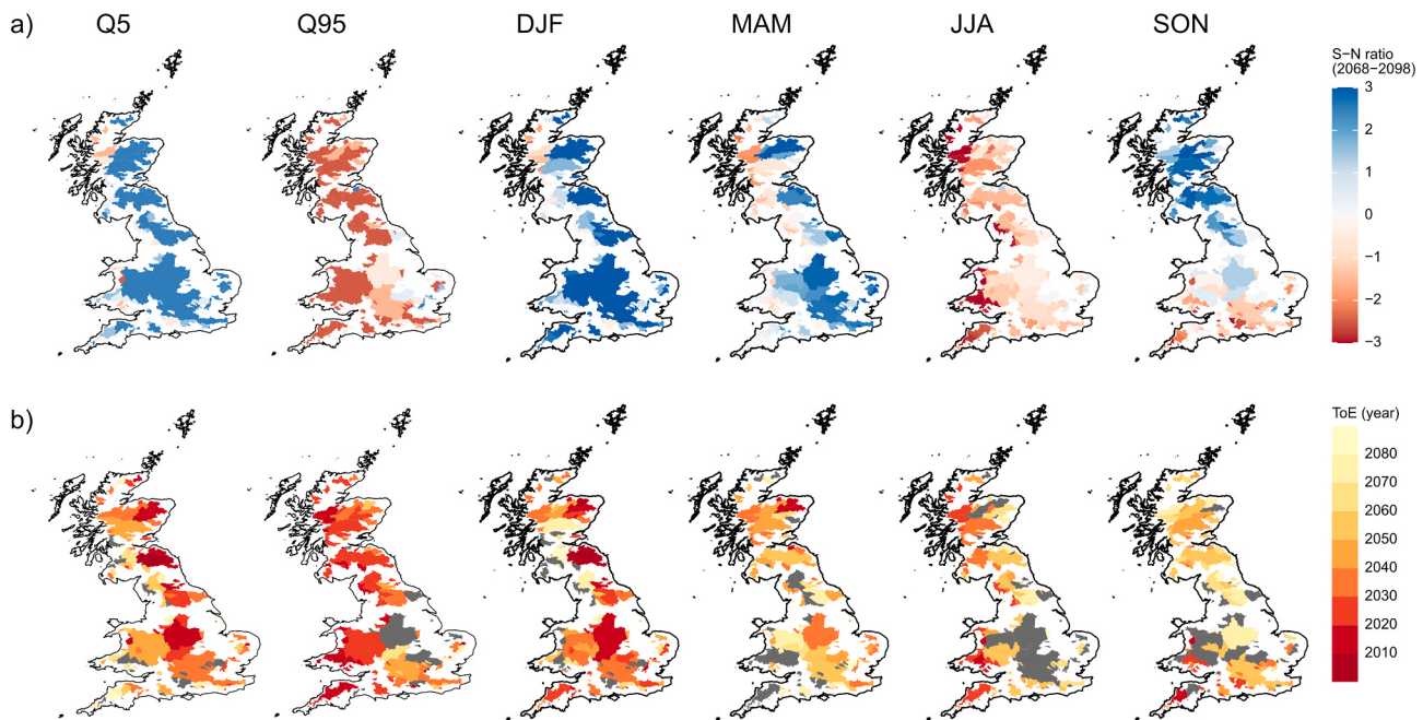
Fig. 7. a) Signal-to-noise (S-N) ratio (2068–2098) and b) the estimated Time of Emergence (ToE) (middle year of 30-year period) for high flows (Q5), low flows (Q95) and mean seasonal river flows. The catchments coloured in grey are ones where the ToE is not reached by the end of the 21st century.
