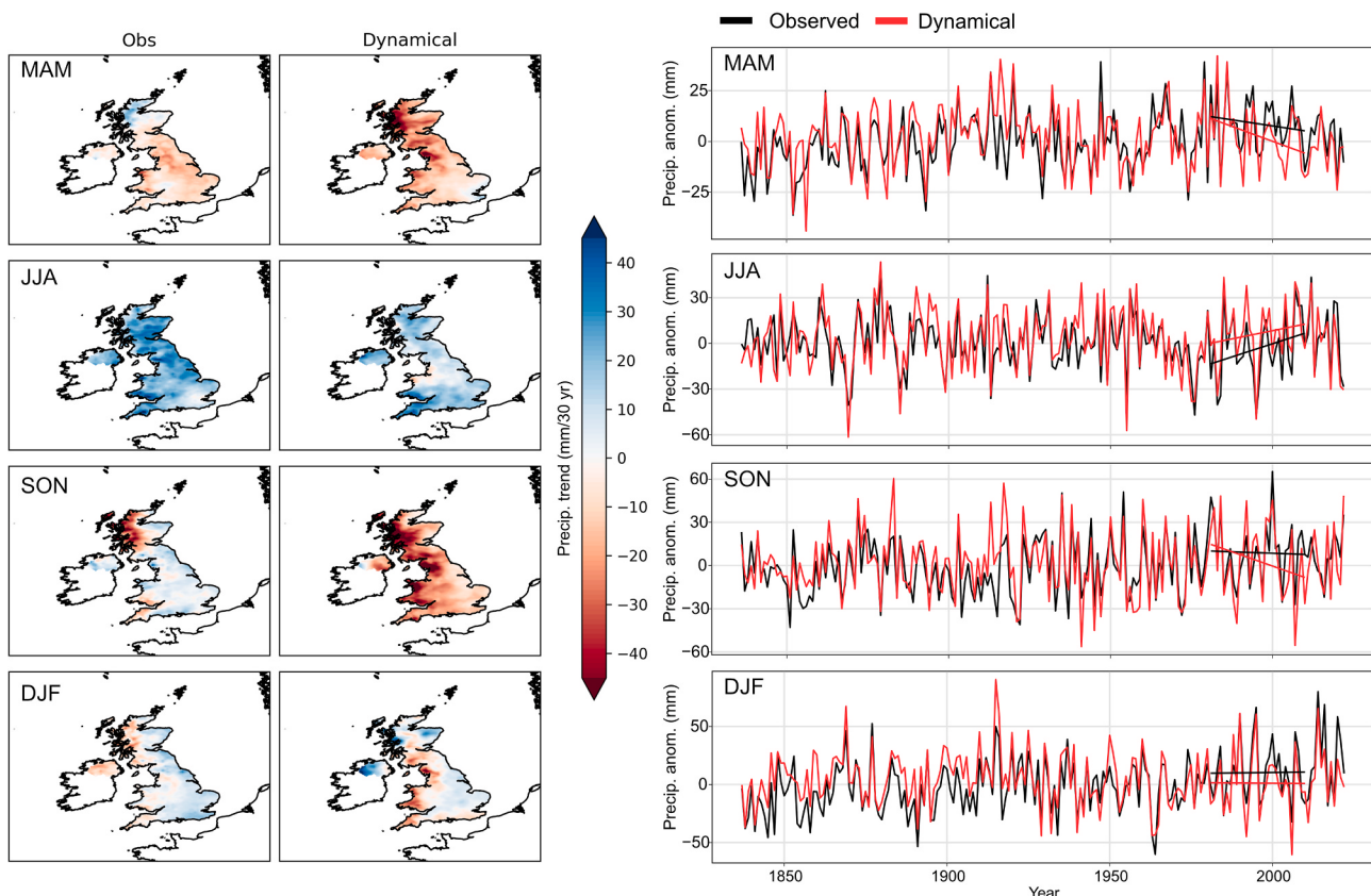
Fig. 2. Observed and dynamically reconstructed rainfall trend (mm/30-yr) over the 1981–2010 period (left) and UK-averaged anomalies (mm) over the entire 1836–2022 period (right) for each season for both the observed (black) and dynamically reconstructed (red) rainfall. The linear trend over 1981–2010 for observed (black) and dynamically reconstructed (red) rainfall is shown for each season. (For interpretation of the references to colour in this figure legend, the reader is referred to the web version of this article.)
