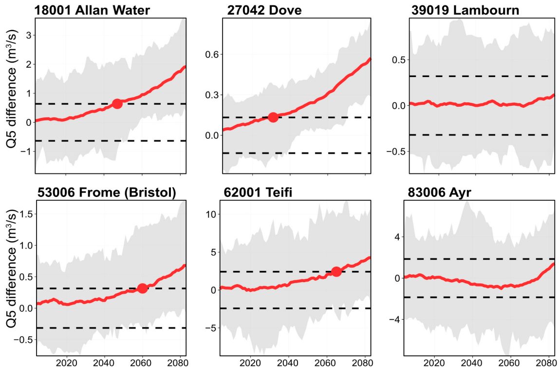
Fig. 6. Relative change ( \text{m}^3/\text{s} ) in a) low flows (Q95) and b) high flows (Q5) over consecutive 30-year time slices and the baseline reference period (1981–2010) for six selected catchments. The year on the horizontal axis represents the middle year of each 30-year time block and the shading the spread across the ensemble members. In each panel, the solid red line represents the ensemble mean and dashed horizontal black lines represent the range of internal variability (i.e., \pm 1 standard deviation over the reference period). The red circle denotes the Time of Emergence (ToE) when the ensemble mean difference exceeds range of historical variability. The location of the six selected catchments is presented in Fig. S2. (For interpretation of the references to colour in this figure legend, the reader is referred to the web version of this article.)
