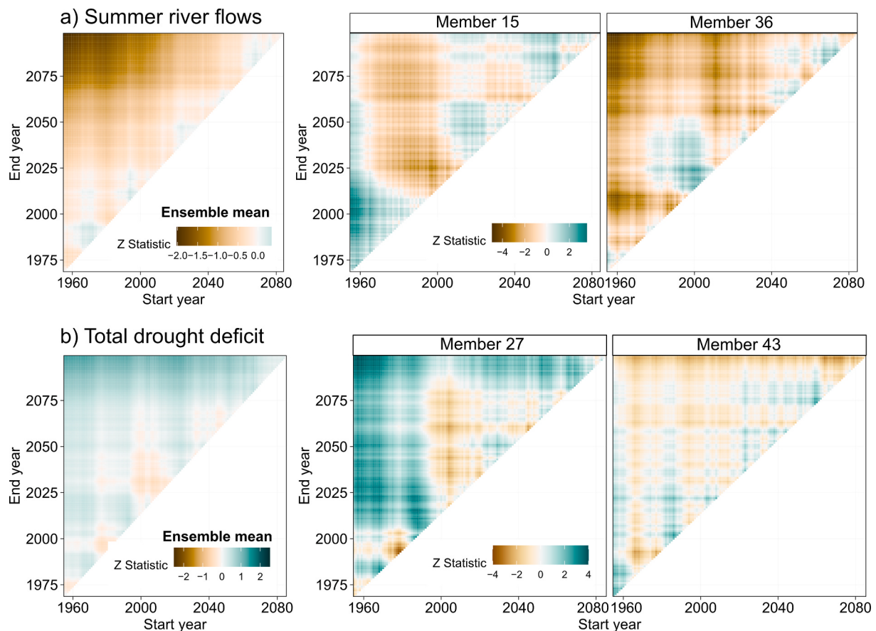
Fig. 5. Ensemble mean multi-temporal trend analysis represented via the Mann-Kendell Z statistic (colors) for a) summer river flows and b) total drought deficit calculated using a Q70 threshold averaged over all catchments in England (ensemble mean) and the equivalent for two contrasting ensemble members with the maximum and minimum long-term (1955–2099) trend. Trend is calculated for every 15-year block between 1955 and 2099 with varying start (horizontal axis) and end years (vertical axis).
