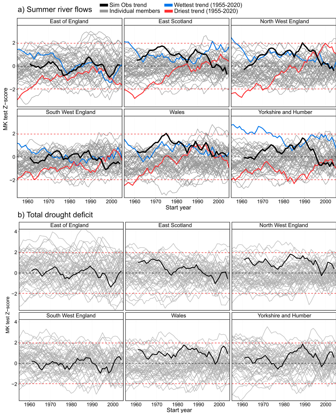
Fig. 4. MK Z-statistic in a) summer river flows and b) annual total drought deficit calculated using a Q70 threshold averaged across catchments in six different administrative regions computed from varying the start year with a fixed end year. Positive (negative) Z statistic indicate a positive (negative) trend. The trend over the observational period is calculated from 1961 with 2018 as the end year and the trend for each ensemble member of the large ensemble is calculated from 1955 with 2020 as the end year. The location of the six administrative regions is presented in Fig. S2. Serial correlation was found for 4.2% and 8.6% of the time series analysed across all catchments and time periods for summer river flows and total drought deficit, respectively.
