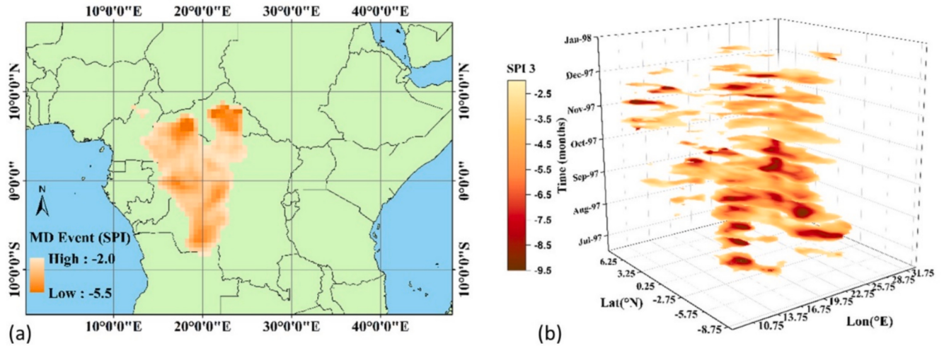
Fig. 1. Spatiotemporal evolution of a meteorological drought event, (a) spatial coverage of the drought event, (b) drought event as 3D cluster of grid cells.
