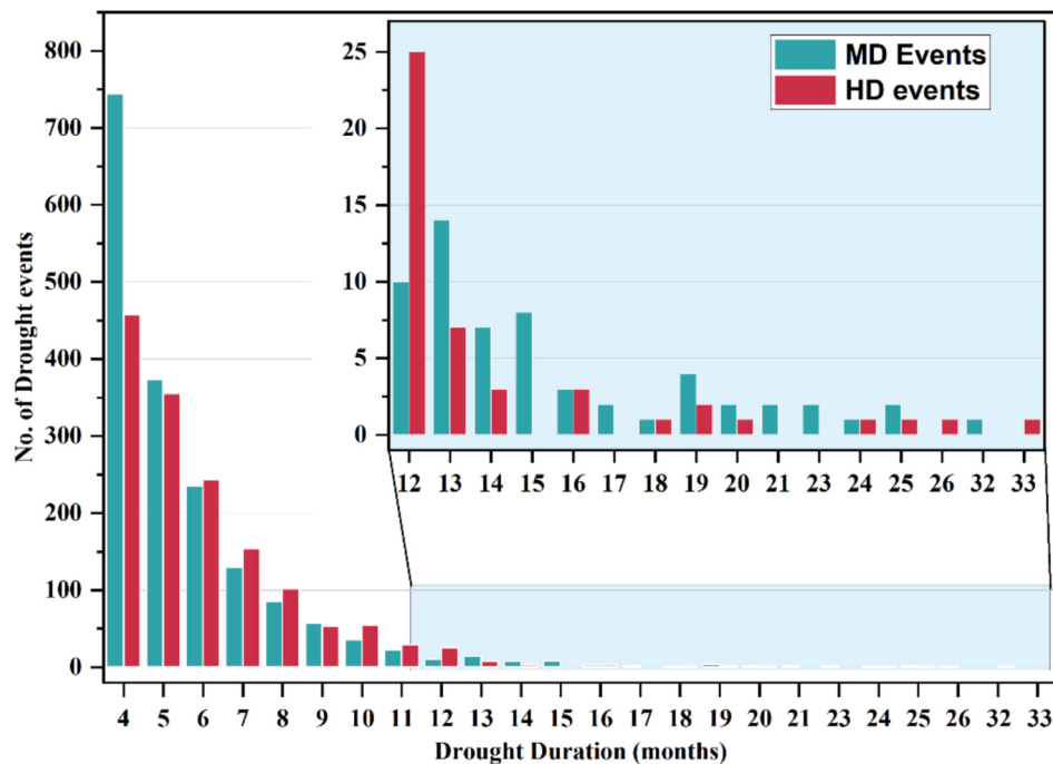
Fig. 5. Frequency distribution of MD and HD events based on duration of drought events.
