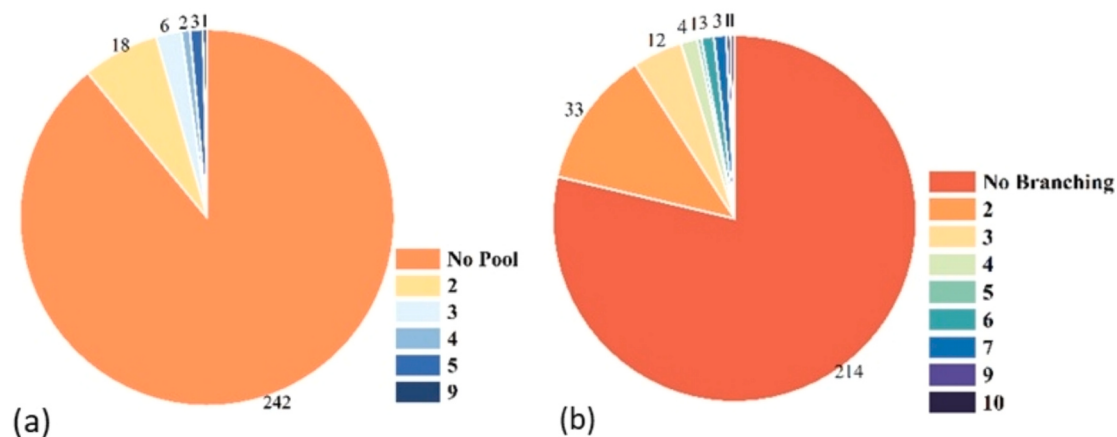
Fig. 8. Propagated MD events showing number of events exhibiting (a) pooling, and (b) branching.
