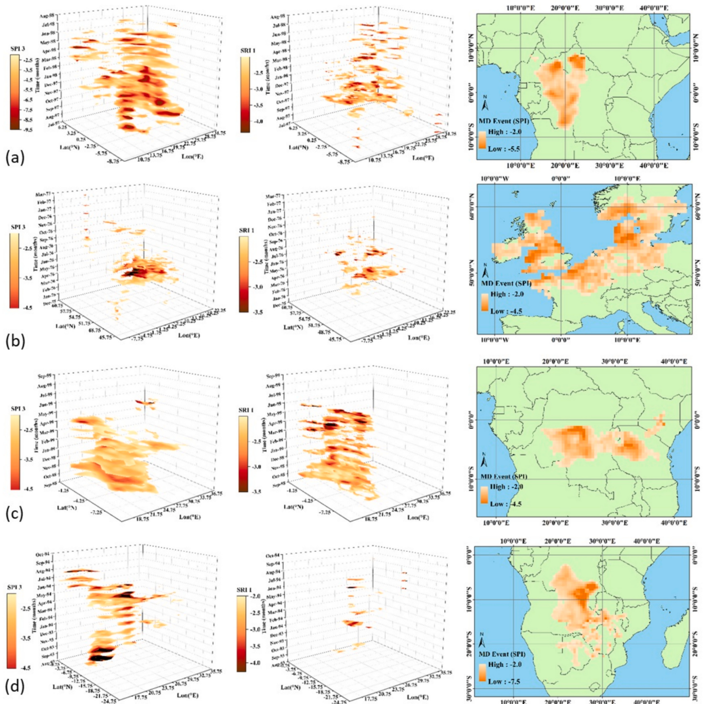
Fig. 7. Propagation of drought events from MD to HD with its spatial coverage in each panel, showing propagation features ‘pooling’ and ‘branching’: (a) M-1481 (with no pooling and branching), (b) M-252 (with no pooling but branching), (c) M-1571 (with pooling but no branching), and (d) M-1125 (with pooling and branching).
