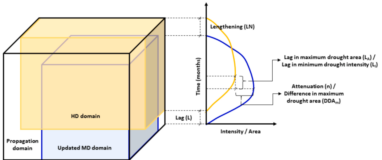
Fig. 4. Conceptual diagram showing updated meteorological drought (MD), hydrological drought (HD) and propagation domains along with graphical representation of propagation features.
