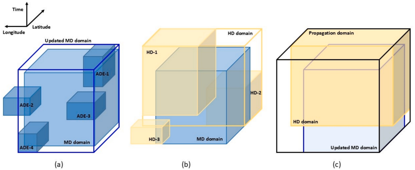
Fig. 3. Conceptual diagram showing role of (a) meteorological drought and (b) hydrological drought domain in defining (c) propagation domain; Additional Drought Events (ADE-x) and hydrological drought events (HD-x) having >70 % of their grids overlapping MD domain in their respective datasets i.e. ADE-1, ADE-2 and ADE-3 in meteorological dataset, and HD-1 and HD-2 in hydrological dataset were used to update MD domain and HD domain.
