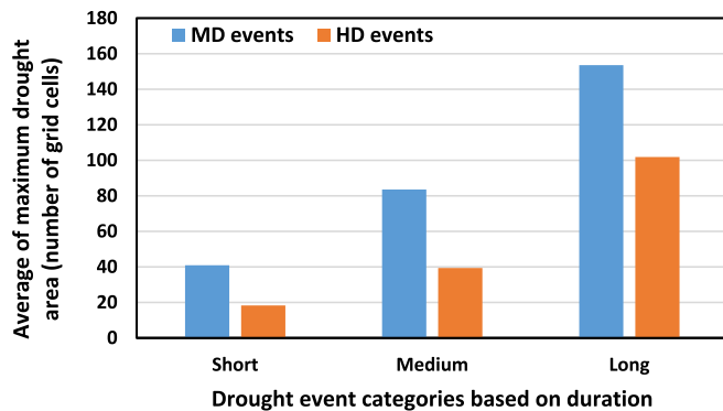
Fig. 6. Average maximum drought area (average DA_m ) for MD and HD under three drought event categories (short-, medium-, and long-term events).
