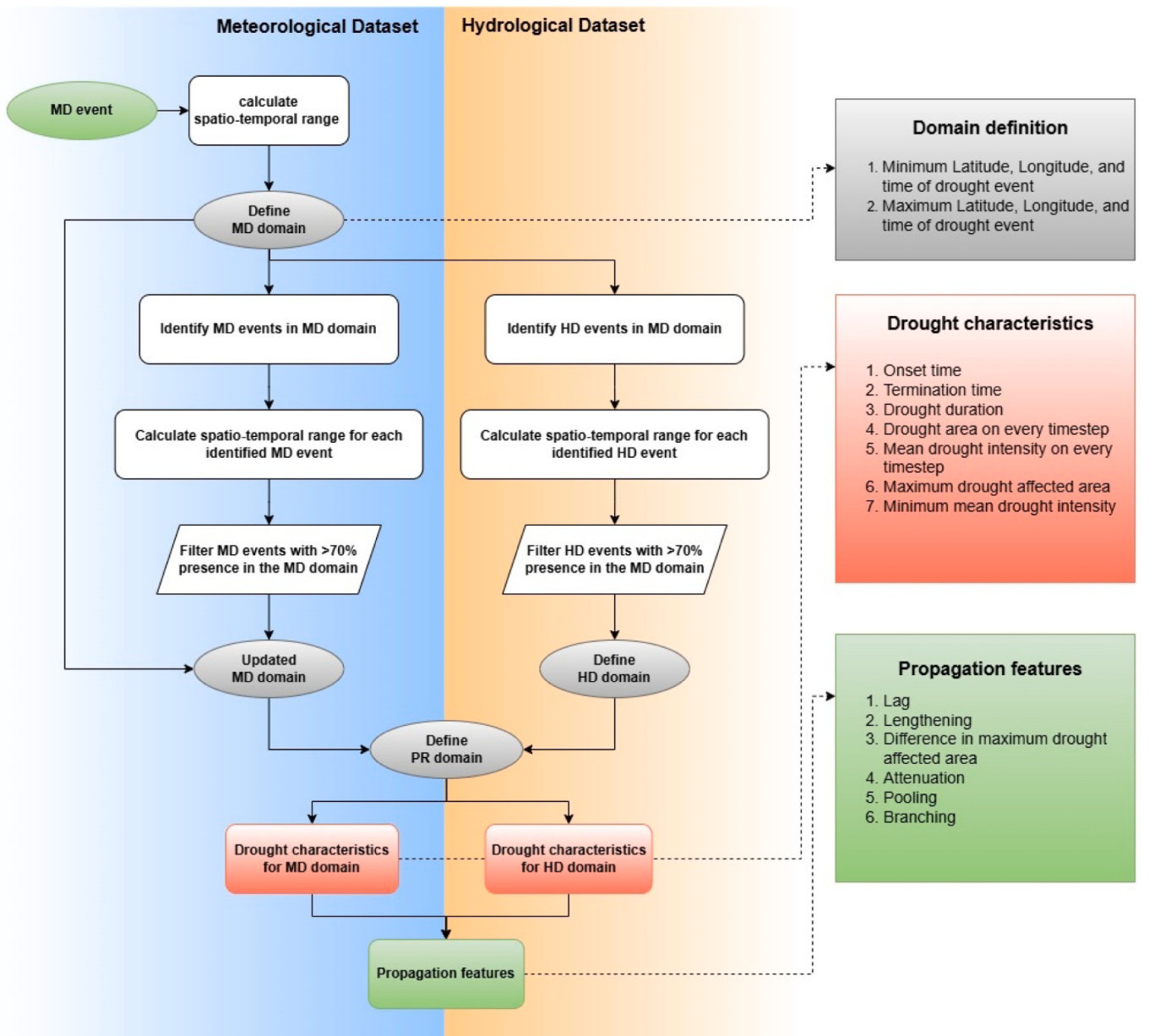
Fig. 2. Flow diagram showing the sequence for calculating 3D drought extents and extraction of key drought characteristics and propagation features.
