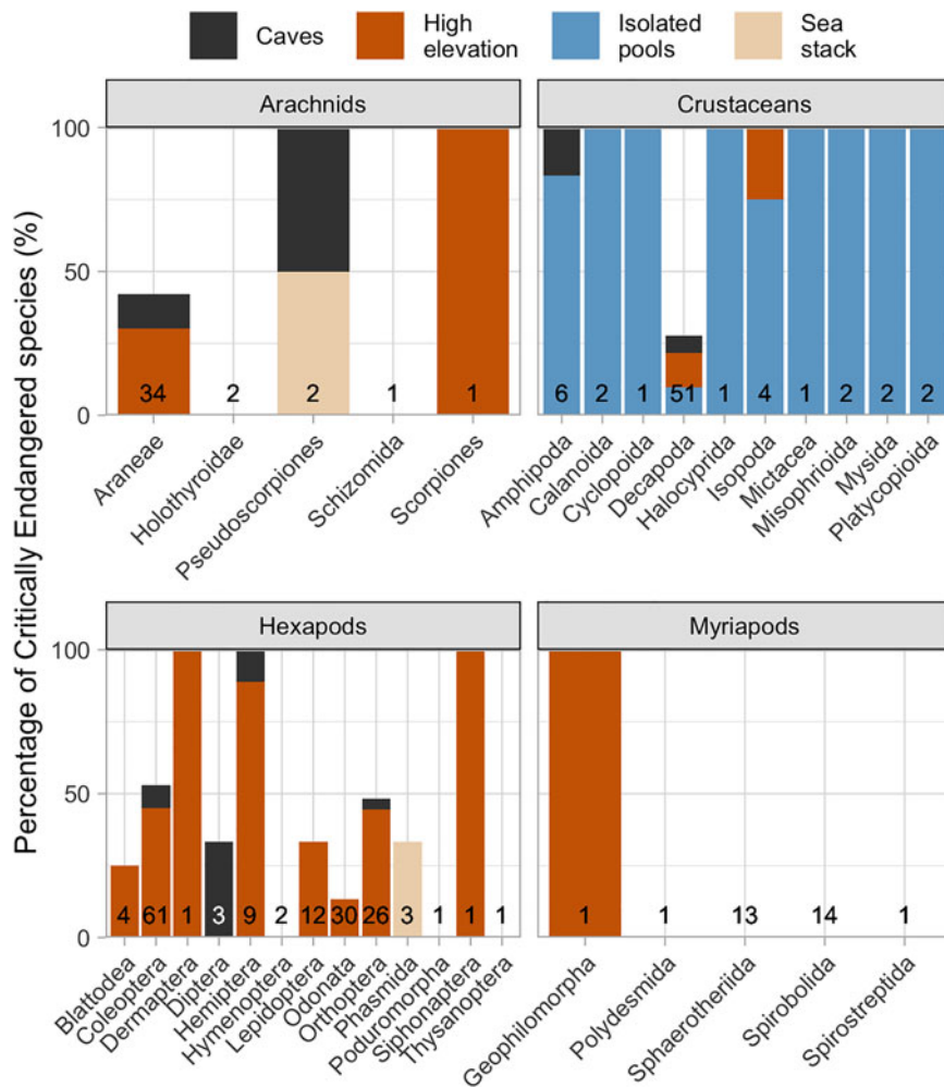
FIG. 2 Per cent of Critically Endangered arthropods from 33 orders that were reported as being confined to one of four micro-refugia. Numbers above the x-axis represent the number of individual species assessments from each taxonomic order.
