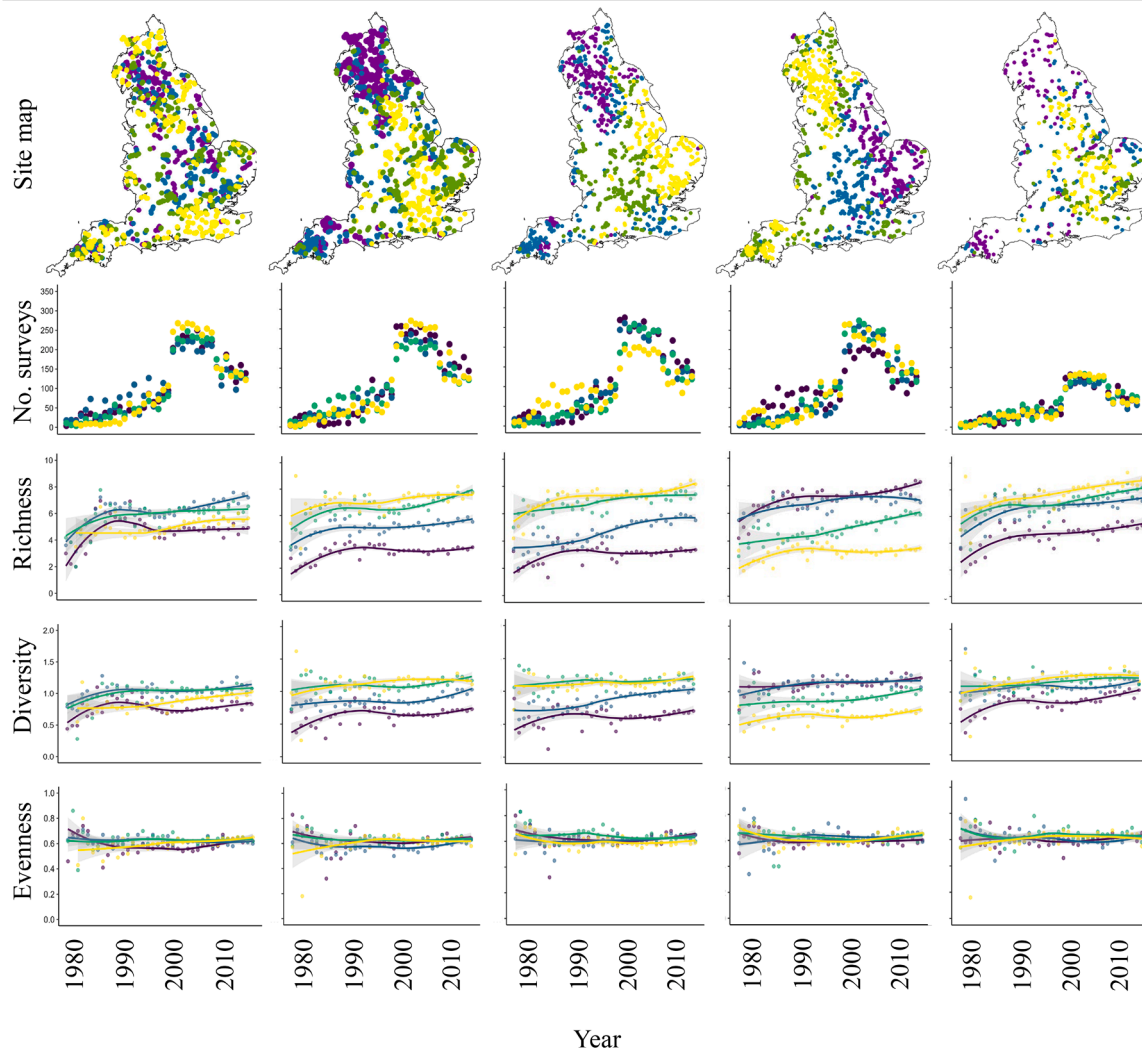
Fig. 2. Fish site locations, survey numbers and mean species richness, diversity and evenness in England's rivers between 1980 and 2017 according to land use (woodland, urban, arable, semi-natural) and wastewater exposure category.
