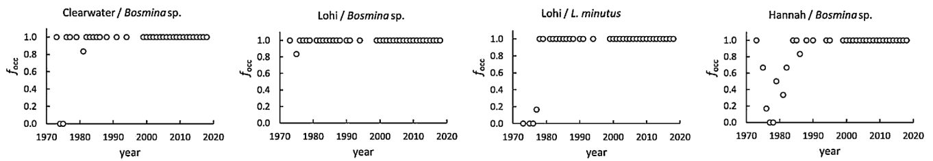
Fig. 5. Variations of f_{occ} with time for insensitive Type A species that could not be fitted owing to the lack of data at high F_{TOX} (see Section 3.2).
