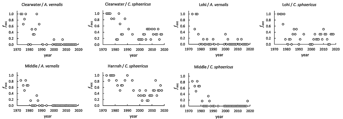
Fig. 6. Variations of f_{occ} with time for insensitive Type B species that could not be fitted owing to the lack of data at high F_{TOX} (see Section 3.2).
