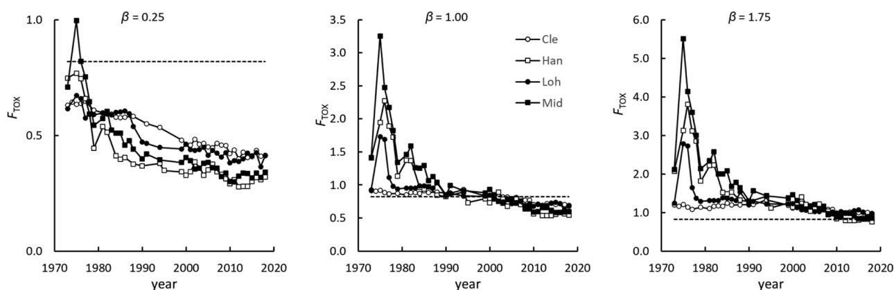
Fig. 2. Values of F_{TOX} over time for the four lakes, for \beta = 0.25, 1.00 and 1.75 . For reference, the dashed line shows the values of F_{TOX,50} (0.82); see Section 2.5. Note the different fitting scales on the y-axis.
