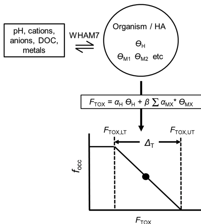
Fig. 1. Schematic of the application of WHAM- F_{TOX}\beta .
