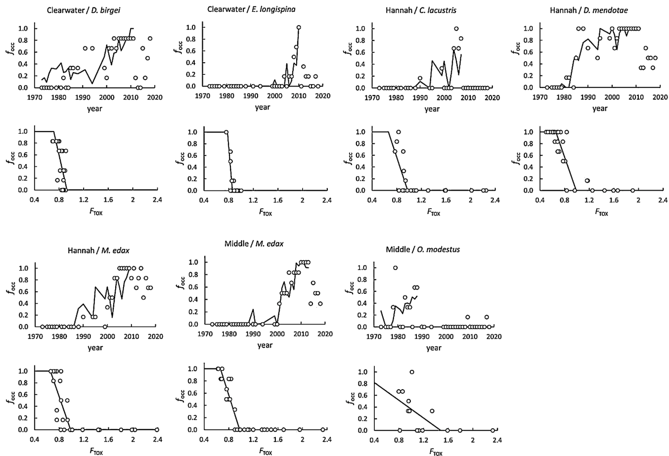
Fig. 4. Variations of f_{occ} with time (upper panels for each species) and F_{TOX} (lower panels), for Type B species-lake pairs. The points are observed values and the lines are model fits; note that fitting was done only for the results over the period during which f_{occ} increased to a maximum, indicated by the extents of the fitted lines. In the lower plots ( F_{TOX} on the x-axis), the direction of time is generally from right to left.
