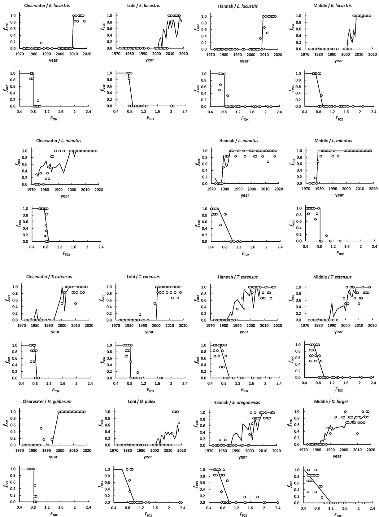
Fig. 3. Variations of f_{occ} with time (upper panels for each species) and F_{TOX} (lower panels), for selected Type A species-lake pairs. The points are observed values and the lines are model fits. In the lower plots ( F_{TOX} on the x-axis), the direction of time is generally from right to left. The remaining fitted Type A results are shown in Fig. S4.
