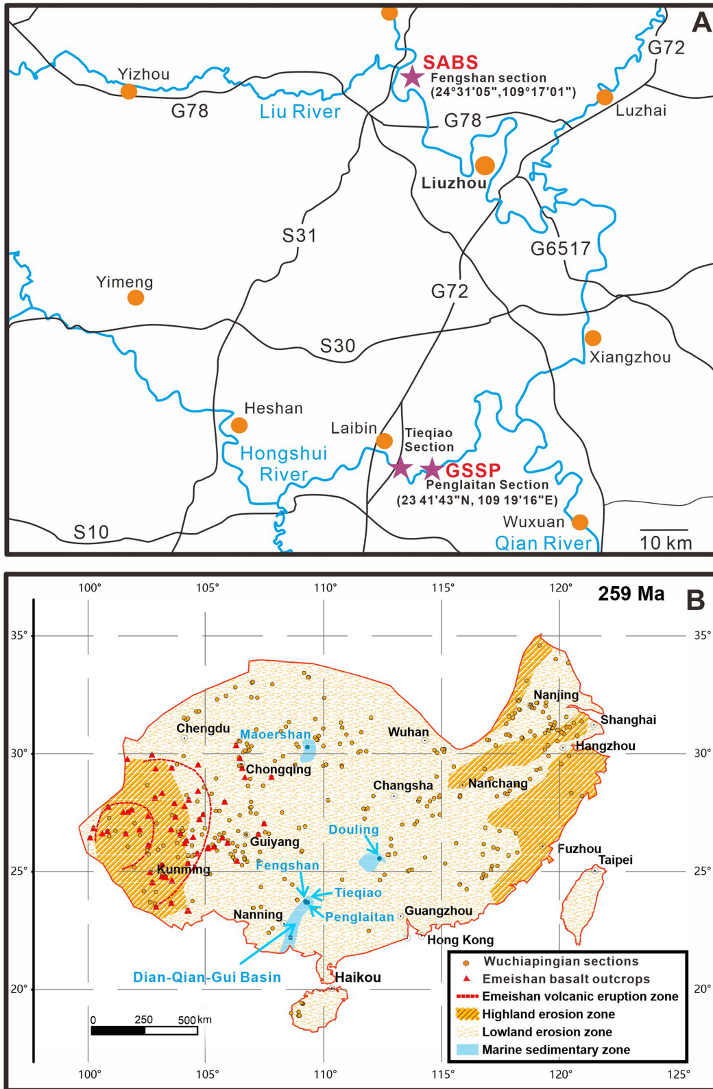
Figure 4. Map of Guangxi Province, South China showing the studied sections (A) and paleogeographical reconstruction map of the South China block during the Guadalupian/Lopingian boundary (after Hou et al., 2020) showing the locations of the Penglaitan, Tiejiao and Fengshan sections (B).
