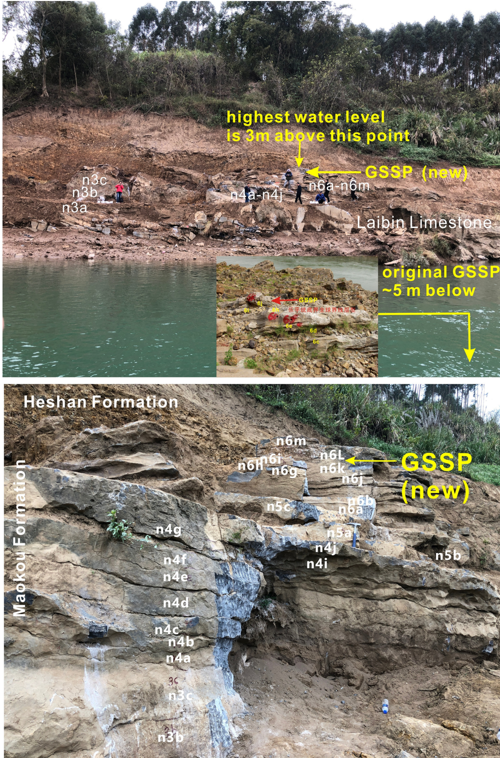
Figure 1. Photos showing the normal water level of the Hongshui River and the new section with the newly defined GSSP. All bed numbers are prefixed with “n” to differentiate from those of the original GSSP section under water.
