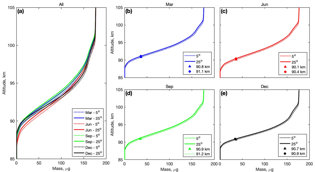
Figure 8. Example vertical mass profiles from CABMOD for a meteoric particle with a fixed initial mass ( 178 \mu\text{g} ) and velocity ( 31 \text{ km s}^{-1} ) at a latitude of 60^\circ \text{ S} . Panel (a) presents mass profiles (units: \mu\text{g} ) as a function of altitude (km) for four different months (Mar, Jun, Sep, and Dec), with meteoric particle entry of either 5^\circ or 25^\circ (entry angles relevant to the Southern Andes stations seen in Figure 5). Panels (b)–(e) depict the vertical mass profiles for each of the 4 months. The altitude at which 80% of the initial mass is lost is indicated by the filled triangle or filled circle for entry angles of 5^\circ and 25^\circ , respectively.
